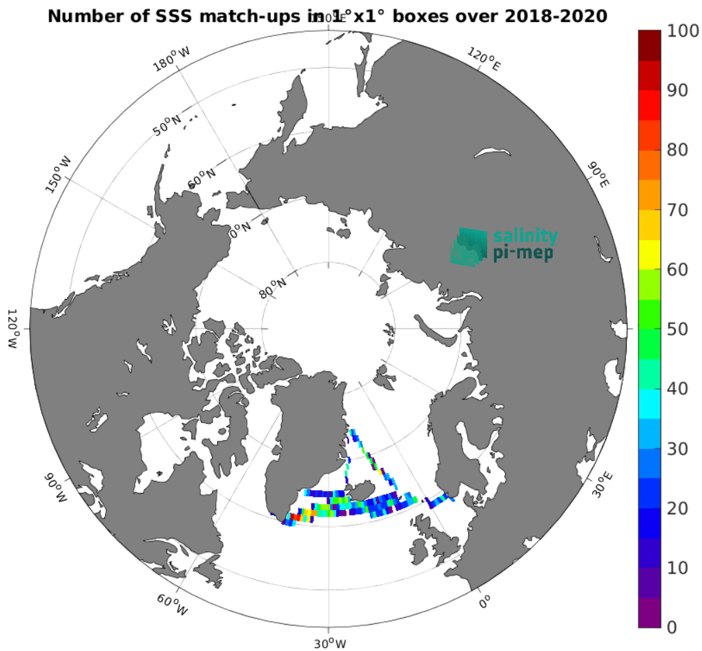
Figure 5: Number of SSS match-ups between TSG (Lauge-Koch) SSS and the CCI SSS L4 POLAR NH Merged-OI v4.41 - 7-day running (ESA) SSS product for the Global Ocean Pi-MEP region over 1^{\circ} \times 1^{\circ} boxes and for the full satellite product period.
