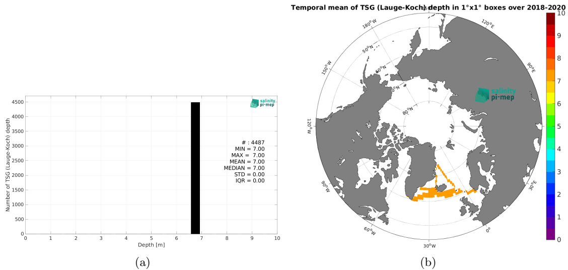
Figure 4: Histograms of the depth of the upper level SSS measurements from TSG (Lauge-Koch) in the Match-up DataBase for the Global Ocean Pi-MEP region (a) and temporal mean spatial distribution of pressure of the in situ SSS data over 1^\circ \times 1^\circ boxes and for the full satellite product period (b).
