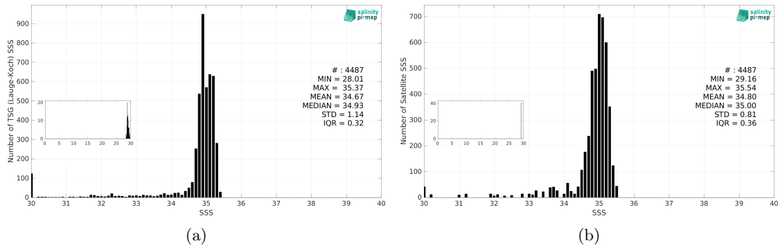
Figure 3: Histograms of SSS from TSG (Lauge-Koch) (a) and CCI SSS L4 POLAR NH Merged-OI v4.41 - 7-day running (ESA) (b) considering all match-up pairs per bins of 0.1 over the Global Ocean Pi-MEP region and for the full satellite product period.
