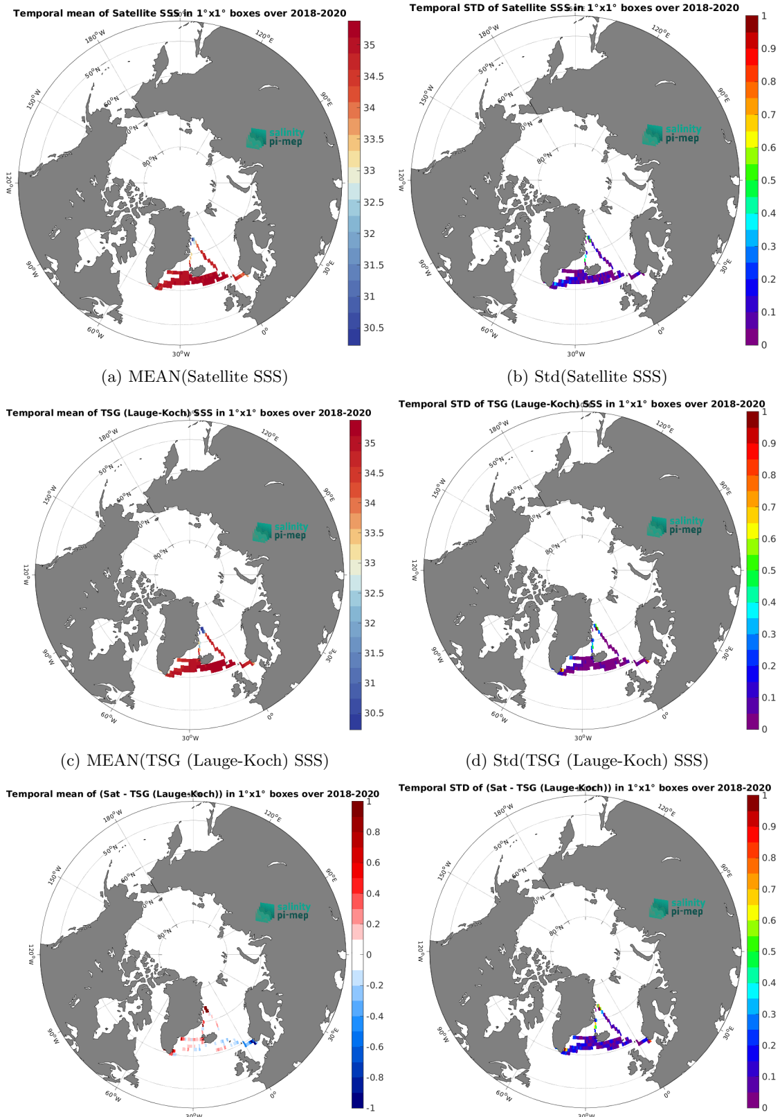
Figure 7: Temporal mean (left) and Std (right) of SSS from CCI SSS L4 POLAR NH Merged-OI v4.41 - 7-day running (ESA) (top), TSG (Lauge-Koch) (middle), and of \Delta SSS (Satellite - TSG (Lauge-Koch)). Only match-up pairs are used to generate these maps.
