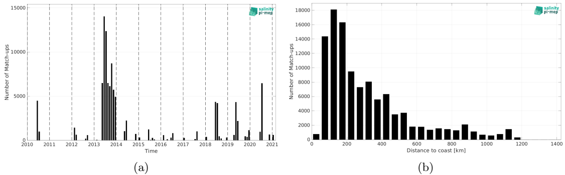
Figure 2: Number of match-ups between TSG (GOSUD-Sailing-ship) and CCI SSS L4 POLAR NH Merged-OI v4.41 - 7-day running (ESA) SSS as a function of time (a) and as function of the distance to coast (b) over the Global Ocean Pi-MEP region and for the full satellite product period.
