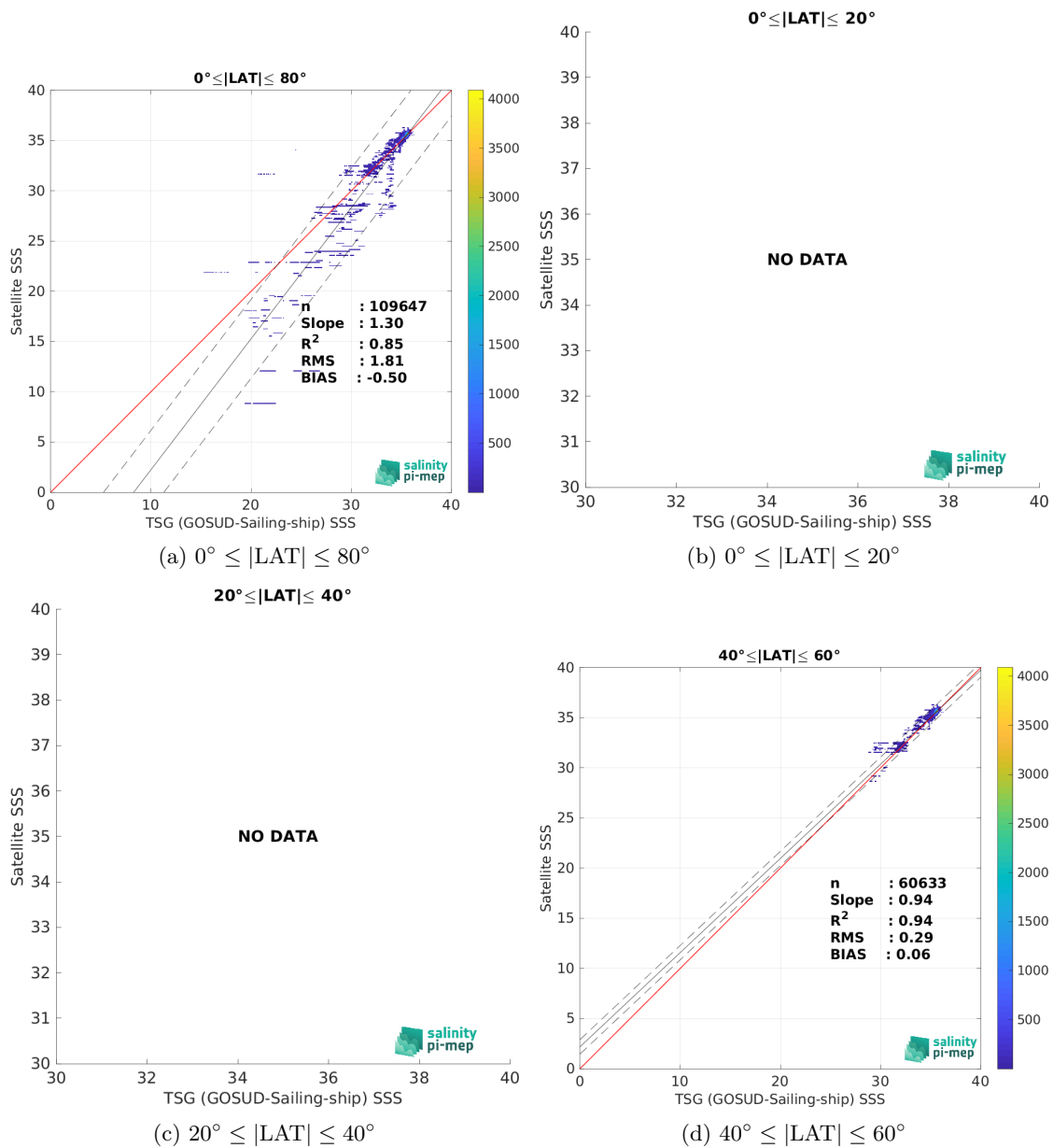
Figure 10: Contour maps of the concentration of CCI SSS L4 POLAR NH Merged-OI v4.41 - 7-day running (ESA) SSS (y-axis) versus TSG (GOSUD-Sailing-ship) SSS (x-axis) at match-up pairs for different latitude bands. For each plot, the red line shows x=y . The black thin and dashed lines indicate a linear fit through the data cloud and the \pm 95\% confidence levels, respectively. The number match-up pairs n , the slope and R^2 coefficient of the linear fit, the root mean square (RMS) and the mean bias between satellite and in situ data are indicated for each latitude band in each plots.
