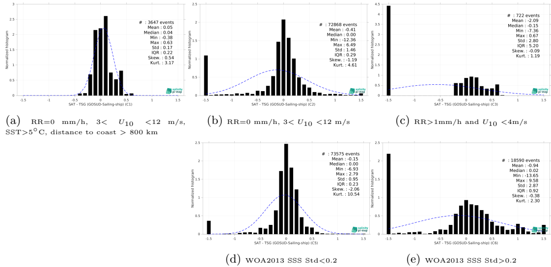
Figure 15: Normalized histogram of \Delta SSS (CCI SSS L4 POLAR NH Merged-OI v4.41 - 7-day running (ESA) - TSG (GOSUD-Sailing-ship)) for 5 different subdatasets corresponding to: RR=0 mm/h, 3 < U_{10} < 12 m/s, SST > 5°C, distance to coast > 800 km (a), RR=0 mm/h, 3 < U_{10} < 12 m/s (b), RR > 1mm/h and U_{10} < 4 m/s (c), WOA2013 SSS Std < 0.2 (d), WOA2013 SSS Std > 0.2 (e).
