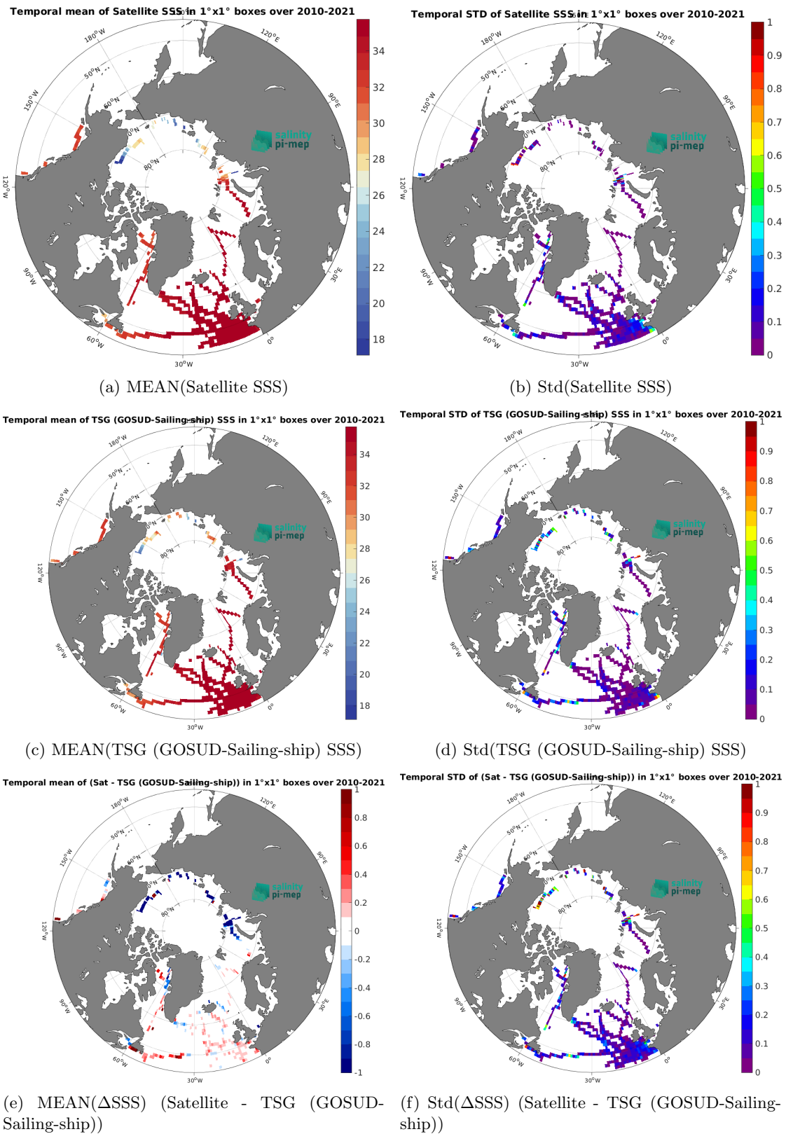
Figure 7: Temporal mean (left) and Std (right) of SSS from CCI SSS L4 POLAR NH Merged-OI v4.41 - 7-day running (ESA) (top), TSG (GOSUD-Sailing-ship) (middle), and of \Delta SSS (Satellite - TSG (GOSUD-Sailing-ship)). Only match-up pairs are used to generate these maps.
