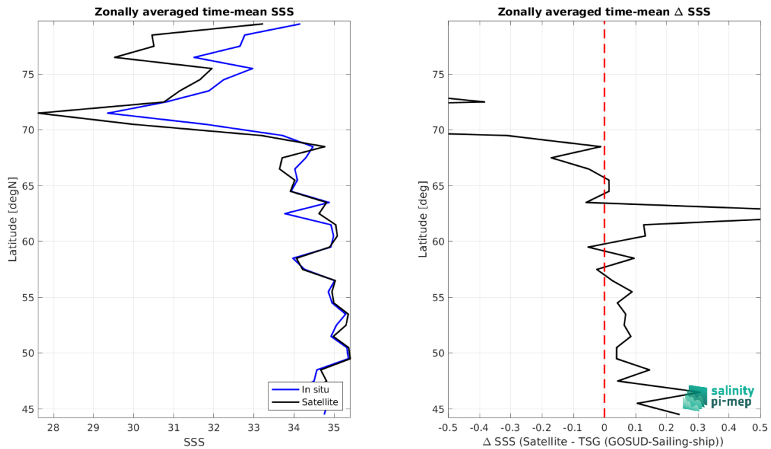
Figure 9: Left panel: Zonal mean SSS from CCI SSS L4 POLAR NH Merged-OI v4.41 - 7-day running (ESA) satellite product (black) and from TSG (GOSUD-Sailing-ship) (blue). Right panel: Zonal mean of \Delta SSS (Satellite - TSG (GOSUD-Sailing-ship)) for all the collected Pi-MEP match-up pairs estimated over the full satellite product period.
