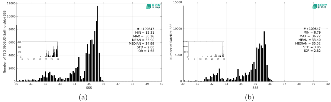
Figure 3: Histograms of SSS from TSG (GOSUD-Sailing-ship) (a) and CCI SSS L4 POLAR NH Merged-OI v4.41 - 7-day running (ESA) (b) considering all match-up pairs per bins of 0.1 over the Global Ocean Pi-MEP region and for the full satellite product period.
