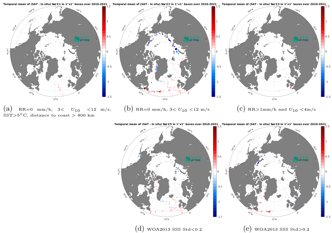
Figure 14: Temporal mean gridded over spatial boxes of size 1^\circ \times 1^\circ of \Delta SSS (CCI SSS L4 POLAR NH Merged-OI v4.41 - 7-day running (ESA) - TSG (GOSUD-Sailing-ship)) for 5 different subdatasets corresponding to:RR=0 mm/h, 3 < U_{10} < 12 m/s, SST >5^\circ C, distance to coast > 800 km (a), RR=0 mm/h, 3 < U_{10} < 12 m/s (b), RR >1 mm/h and U_{10} < 4 m/s (c), WOA2013 SSS Std <0.2 (d), WOA2013 SSS Std >0.2 (e).
