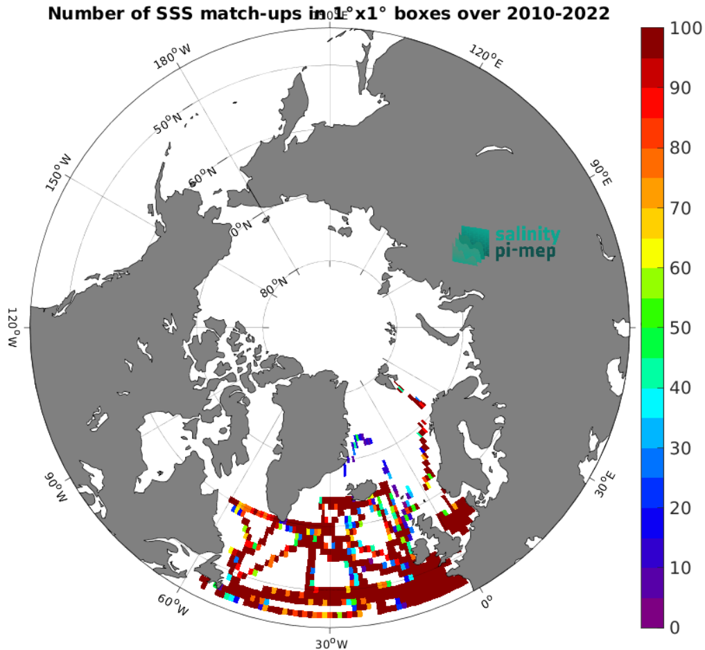
Figure 5: Number of SSS match-ups between TSG (GOSUD-Research-vessel) SSS and the CCI SSS L4 POLAR NH Merged-OI v4.41 - 7-day running (ESA) SSS product for the Global Ocean Pi-MEP region over 1^\circ \times 1^\circ boxes and for the full satellite product period.
