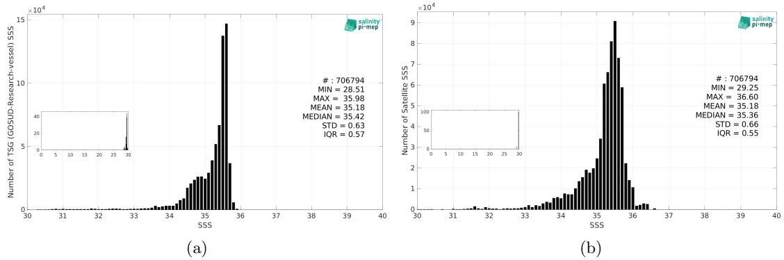
Figure 3: Histograms of SSS from TSG (GOSUD-Research-vessel) (a) and CCI SSS L4 POLAR NH Merged-OI v4.41 - 7-day running (ESA) (b) considering all match-up pairs per bins of 0.1 over the Global Ocean Pi-MEP region and for the full satellite product period.
