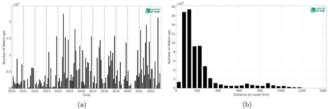
Figure 2: Number of match-ups between TSG (GOSUD-Research-vessel) and CCI SSS L4 POLAR NH Merged-OI v4.41 - 7-day running (ESA) SSS as a function of time (a) and as function of the distance to coast (b) over the Global Ocean Pi-MEP region and for the full satellite product period.
