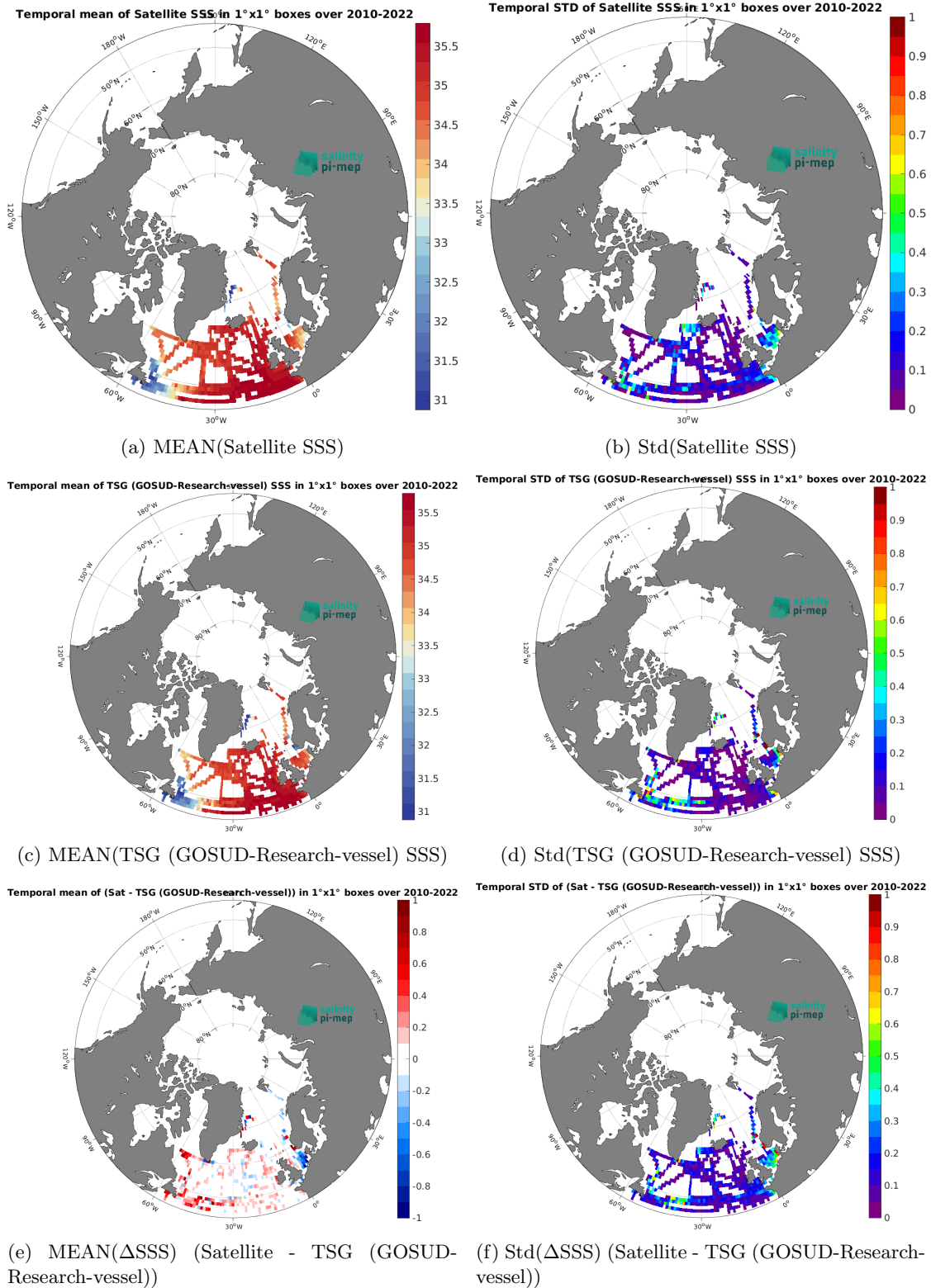
Figure 7: Temporal mean (left) and Std (right) of SSS from CCI SSS L4 POLAR NH Merged-OI v4.41 - 7-day running (ESA) (top), TSG (GOSUD-Research-vessel) (middle), and of \Delta SSS (Satellite - TSG (GOSUD-Research-vessel)). Only match-up pairs are used to generate these maps.
