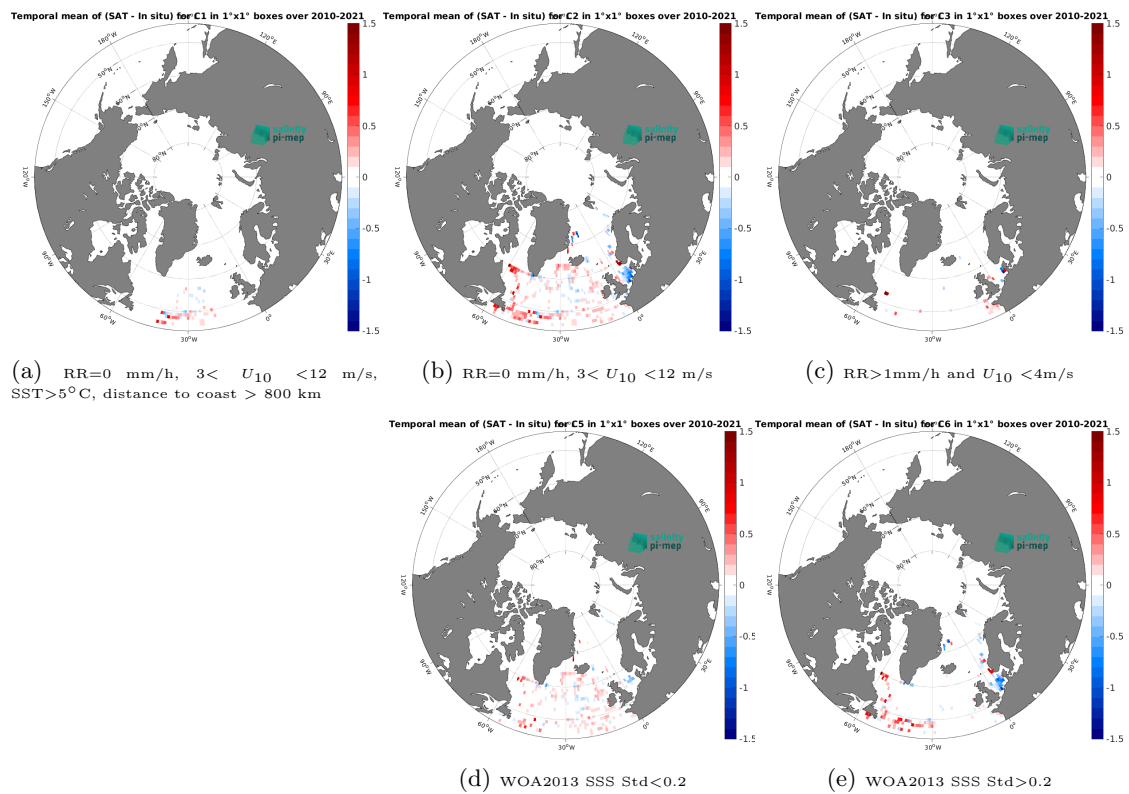
Figure 14: Temporal mean gridded over spatial boxes of size 1^\circ \times 1^\circ of \Delta\text{SSS} (CCI SSS L4 POLAR NH Merged-OI v4.41 - 7-day running (ESA) - TSG (GOSUD-Research-vessel)) for 5 different subdatasets corresponding to:RR=0 mm/h, 3 < U_{10} < 12 m/s, SST >5^\circ\text{C} , distance to coast > 800 km (a), RR=0 mm/h, 3 < U_{10} < 12 m/s (b), RR >1 mm/h and U_{10} < 4 m/s (c), WOA2013 SSS Std <0.2 (d), WOA2013 SSS Std >0.2 (e).
