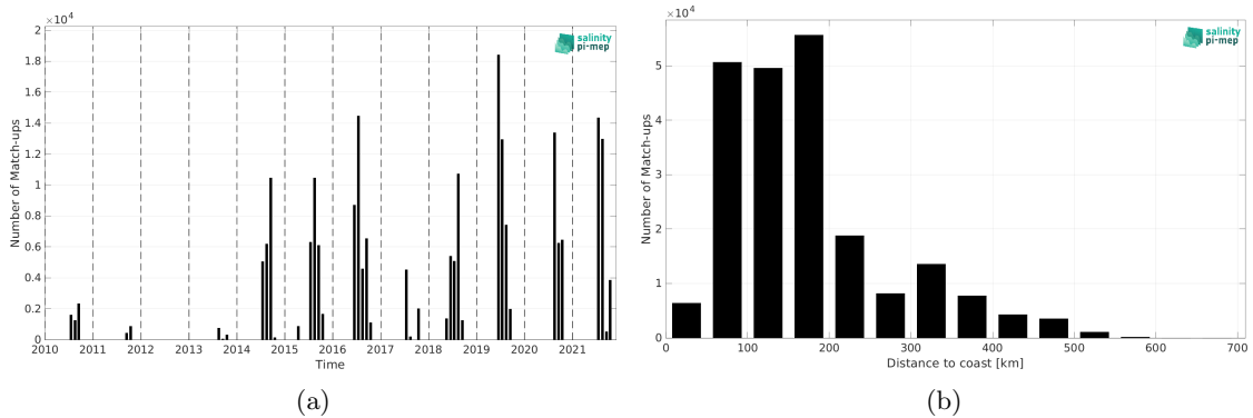
Figure 2: Number of match-ups between TSG (Amundsen) and CCI SSS L4 POLAR NH Merged-OI v4.41 - 7-day running (ESA) SSS as a function of time (a) and as function of the distance to coast (b) over the Global Ocean Pi-MEP region and for the full satellite product period.
