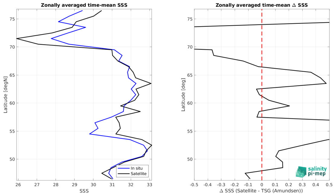
Figure 9: Left panel: Zonal mean SSS from CCI SSS L4 POLAR NH Merged-OI v4.41 - 7-day running (ESA) satellite product (black) and from TSG (Amundsen) (blue). Right panel: Zonal mean of \Delta SSS (Satellite - TSG (Amundsen)) for all the collected Pi-MEP match-up pairs estimated over the full satellite product period.
