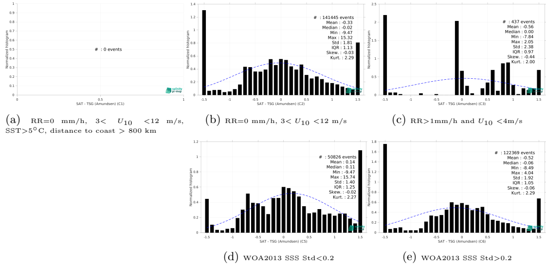
Figure 15: Normalized histogram of \Delta SSS (CCI SSS L4 POLAR NH Merged-OI v4.41 - 7-day running (ESA) - TSG (Amundsen)) for 5 different subdatasets corresponding to: RR=0 mm/h, 3 < U_{10} < 12 m/s, SST > 5°C, distance to coast > 800 km (a), RR=0 mm/h, 3 < U_{10} < 12 m/s (b), RR > 1mm/h and U_{10} < 4 m/s (c), WOA2013 SSS Std < 0.2 (d), WOA2013 SSS Std > 0.2 (e).
