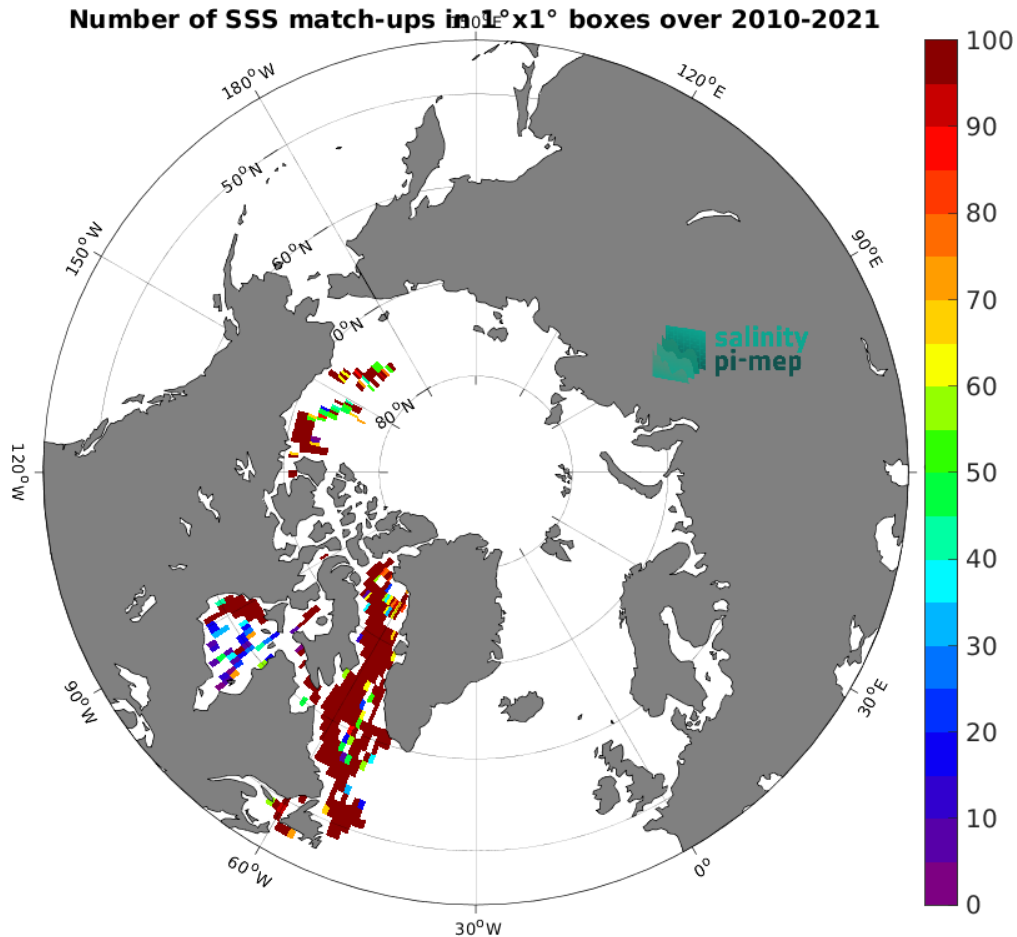
Figure 5: Number of SSS match-ups between TSG (Amundsen) SSS and the CCI SSS L4 POLAR NH Merged-OI v4.41 - 7-day running (ESA) SSS product for the Global Ocean Pi-MEP region over 1^\circ \times 1^\circ boxes and for the full satellite product period.
