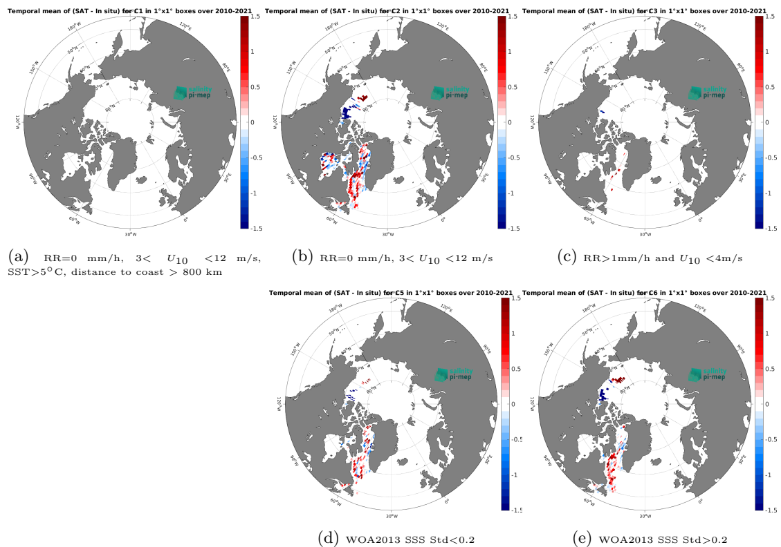
Figure 14: Temporal mean gridded over spatial boxes of size 1^\circ \times 1^\circ of \Delta SSS (CCI SSS L4 POLAR NH Merged-OI v4.41 - 7-day running (ESA) - TSG (Amundsen)) for 5 different subdatasets corresponding to:RR=0 mm/h, 3 < U_{10} < 12 m/s, SST >5^\circ C, distance to coast > 800 km (a), RR=0 mm/h, 3 < U_{10} < 12 m/s (b), RR >1 mm/h and U_{10} < 4 m/s (c), WOA2013 SSS Std <0.2 (d), WOA2013 SSS Std >0.2 (e).
