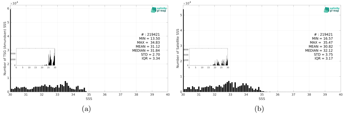
Figure 3: Histograms of SSS from TSG (Amundsen) (a) and CCI SSS L4 POLAR NH Merged-OI v4.41 - 7-day running (ESA) (b) considering all match-up pairs per bins of 0.1 over the Global Ocean Pi-MEP region and for the full satellite product period.
