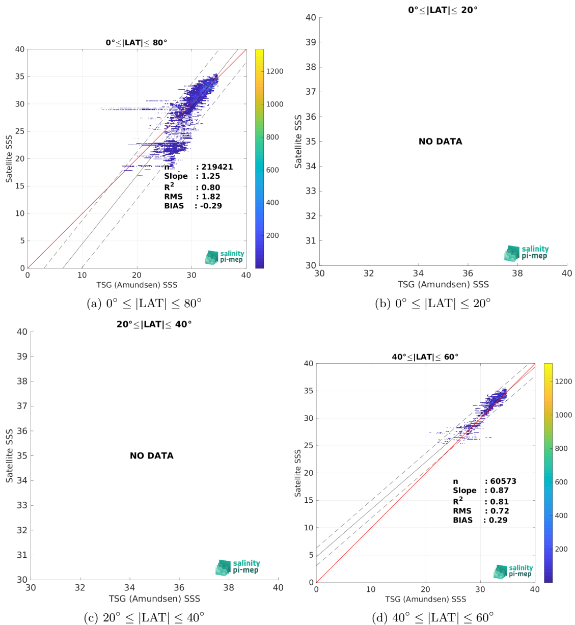
Figure 10: Contour maps of the concentration of CCI SSS L4 POLAR NH Merged-OI v4.41 - 7-day running (ESA) SSS (y-axis) versus TSG (Amundsen) SSS (x-axis) at match-up pairs for different latitude bands. For each plot, the red line shows x=y . The black thin and dashed lines indicate a linear fit through the data cloud and the \pm 95\% confidence levels, respectively. The number match-up pairs n , the slope and R^2 coefficient of the linear fit, the root mean square (RMS) and the mean bias between satellite and in situ data are indicated for each latitude band in each plots.
