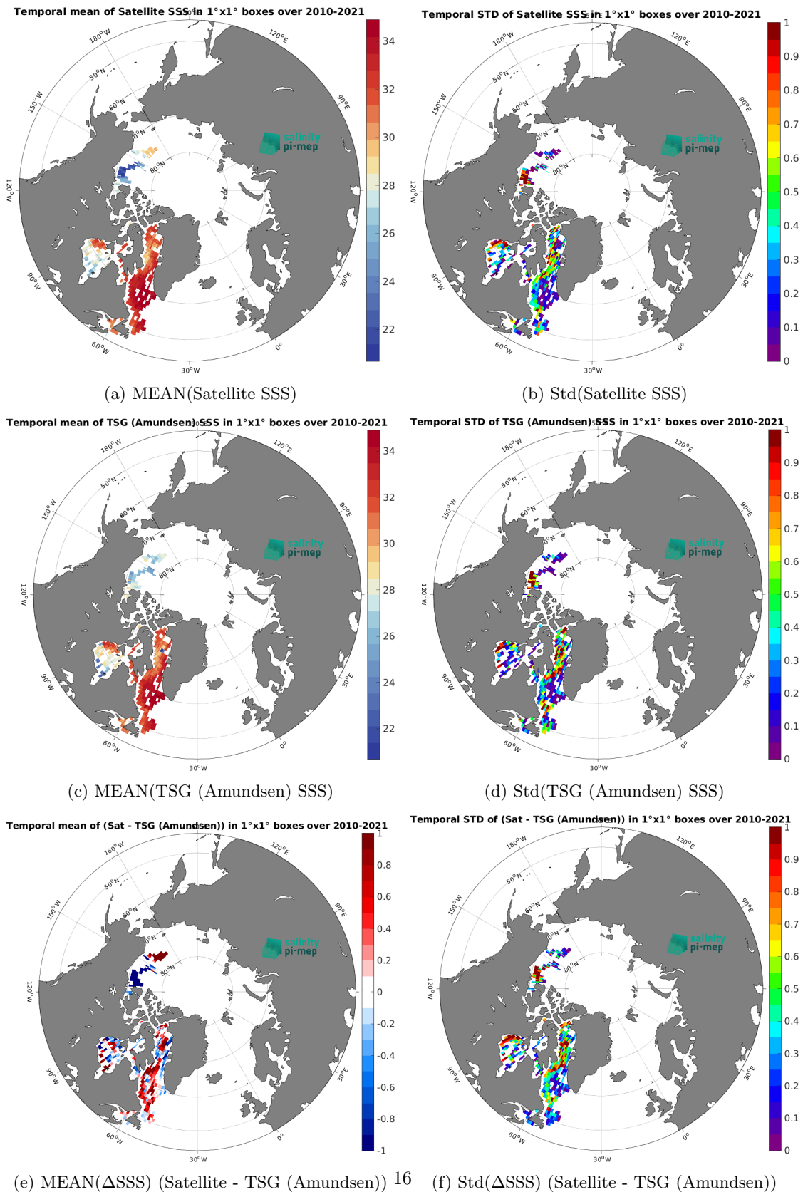
Figure 7: Temporal mean (left) and Std (right) of SSS from CCI SSS L4 POLAR NH Merged-OI v4.41 - 7-day running (ESA) (top), TSG (Amundsen) (middle), and of \Delta SSS (Satellite - TSG (Amundsen)). Only match-up pairs are used to generate these maps.
