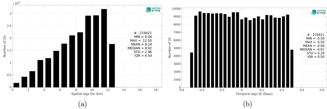
Figure 6: Histograms of the spatial (a) and temporal (b) lags between the location/time of the TSG (Amundsen) measurement and the date of the corresponding CCI SSS L4 POLAR NH Merged-OI v4.41 - 7-day running (ESA) SSS pixel.
