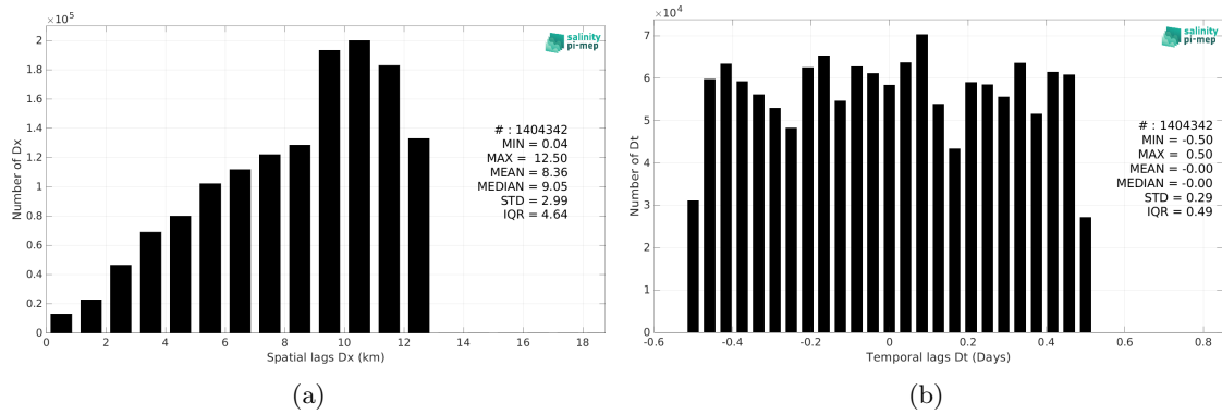
Figure 6: Histograms of the spatial (a) and temporal (b) lags between the location/time of the SASSIE measurement and the date of the corresponding CCI SSS L4 POLAR NH Merged-OI v4.41 - 7-day running (ESA) SSS pixel.
