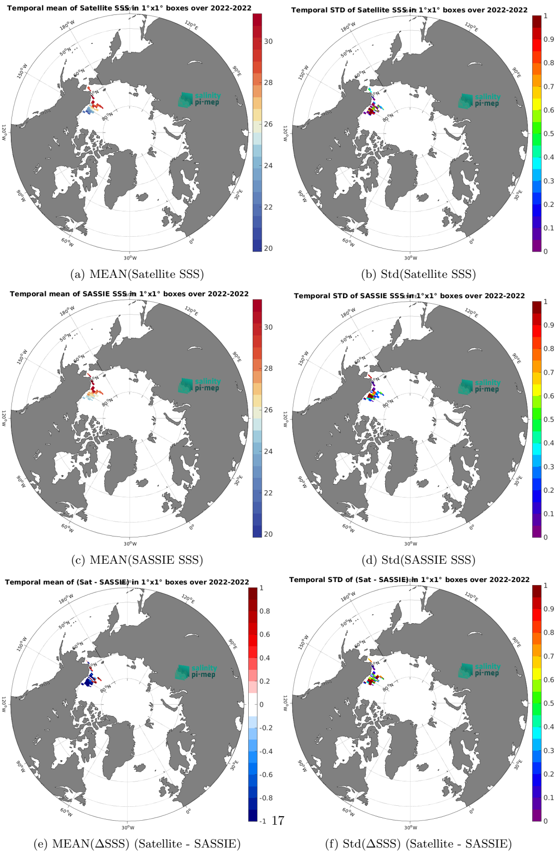
Figure 7: Temporal mean (left) and Std (right) of SSS from CCI SSS L4 POLAR NH Merged-OI v4.41 - 7-day running (ESA) (top), SASSIE (middle), and of \Delta SSS (Satellite - SASSIE). Only match-up pairs are used to generate these maps.
