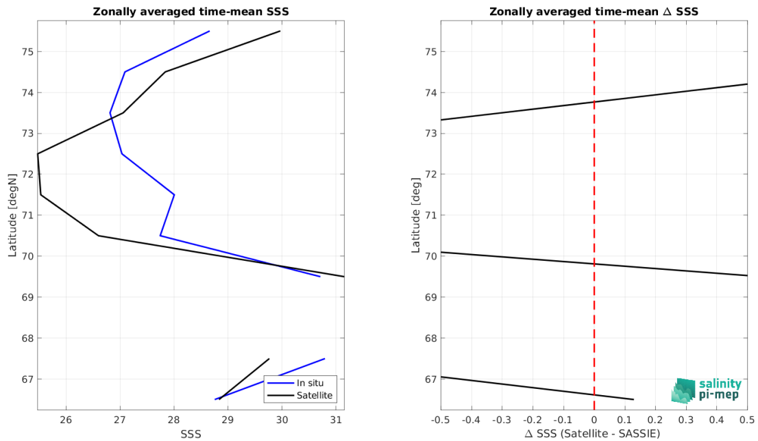
Figure 9: Left panel: Zonal mean SSS from CCI SSS L4 POLAR NH Merged-OI v4.41 - 7-day running (ESA) satellite product (black) and from SASSIE (blue). Right panel: Zonal mean of \Delta SSS (Satellite - SASSIE) for all the collected Pi-MEP match-up pairs estimated over the full satellite product period.
