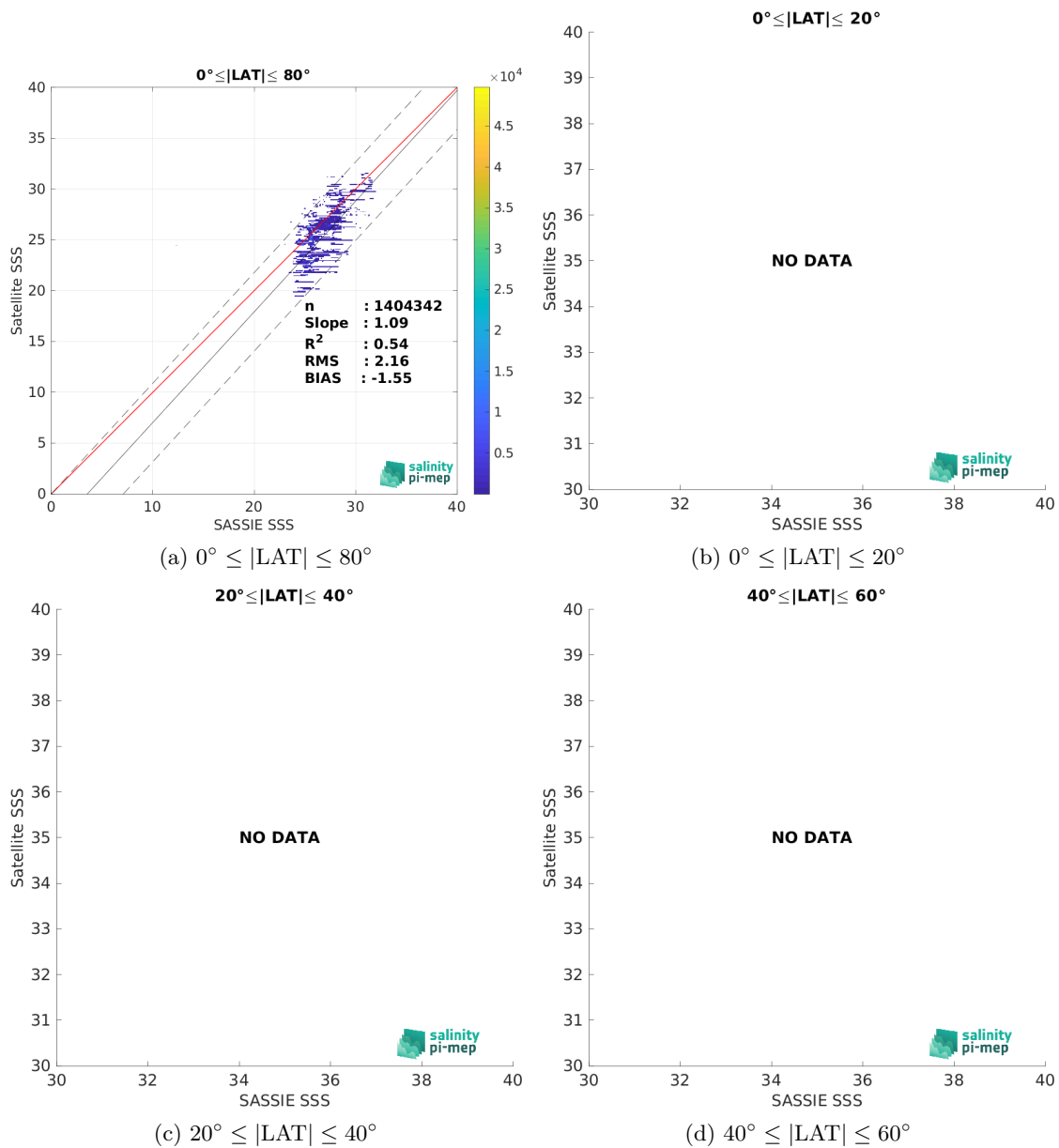
Figure 10: Contour maps of the concentration of CCI SSS L4 POLAR NH Merged-OI v4.41 - 7-day running (ESA) SSS (y-axis) versus SASSIE SSS (x-axis) at match-up pairs for different latitude bands. For each plot, the red line shows x=y . The black thin and dashed lines indicate a linear fit through the data cloud and the \pm 95\% confidence levels, respectively. The number match-up pairs n , the slope and R^2 coefficient of the linear fit, the root mean square (RMS) and the mean bias between satellite and in situ data are indicated for each latitude band in each plots.
