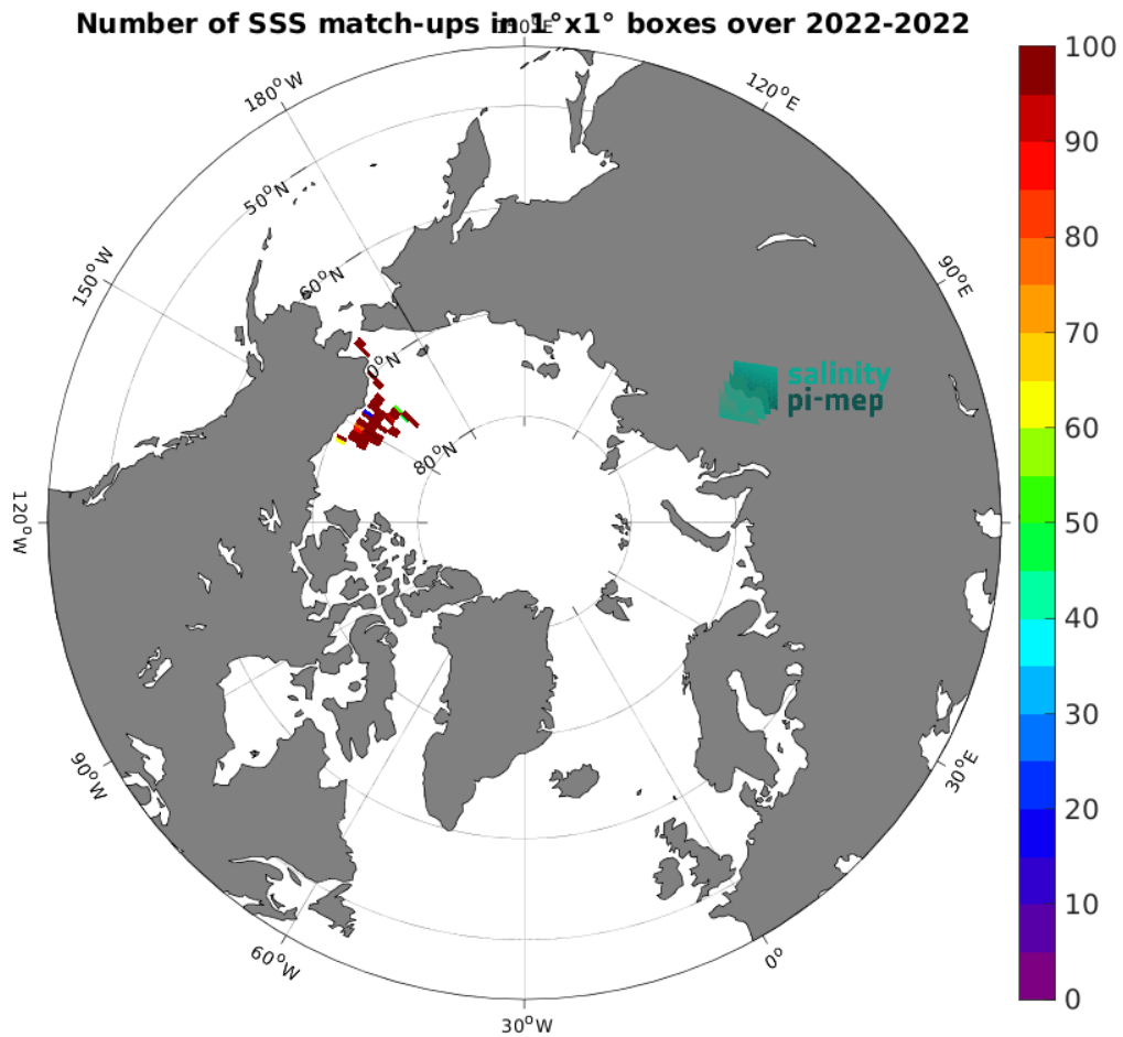
Figure 5: Number of SSS match-ups between SASSIE SSS and the CCI SSS L4 POLAR NH Merged-OI v4.41 - 7-day running (ESA) SSS product for the Global Ocean Pi-MEP region over 1^{\circ} \times 1^{\circ} boxes and for the full satellite product period.
