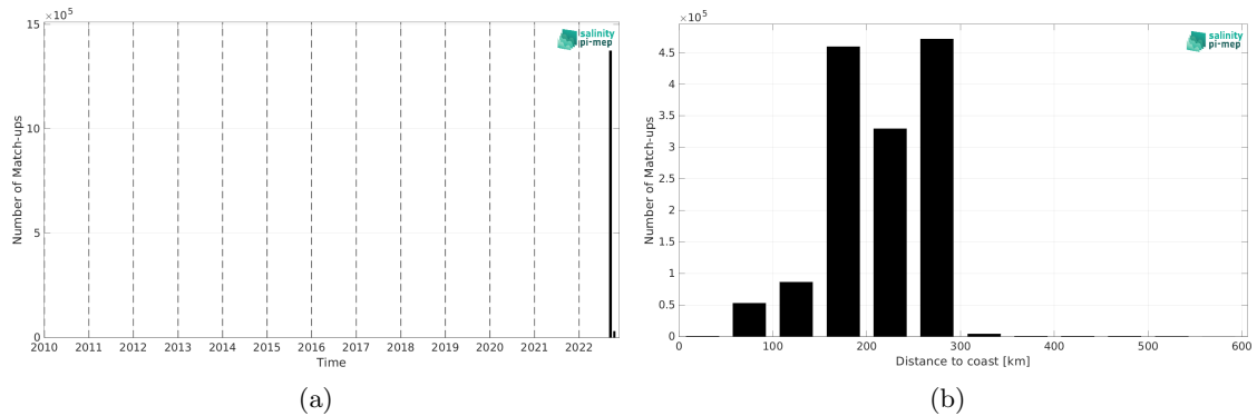
Figure 2: Number of match-ups between SASSIE and CCI SSS L4 POLAR NH Merged-OI v4.41 - 7-day running (ESA) SSS as a function of time (a) and as function of the distance to coast (b) over the Global Ocean Pi-MEP region and for the full satellite product period.
