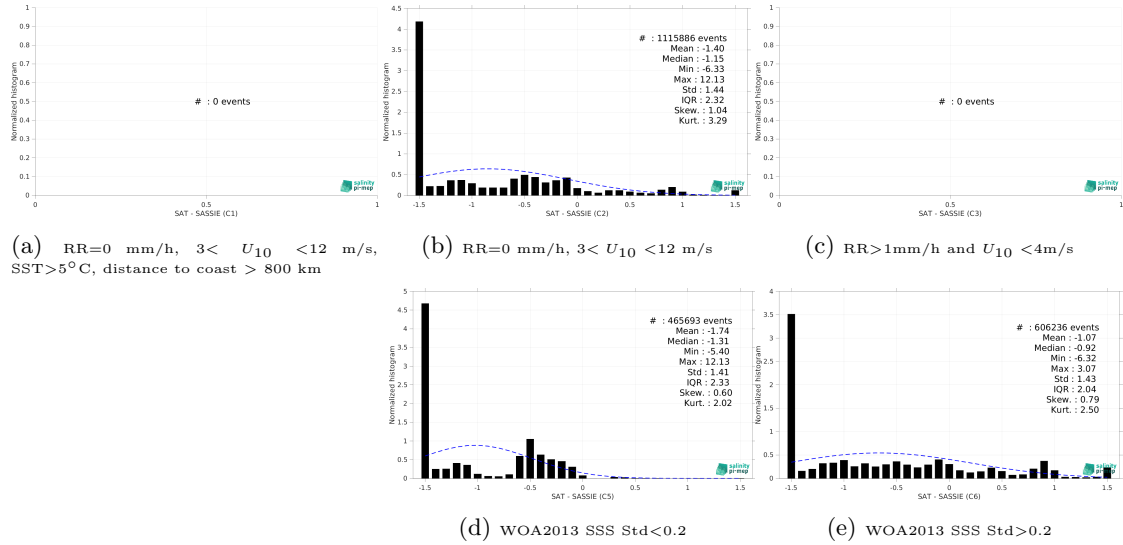
Figure 15: Normalized histogram of \Delta SSS (CCI SSS L4 POLAR NH Merged-OI v4.41 - 7-day running (ESA) - SASSIE) for 5 different subdatasets corresponding to: RR=0 mm/h, 3 < U_{10} < 12 m/s, SST > 5°C, distance to coast > 800 km (a), RR=0 mm/h, 3 < U_{10} < 12 m/s (b), RR > 1mm/h and U_{10} < 4 m/s (c), WOA2013 SSS Std < 0.2 (d), WOA2013 SSS Std > 0.2 (e).
