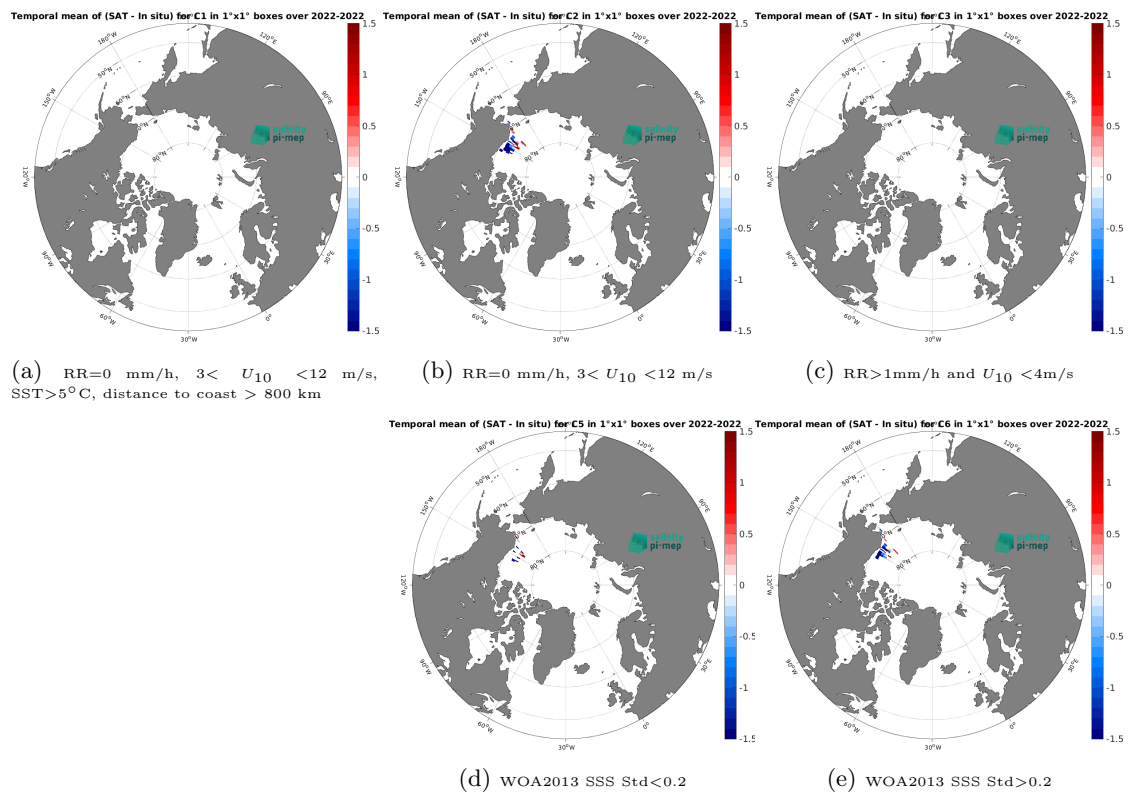
Figure 14: Temporal mean gridded over spatial boxes of size 1^\circ \times 1^\circ of \Delta SSS (CCI SSS L4 POLAR NH Merged-OI v4.41 - 7-day running (ESA) - SASSIE) for 5 different subdatasets corresponding to:RR=0 mm/h, 3 < U_{10} < 12 m/s, SST >5^\circ C, distance to coast > 800 km (a), RR=0 mm/h, 3 < U_{10} < 12 m/s (b), RR >1 mm/h and U_{10} < 4 m/s (c), WOA2013 SSS Std <0.2 (d), WOA2013 SSS Std >0.2 (e).
