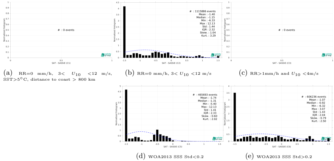
Figure 15: Normalized histogram of \Delta SSS (CCI SSS L4 POLAR NH Merged-OI v4.41 - 7-day running (ESA) - SASSIE) for 5 different subdatasets corresponding to: RR=0 mm/h, 3 < U_{10} < 12 m/s, SST > 5°C, distance to coast > 800 km (a), RR=0 mm/h, 3 < U_{10} < 12 m/s (b), RR > 1mm/h and U_{10} < 4 m/s (c), WOA2013 SSS Std < 0.2 (d), WOA2013 SSS Std > 0.2 (e).
