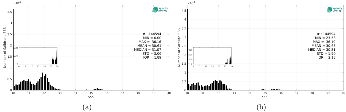
Figure 3: Histograms of SSS from Saildrone (a) and CCI SSS L4 POLAR NH Merged-OI v4.41 - 7-day running (ESA) (b) considering all match-up pairs per bins of 0.1 over the Global Ocean Pi-MEP region and for the full satellite product period.
