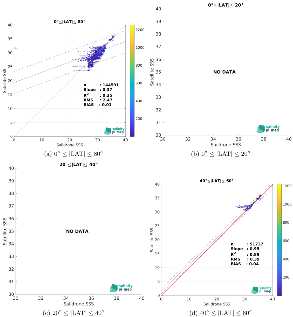
Figure 10: Contour maps of the concentration of CCI SSS L4 POLAR NH Merged-OI v4.41 - 7-day running (ESA) SSS (y-axis) versus Saildrone SSS (x-axis) at match-up pairs for different latitude bands. For each plot, the red line shows x=y . The black thin and dashed lines indicate a linear fit through the data cloud and the \pm 95\% confidence levels, respectively. The number match-up pairs n , the slope and R^2 coefficient of the linear fit, the root mean square (RMS) and the mean bias between satellite and in situ data are indicated for each latitude band in each plots.
