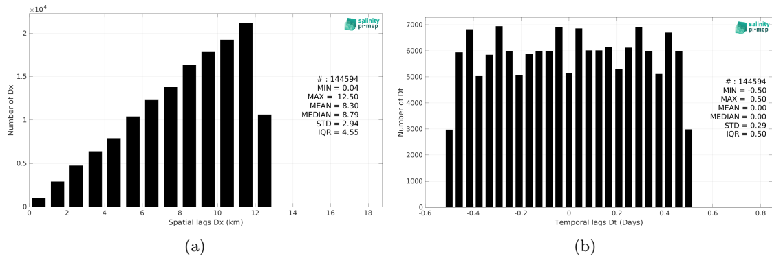
Figure 6: Histograms of the spatial (a) and temporal (b) lags between the location/time of the Saildrone measurement and the date of the corresponding CCI SSS L4 POLAR NH Merged-OI v4.41 - 7-day running (ESA) SSS pixel.
