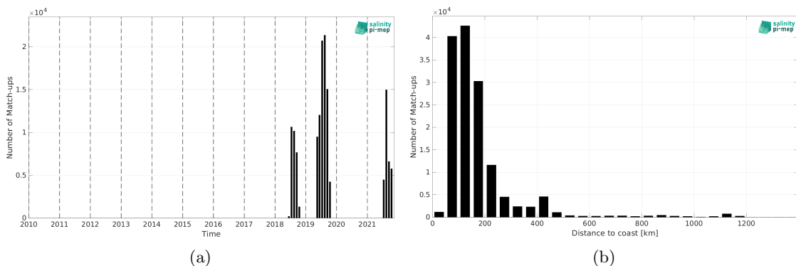
Figure 2: Number of match-ups between Saildrone and CCI SSS L4 POLAR NH Merged-OI v4.41 - 7-day running (ESA) SSS as a function of time (a) and as function of the distance to coast (b) over the Global Ocean Pi-MEP region and for the full satellite product period.
