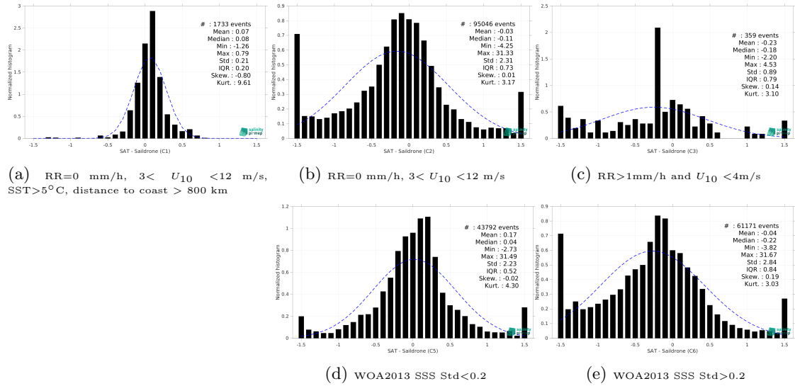
Figure 15: Normalized histogram of \Delta SSS (CCI SSS L4 POLAR NH Merged-OI v4.41 - 7-day running (ESA) - Saldrone) for 5 different subdatasets corresponding to: RR=0 mm/h, 3 < U_{10} < 12 m/s, SST>5°C, distance to coast > 800 km (a), RR=0 mm/h, 3 < U_{10} < 12 m/s (b), RR>1mm/h and U_{10} < 4 m/s (c), WOA2013 SSS Std<0.2 (d), WOA2013 SSS Std>0.2 (e).
