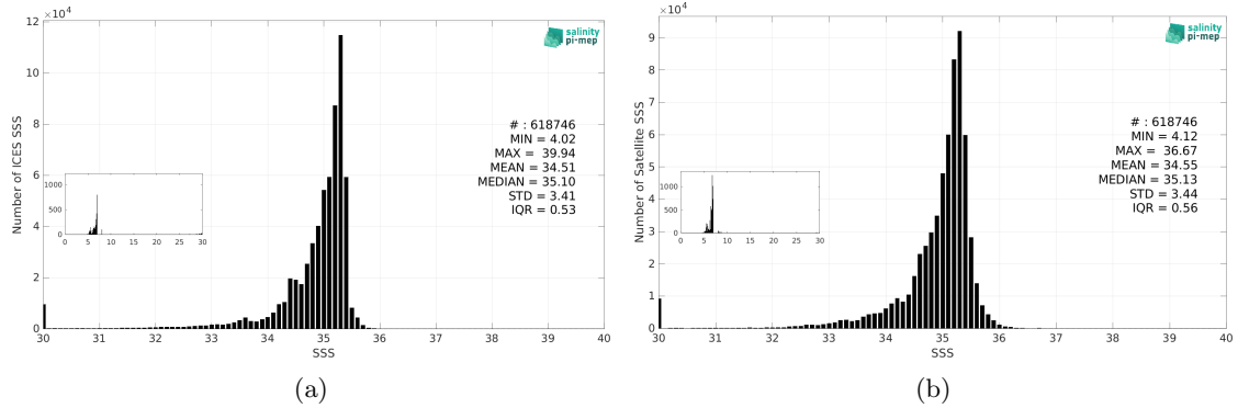
Figure 3: Histograms of SSS from ICES (a) and CCI SSS L4 POLAR NH Merged-OI v4.41 - 7-day running (ESA) (b) considering all match-up pairs per bins of 0.1 over the Global Ocean Pi-MEP region and for the full satellite product period.
