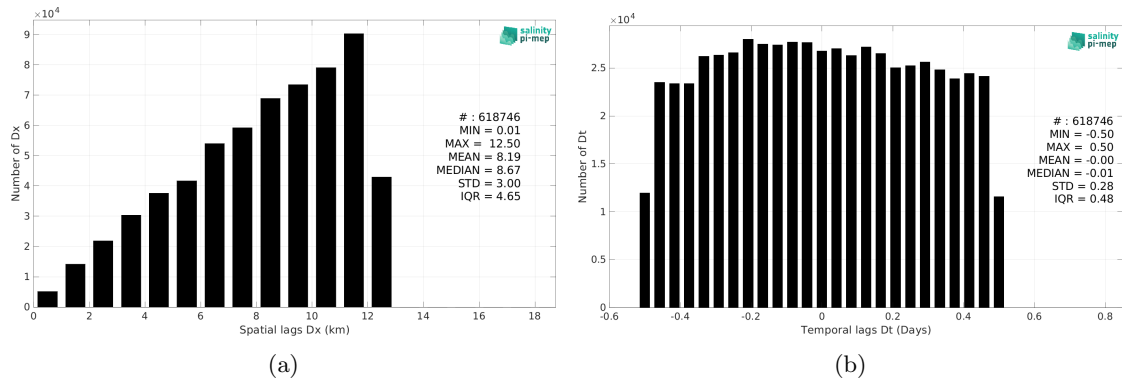
Figure 6: Histograms of the spatial (a) and temporal (b) lags between the location/time of the ICES measurement and the date of the corresponding CCI SSS L4 POLAR NH Merged-OI v4.41 - 7-day running (ESA) SSS pixel.
