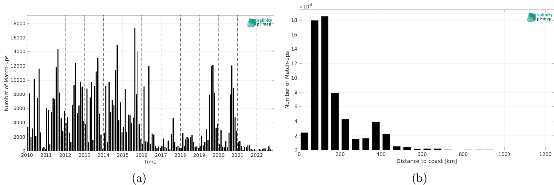
Figure 2: Number of match-ups between ICES and CCI SSS L4 POLAR NH Merged-OI v4.41 - 7-day running (ESA) SSS as a function of time (a) and as function of the distance to coast (b) over the Global Ocean Pi-MEP region and for the full satellite product period.
