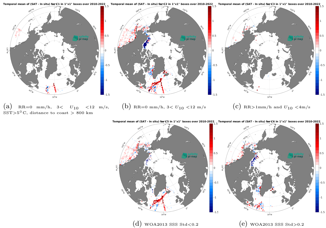
Figure 14: Temporal mean gridded over spatial boxes of size 1^\circ \times 1^\circ of \Delta\text{SSS} (CCI SSS L4 POLAR NH Merged-OI v4.41 - 30-day running (ESA) - TSG (SAMOS)) for 5 different subdatasets corresponding to:RR=0 mm/h, 3 < U_{10} < 12 m/s, SST>5°C, distance to coast > 800 km (a), RR=0 mm/h, 3 < U_{10} < 12 m/s (b), RR>1mm/h and U_{10} < 4 m/s (c), WOA2013 SSS Std<0.2 (d), WOA2013 SSS Std>0.2 (e).
