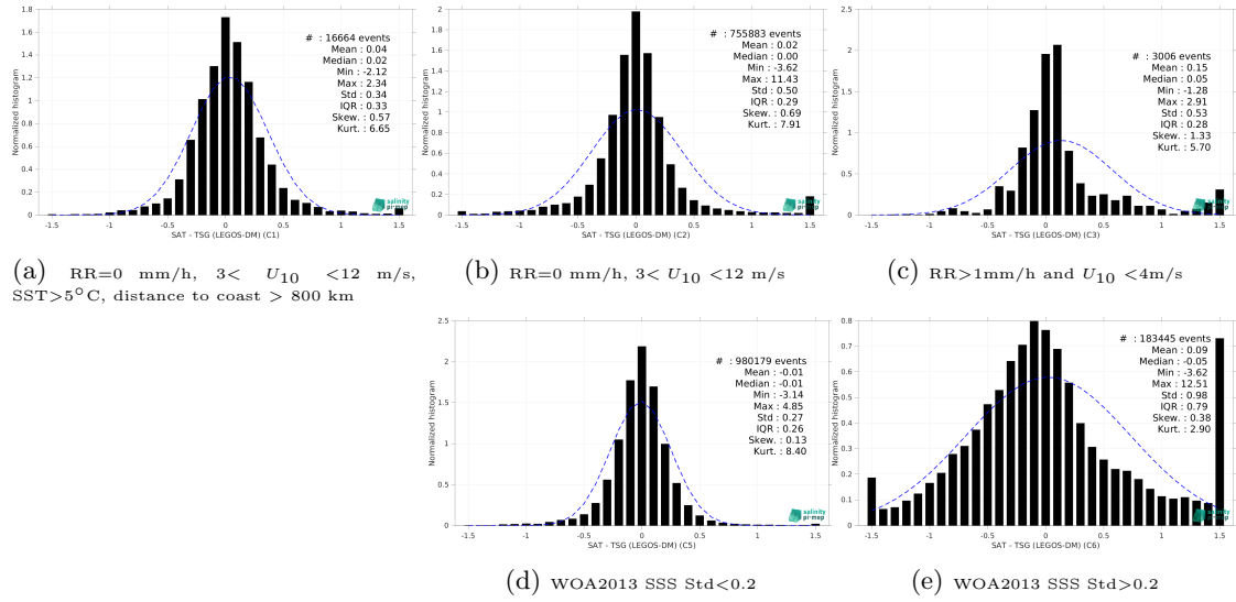
Figure 15: Normalized histogram of \Delta\text{SSS} (CCI SSS L4 POLAR NH Merged-OI v4.41 - 30-day running (ESA) - TSG (LEGOS-DM)) for 5 different subdatasets corresponding to: RR=0 mm/h, 3 < U_{10} < 12 m/s, SST>5°C, distance to coast > 800 km (a), RR=0 mm/h, 3 < U_{10} < 12 m/s (b), RR>1mm/h and U_{10} < 4 m/s (c), WOA2013 SSS Std<0.2 (d), WOA2013 SSS Std>0.2 (e).
