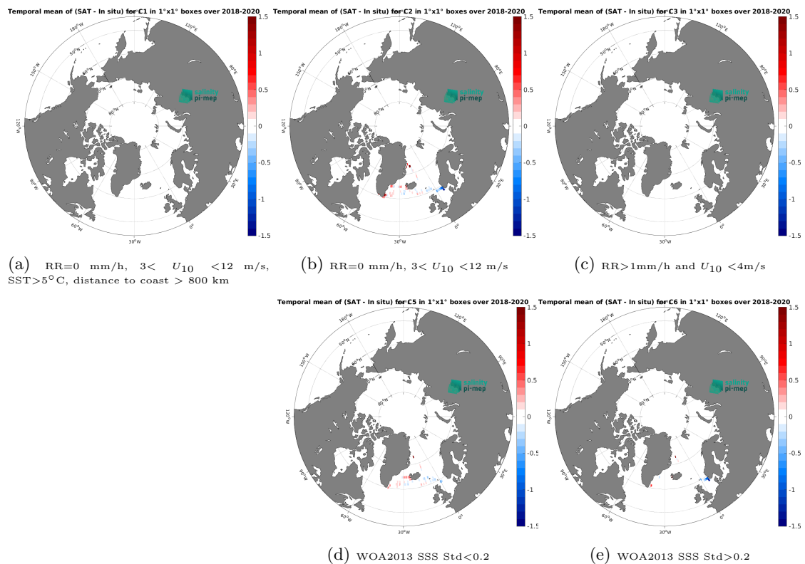
Figure 14: Temporal mean gridded over spatial boxes of size 1^\circ \times 1^\circ of \Delta SSS (CCI SSS L4 POLAR NH Merged-OI v4.41 - 30-day running (ESA) - TSG (Lauge-Koch)) for 5 different subdatasets corresponding to:RR=0 mm/h, 3 < U_{10} < 12 m/s, SST >5^\circ\text{C} , distance to coast > 800 km (a), RR=0 mm/h, 3 < U_{10} < 12 m/s (b), RR >1 mm/h and U_{10} < 4 m/s (c), WOA2013 SSS Std <0.2 (d), WOA2013 SSS Std >0.2 (e).
