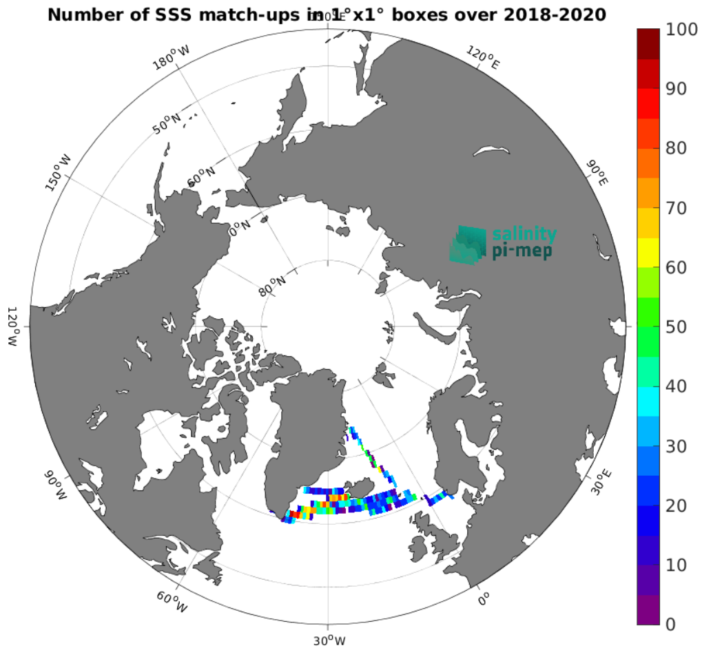
Figure 5: Number of SSS match-ups between TSG (Lauge-Koch) SSS and the CCI SSS L4 POLAR NH Merged-OI v4.41 - 30-day running (ESA) SSS product for the Global Ocean Pi-MEP region over 1^\circ \times 1^\circ boxes and for the full satellite product period.
