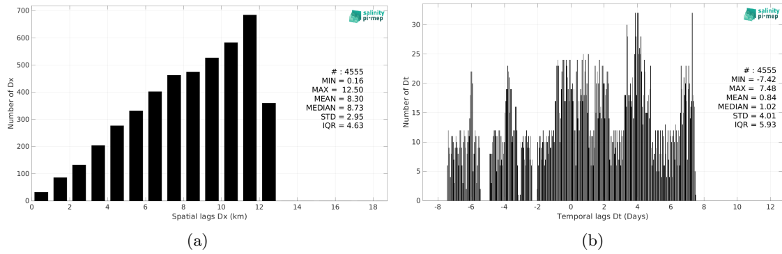
Figure 6: Histograms of the spatial (a) and temporal (b) lags between the location/time of the TSG (Lauge-Koch) measurement and the date of the corresponding CCI SSS L4 POLAR NH Merged-OI v4.41 - 30-day running (ESA) SSS pixel.
