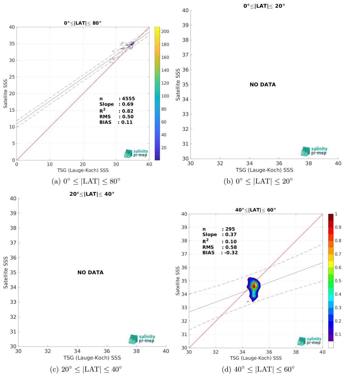
Figure 10: Contour maps of the concentration of CCI SSS L4 POLAR NH Merged-OI v4.41 - 30-day running (ESA) SSS (y-axis) versus TSG (Lauge-Koch) SSS (x-axis) at match-up pairs for different latitude bands. For each plot, the red line shows x=y . The black thin and dashed lines indicate a linear fit through the data cloud and the \pm 95\% confidence levels, respectively. The number match-up pairs n , the slope and R^2 coefficient of the linear fit, the root mean square (RMS) and the mean bias between satellite and in situ data are indicated for each latitude band in each plots.
