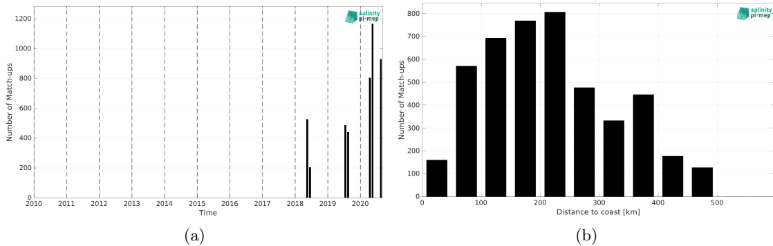
Figure 2: Number of match-ups between TSG (Lauge-Koch) and CCI SSS L4 POLAR NH Merged-OI v4.41 - 30-day running (ESA) SSS as a function of time (a) and as function of the distance to coast (b) over the Global Ocean Pi-MEP region and for the full satellite product period.
