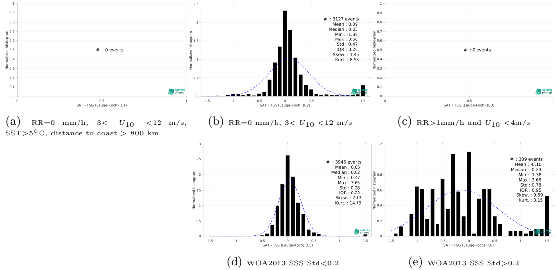
Figure 15: Normalized histogram of \Delta SSS (CCI SSS L4 POLAR NH Merged-OI v4.41 - 30-day running (ESA) - TSG (Laue-Koch)) for 5 different subdatasets corresponding to: RR=0 mm/h, 3 < U_{10} < 12 m/s, SST > 5°C, distance to coast > 800 km (a), RR=0 mm/h, 3 < U_{10} < 12 m/s (b), RR > 1mm/h and U_{10} < 4 m/s (c), WOA2013 SSS Std < 0.2 (d), WOA2013 SSS Std > 0.2 (e).
