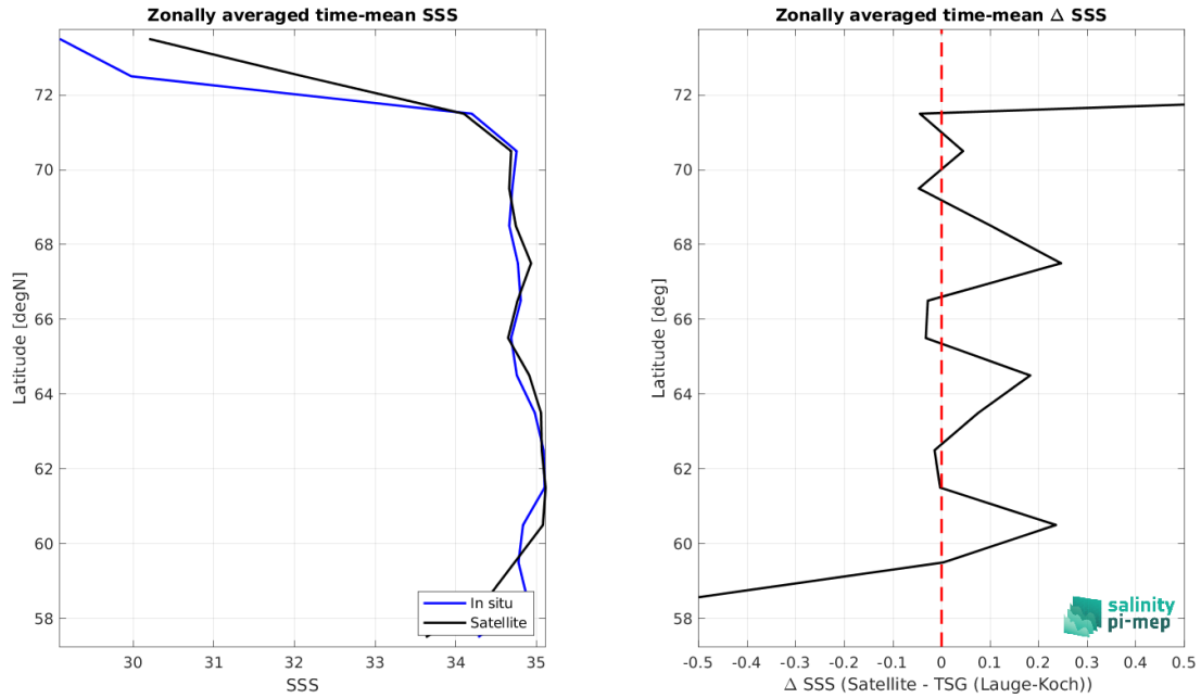
Figure 9: Left panel: Zonal mean SSS from CCI SSS L4 POLAR NH Merged-OI v4.41 - 30-day running (ESA) satellite product (black) and from TSG (Lauge-Koch) (blue). Right panel: Zonal mean of \Delta SSS (Satellite - TSG (Lauge-Koch)) for all the collected Pi-MEP match-up pairs estimated over the full satellite product period.
