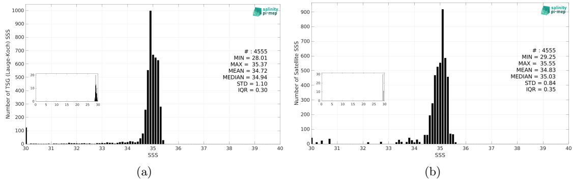
Figure 3: Histograms of SSS from TSG (Lauge-Koch) (a) and CCI SSS L4 POLAR NH Merged-OI v4.41 - 30-day running (ESA) (b) considering all match-up pairs per bins of 0.1 over the Global Ocean Pi-MEP region and for the full satellite product period.
