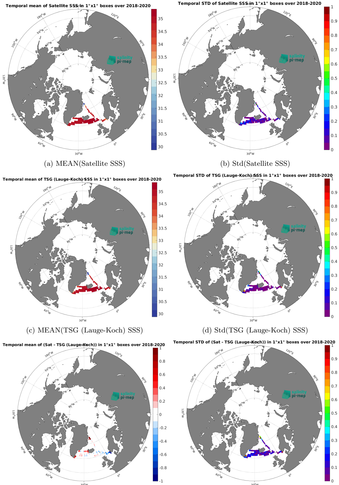
Figure 7: Temporal mean (left) and Std (right) of SSS from CCI SSS L4 POLAR NH Merged-OI v4.41 - 30-day running (ESA) (top), TSG (Lauge-Koch) (middle), and of \Delta SSS (Satellite - TSG (Lauge-Koch)). Only match-up pairs are used to generate these maps.
