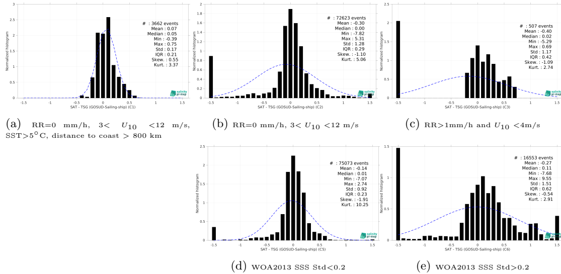
Figure 15: Normalized histogram of \Delta\text{SSS} (CCI SSS L4 POLAR NH Merged-OI v4.41 - 30-day running (ESA) - TSG (GOSUD-Sailing-ship)) for 5 different subdatasets corresponding to: RR=0 mm/h, 3 < U_{10} < 12 m/s, SST>5°C, distance to coast > 800 km (a), RR=0 mm/h, 3 < U_{10} < 12 m/s (b), RR>1mm/h and U_{10} < 4 m/s (c), WOA2013 SSS Std<0.2 (d), WOA2013 SSS Std>0.2 (e).
