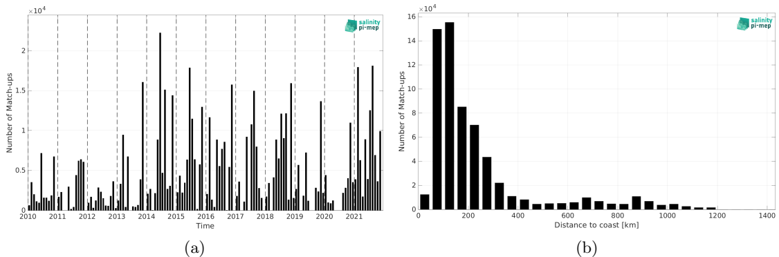
Figure 2: Number of match-ups between TSG (GOSUD-Research-vessel) and CCI SSS L4 POLAR NH Merged-OI v4.41 - 30-day running (ESA) SSS as a function of time (a) and as function of the distance to coast (b) over the Global Ocean Pi-MEP region and for the full satellite product period.
