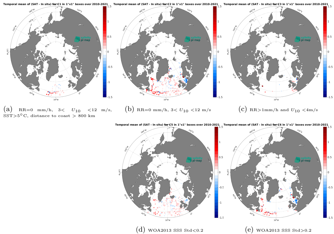
Figure 14: Temporal mean gridded over spatial boxes of size 1^\circ \times 1^\circ of \Delta SSS (CCI SSS L4 POLAR NH Merged-OI v4.41 - 30-day running (ESA) - TSG (GOSUD-Research-vessel)) for 5 different subdatasets corresponding to:RR=0 mm/h, 3 < U_{10} < 12 m/s, SST >5^\circ C, distance to coast > 800 km (a), RR=0 mm/h, 3 < U_{10} < 12 m/s (b), RR >1 mm/h and U_{10} < 4 m/s (c), WOA2013 SSS Std <0.2 (d), WOA2013 SSS Std >0.2 (e).
