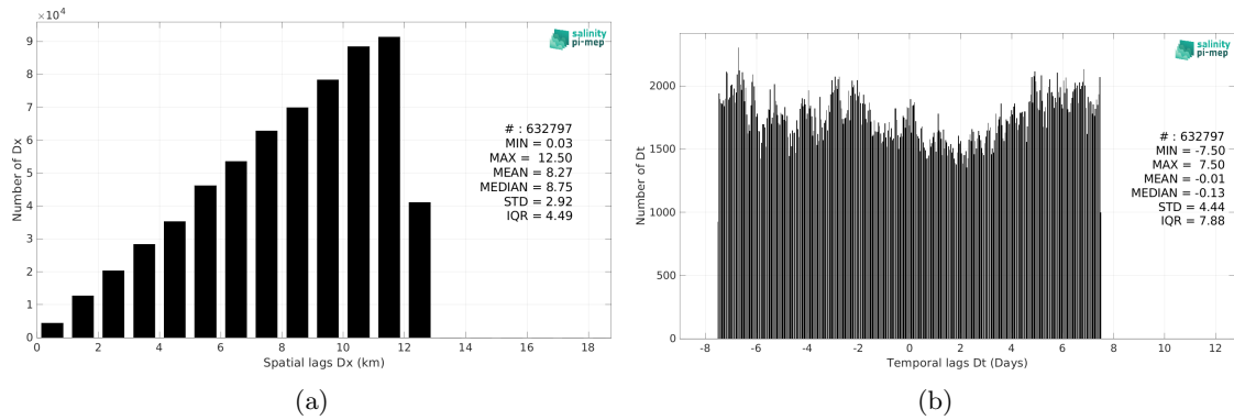
Figure 6: Histograms of the spatial (a) and temporal (b) lags between the location/time of the TSG (GOSUD-Research-vessel) measurement and the date of the corresponding CCI SSS L4 POLAR NH Merged-OI v4.41 - 30-day running (ESA) SSS pixel.
