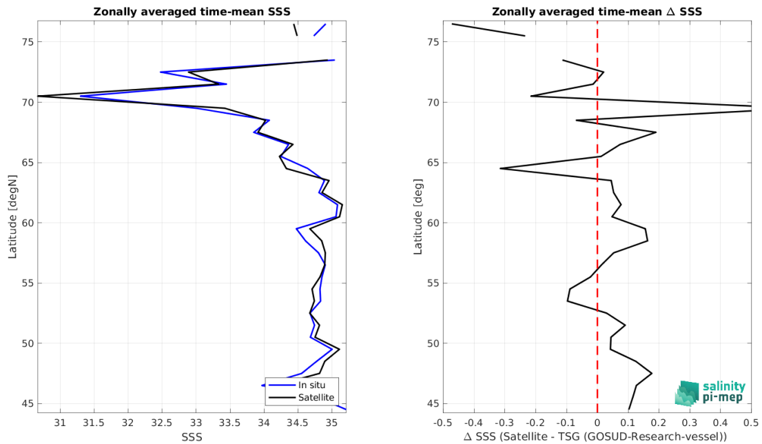
Figure 9: Left panel: Zonal mean SSS from CCI SSS L4 POLAR NH Merged-OI v4.41 - 30-day running (ESA) satellite product (black) and from TSG (GOSUD-Research-vessel) (blue). Right panel: Zonal mean of \Delta SSS (Satellite - TSG (GOSUD-Research-vessel)) for all the collected Pi-MEP match-up pairs estimated over the full satellite product period.
