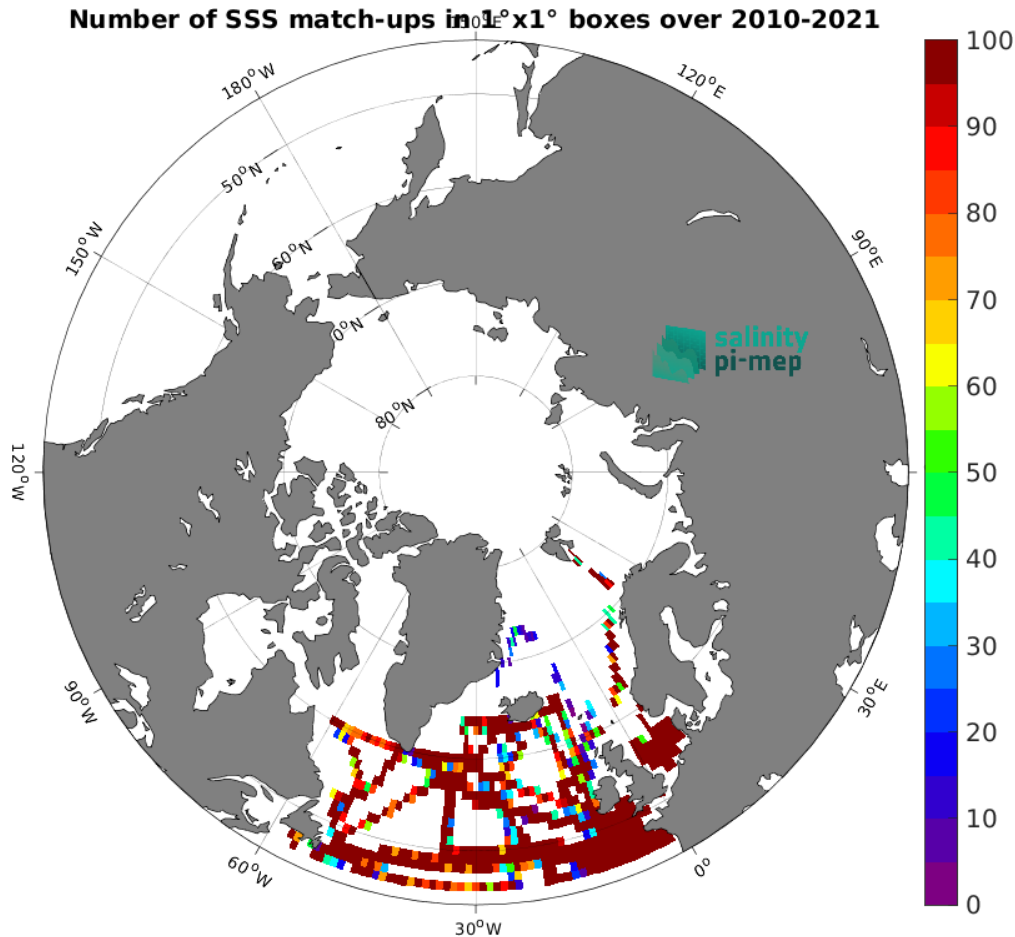
Figure 5: Number of SSS match-ups between TSG (GOSUD-Research-vessel) SSS and the CCI SSS L4 POLAR NH Merged-OI v4.41 - 30-day running (ESA) SSS product for the Global Ocean Pi-MEP region over 1^\circ \times 1^\circ boxes and for the full satellite product period.
