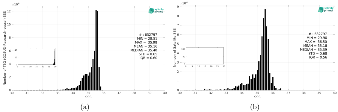
Figure 3: Histograms of SSS from TSG (GOSUD-Research-vessel) (a) and CCI SSS L4 POLAR NH Merged-OI v4.41 - 30-day running (ESA) (b) considering all match-up pairs per bins of 0.1 over the Global Ocean Pi-MEP region and for the full satellite product period.
