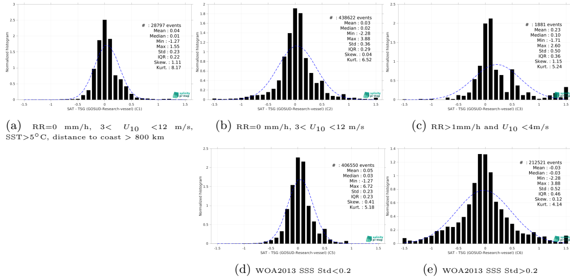
Figure 15: Normalized histogram of \Delta SSS (CCI SSS L4 POLAR NH Merged-OI v4.41 - 30-day running (ESA) - TSG (GOSUD-Research-vessel)) for 5 different subdatasets corresponding to: RR=0 mm/h, 3 < U_{10} < 12 m/s, SST>5°C, distance to coast > 800 km (a), RR=0 mm/h, 3 < U_{10} < 12 m/s (b), RR>1mm/h and U_{10} < 4 m/s (c), WOA2013 SSS Std<0.2 (d), WOA2013 SSS Std>0.2 (e).
