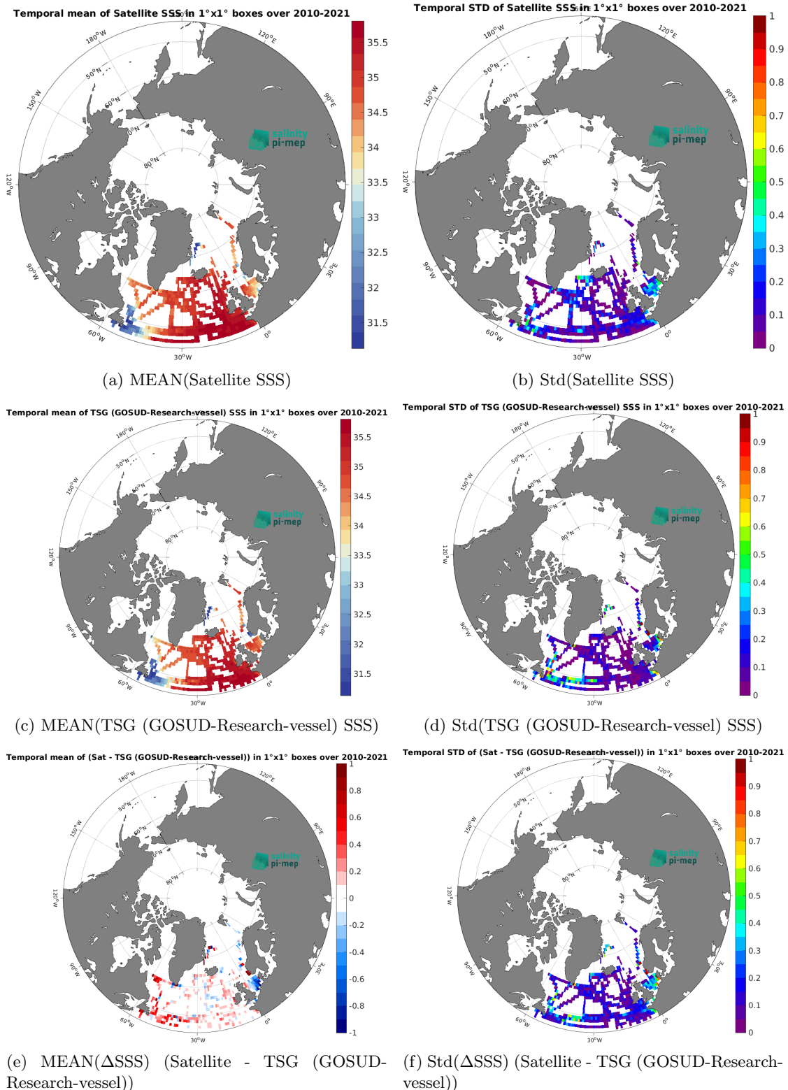
Figure 7: Temporal mean (left) and Std (right) of SSS from CCI SSS L4 POLAR NH Merged-OI v4.41 - 30-day running (ESA) (top), TSG (GOSUD-Research-vessel) (middle), and of \Delta SSS (Satellite - TSG (GOSUD-Research-vessel)). Only match-up pairs are used to generate these maps.
