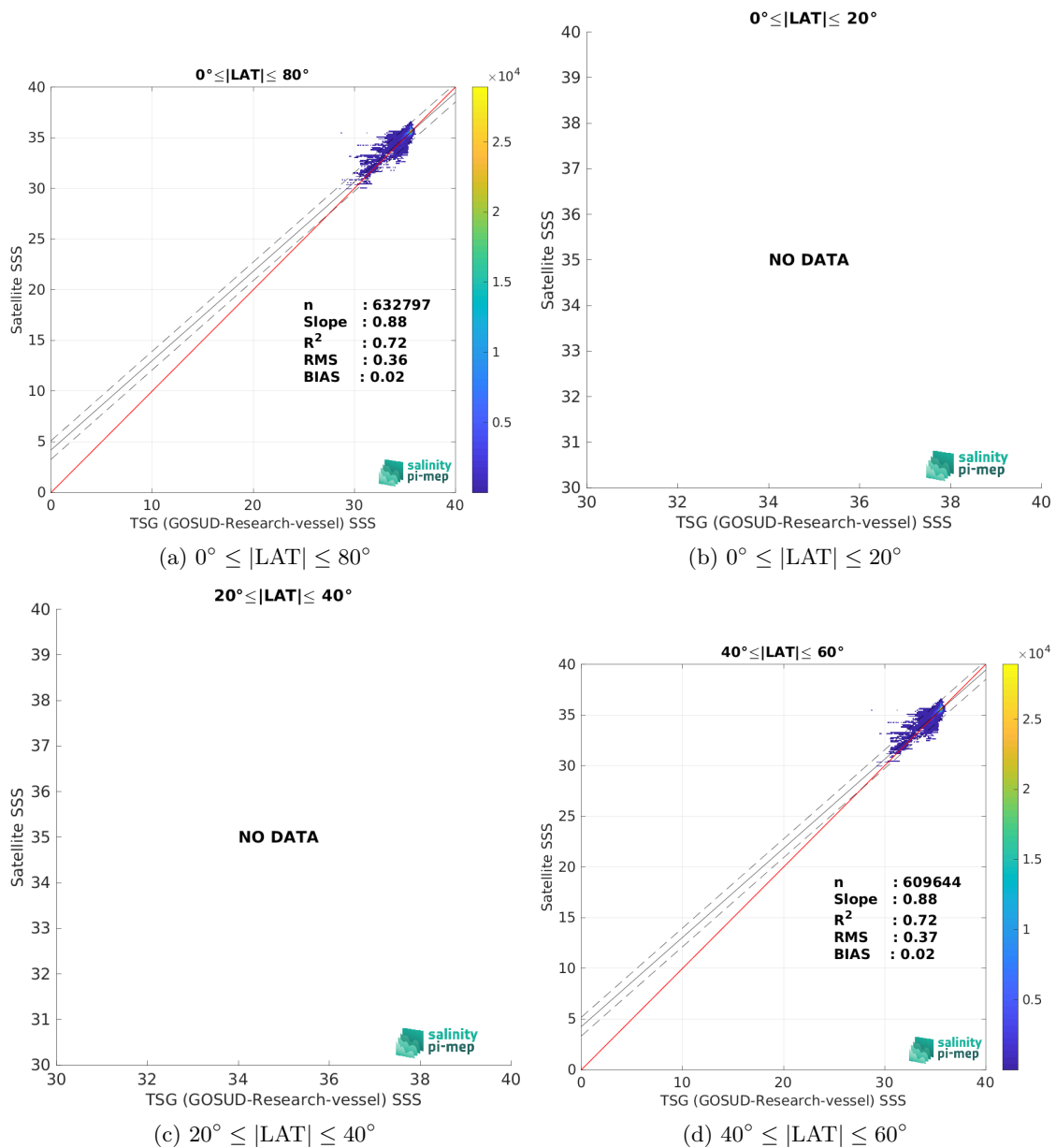
Figure 10: Contour maps of the concentration of CCI SSS L4 POLAR NH Merged-OI v4.41 - 30-day running (ESA) SSS (y-axis) versus TSG (GOSUD-Research-vessel) SSS (x-axis) at match-up pairs for different latitude bands. For each plot, the red line shows x=y . The black thin and dashed lines indicate a linear fit through the data cloud and the \pm 95\% confidence levels, respectively. The number match-up pairs n , the slope and R^2 coefficient of the linear fit, the root mean square (RMS) and the mean bias between satellite and in situ data are indicated for each latitude band in each plots.
