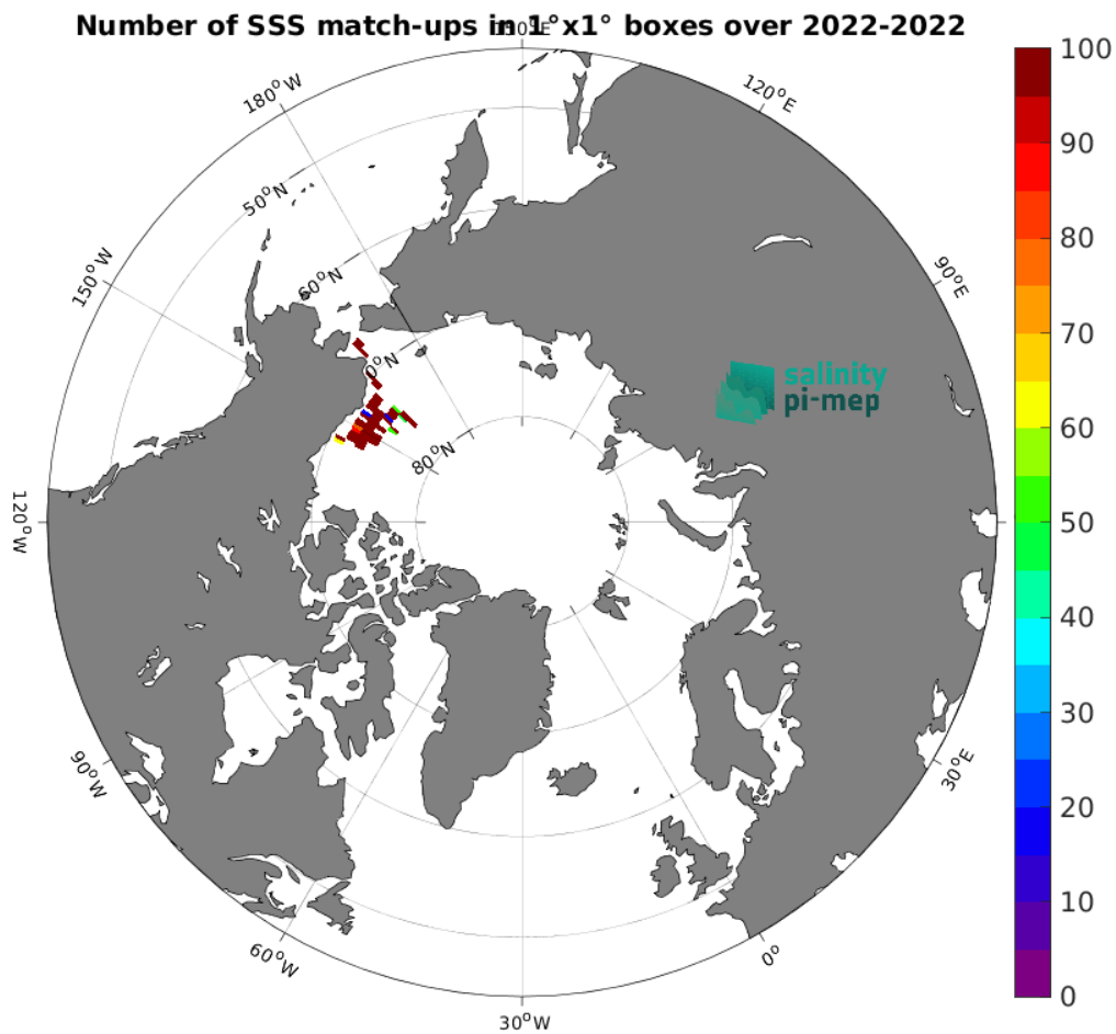
Figure 5: Number of SSS match-ups between SASSIE SSS and the CCI SSS L4 POLAR NH Merged-OI v4.41 - 30-day running (ESA) SSS product for the Global Ocean Pi-MEP region over 1^\circ \times 1^\circ boxes and for the full satellite product period.
