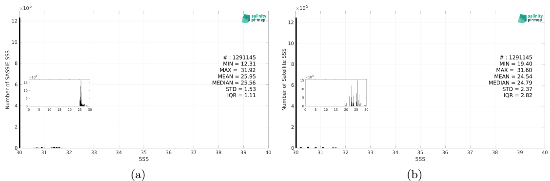
Figure 3: Histograms of SSS from SASSIE (a) and CCI SSS L4 POLAR NH Merged-OI v4.41 - 30-day running (ESA) (b) considering all match-up pairs per bins of 0.1 over the Global Ocean Pi-MEP region and for the full satellite product period.
