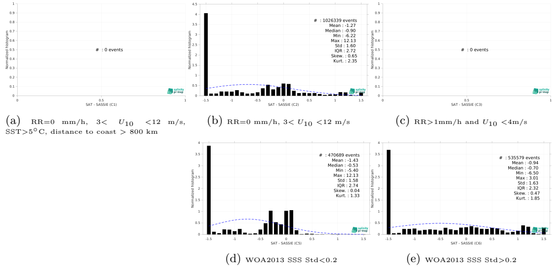
Figure 15: Normalized histogram of \Delta SSS (CCI SSS L4 POLAR NH Merged-OI v4.41 - 30-day running (ESA) - SASSIE) for 5 different subdatasets corresponding to: RR=0 mm/h, 3 < U_{10} < 12 m/s, SST > 5°C, distance to coast > 800 km (a), RR=0 mm/h, 3 < U_{10} < 12 m/s (b), RR > 1mm/h and U_{10} < 4 m/s (c), WOA2013 SSS Std < 0.2 (d), WOA2013 SSS Std > 0.2 (e).
