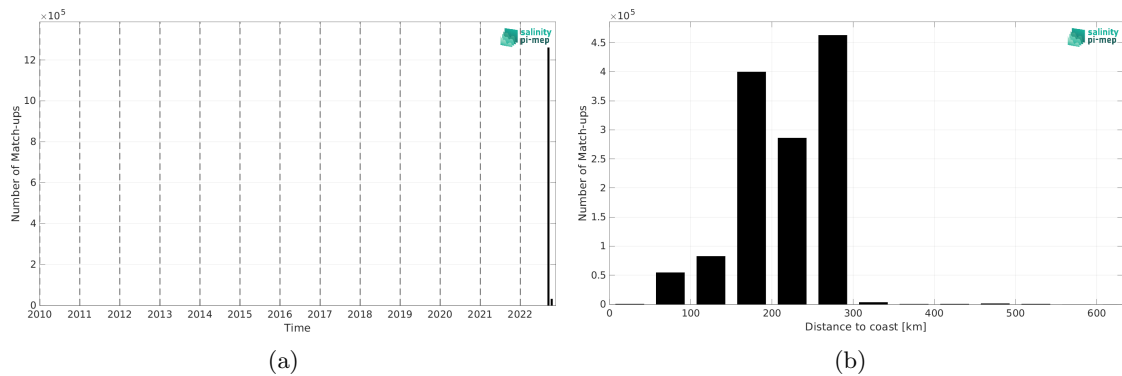
Figure 2: Number of match-ups between SASSIE and CCI SSS L4 POLAR NH Merged-OI v4.41 - 30-day running (ESA) SSS as a function of time (a) and as function of the distance to coast (b) over the Global Ocean Pi-MEP region and for the full satellite product period.
