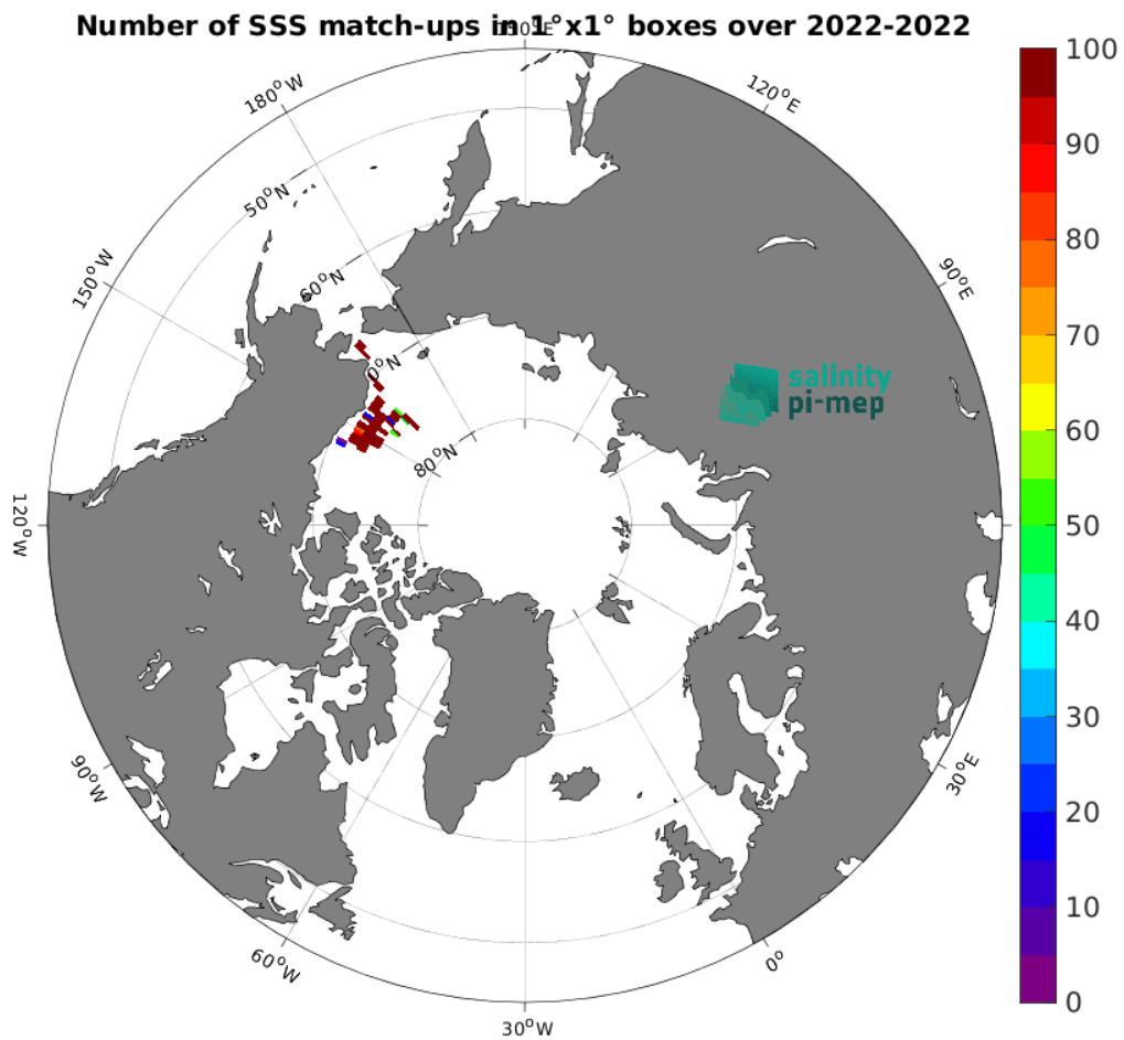
Figure 5: Number of SSS match-ups between SASSIE SSS and the CCI SSS L4 POLAR NH Merged-OI v4.41 - 30-day running (ESA) SSS product for the Global Ocean Pi-MEP region over 1^{\circ} \times 1^{\circ} boxes and for the full satellite product period.
