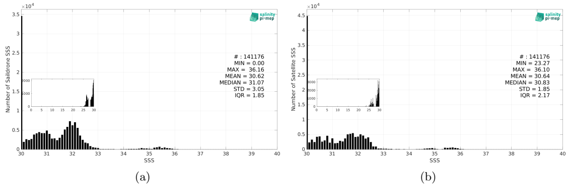
Figure 3: Histograms of SSS from Saildrone (a) and CCI SSS L4 POLAR NH Merged-OI v4.41 - 30-day running (ESA) (b) considering all match-up pairs per bins of 0.1 over the Global Ocean Pi-MEP region and for the full satellite product period.
