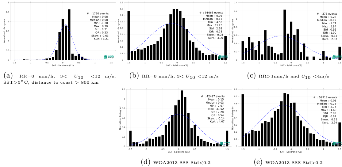
Figure 15: Normalized histogram of \Delta SSS (CCI SSS L4 POLAR NH Merged-OI v4.41 - 30-day running (ESA) - Saildrone) for 5 different subdatasets corresponding to: RR=0 mm/h, 3 < U_{10} < 12 m/s, SST>5°C, distance to coast > 800 km (a), RR=0 mm/h, 3 < U_{10} < 12 m/s (b), RR>1mm/h and U_{10} < 4 m/s (c), WOA2013 SSS Std<0.2 (d), WOA2013 SSS Std>0.2 (e).
