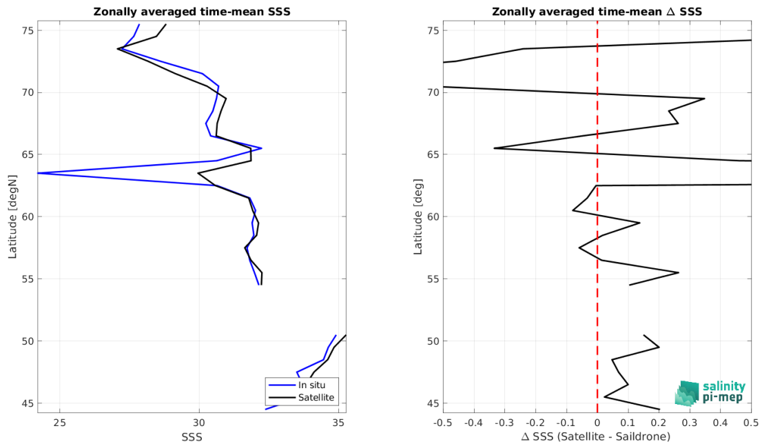
Figure 9: Left panel: Zonal mean SSS from CCI SSS L4 POLAR NH Merged-OI v4.41 - 30-day running (ESA) satellite product (black) and from Saildrone (blue). Right panel: Zonal mean of \Delta SSS (Satellite - Saildrone) for all the collected Pi-MEP match-up pairs estimated over the full satellite product period.
