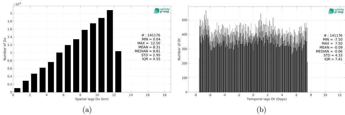
Figure 6: Histograms of the spatial (a) and temporal (b) lags between the location/time of the Saildrone measurement and the date of the corresponding CCI SSS L4 POLAR NH Merged-OI v4.41 - 30-day running (ESA) SSS pixel.
