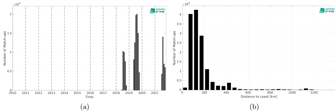
Figure 2: Number of match-ups between Saildrone and CCI SSS L4 POLAR NH Merged-OI v4.41 - 30-day running (ESA) SSS as a function of time (a) and as function of the distance to coast (b) over the Global Ocean Pi-MEP region and for the full satellite product period.
