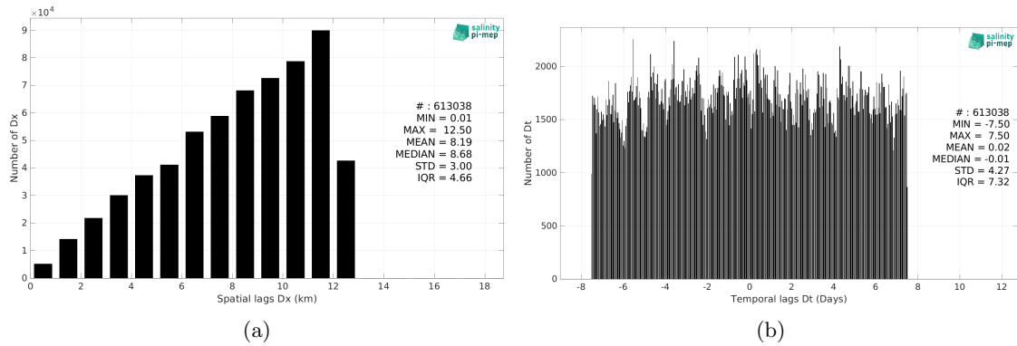
Figure 6: Histograms of the spatial (a) and temporal (b) lags between the location/time of the ICES measurement and the date of the corresponding CCI SSS L4 POLAR NH Merged-OI v4.41 - 30-day running (ESA) SSS pixel.
