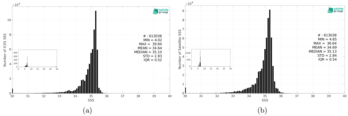
Figure 3: Histograms of SSS from ICES (a) and CCI SSS L4 POLAR NH Merged-OI v4.41 - 30-day running (ESA) (b) considering all match-up pairs per bins of 0.1 over the Global Ocean Pi-MEP region and for the full satellite product period.
