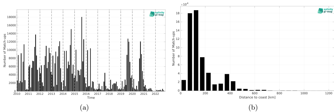
Figure 2: Number of match-ups between ICES and CCI SSS L4 POLAR NH Merged-OI v4.41 - 30-day running (ESA) SSS as a function of time (a) and as function of the distance to coast (b) over the Global Ocean Pi-MEP region and for the full satellite product period.
