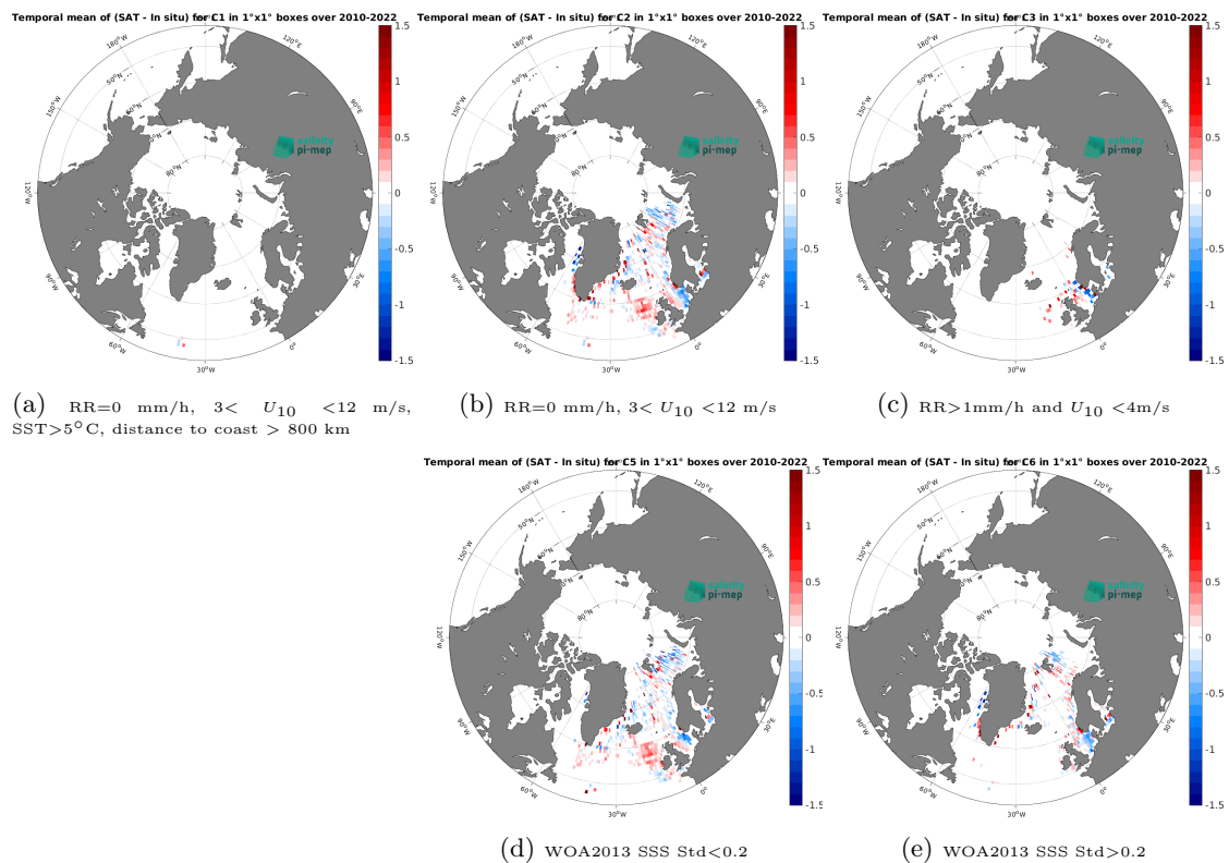
Figure 14: Temporal mean gridded over spatial boxes of size 1^\circ \times 1^\circ of \Delta SSS (CCI SSS L4 POLAR NH Merged-OI v4.41 - 30-day running (ESA) - ICES) for 5 different subdatasets corresponding to:RR=0 mm/h, 3 < U_{10} < 12 m/s, SST >5^\circ C, distance to coast > 800 km (a), RR=0 mm/h, 3 < U_{10} < 12 m/s (b), RR >1 mm/h and U_{10} < 4 m/s (c), WOA2013 SSS Std <0.2 (d), WOA2013 SSS Std >0.2 (e).
