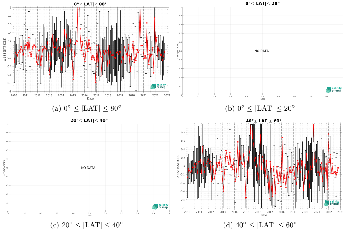
Figure 11: Monthly median (red curves) of \Delta SSS (Satellite - ICES) and \pm 1 Std (black vertical thick bars) as function of time for all the collected Pi-MEP match-up pairs estimated over the Global Ocean Pi-MEP region and for the full satellite product period are shown for different latitude bands: (a) 80^\circ\text{S}-80^\circ\text{N} , (b) 20^\circ\text{S}-20^\circ\text{N} , (c) 40^\circ\text{S}-20^\circ\text{S} and 20^\circ\text{N}-40^\circ\text{N} and (d) 60^\circ\text{S}-40^\circ\text{S} and 40^\circ\text{N}-60^\circ\text{N} .
