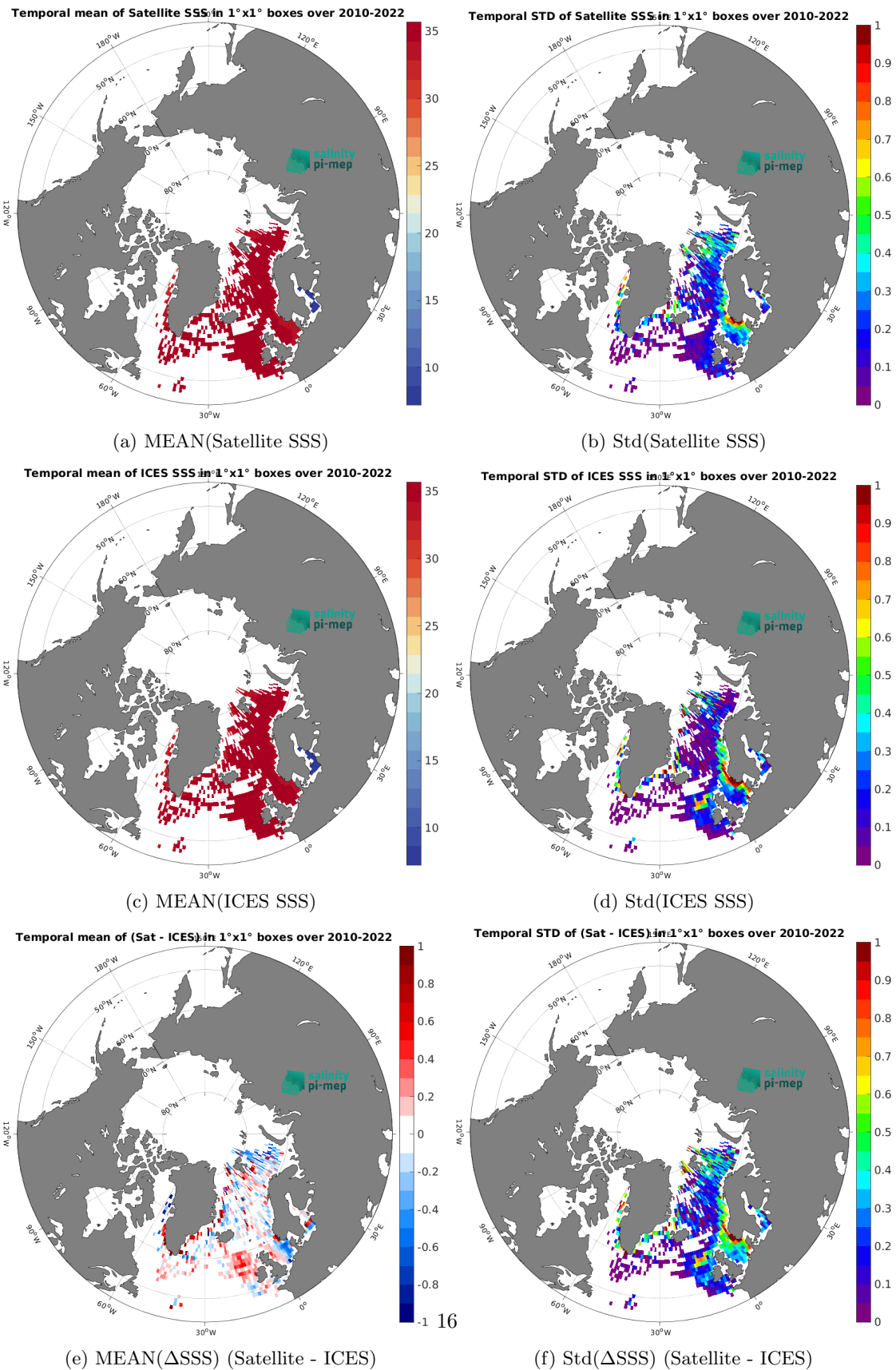
Figure 7: Temporal mean (left) and Std (right) of SSS from CCI SSS L4 POLAR NH Merged-OI v4.41 - 30-day running (ESA) (top), ICES (middle), and of \Delta SSS (Satellite - ICES). Only match-up pairs are used to generate these maps.
