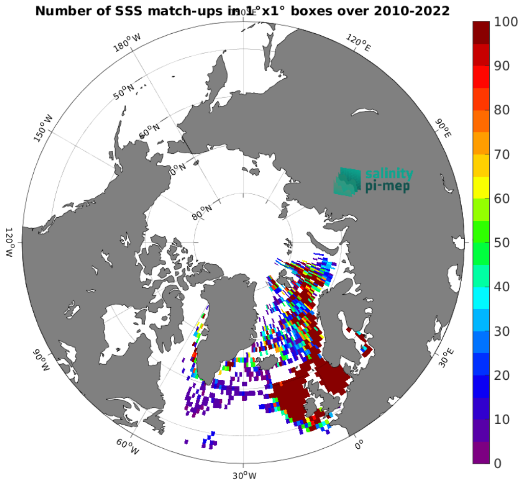
Figure 5: Number of SSS match-ups between ICES SSS and the CCI SSS L4 POLAR NH Merged-OI v4.41 - 30-day running (ESA) SSS product for the Global Ocean Pi-MEP region over 1^{\circ} \times 1^{\circ} boxes and for the full satellite product period.
