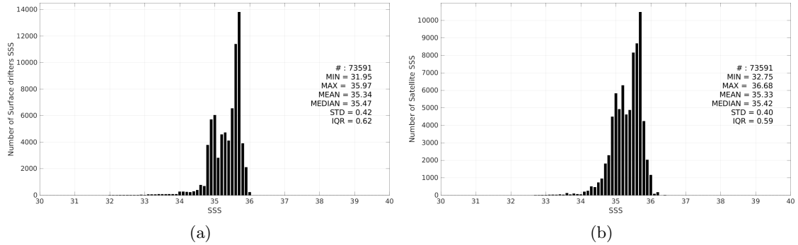
Figure 3: Histograms of SSS from Surface drifters (a) and CCI SSS L4 POLAR NH Merged-OI v4.41 - 30-day running (ESA) (b) considering all match-up pairs per bins of 0.1 over the Global Ocean Pi-MEP region and for the full satellite product period.
