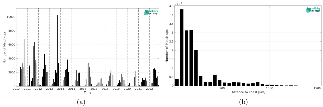
Figure 1: Number of match-ups between TSG (SAMOS) and CCI SSS L4 POLAR NH Merged-OI v4.4 - 7-day running (ESA) SSS as a function of time (a) and as function of the distance to coast (b) over the Global Ocean Pi-MEP region and for the full satellite product period.
