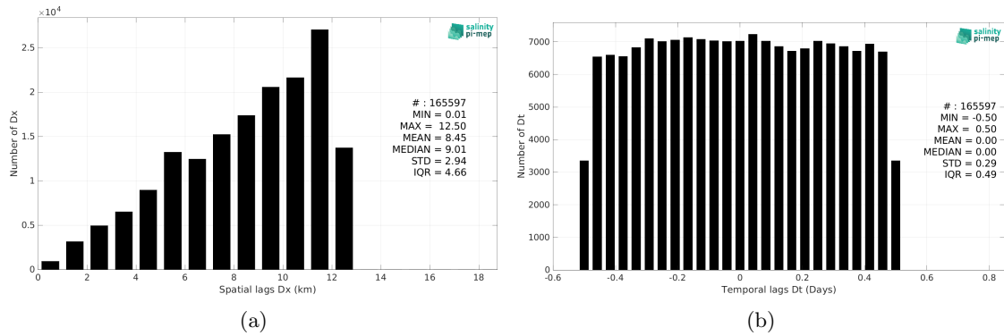
Figure 5: Histograms of the spatial (a) and temporal (b) lags between the location/time of the TSG (SAMOS) measurement and the date of the corresponding CCI SSS L4 POLAR NH Merged-OI v4.4 - 7-day running (ESA) SSS pixel.
