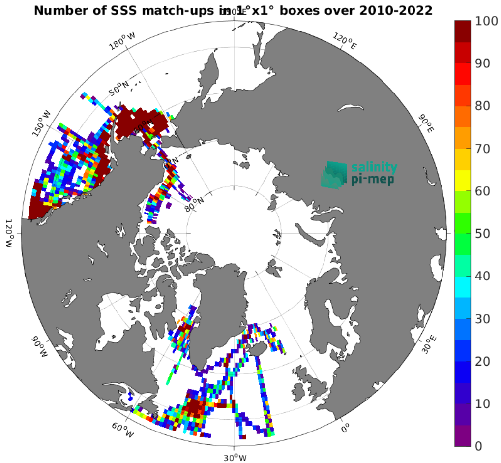
Figure 4: Number of SSS match-ups between TSG (SAMOS) SSS and the CCI SSS L4 POLAR NH Merged-OI v4.4 - 7-day running (ESA) SSS product for the Global Ocean Pi-MEP region over 1^{\circ} \times 1^{\circ} boxes and for the full satellite product period.
