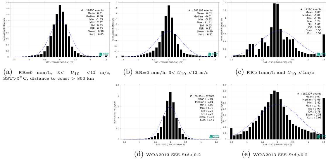
Figure 13: Normalized histogram of \Delta SSS (CCI SSS L4 POLAR NH Merged-OI v4.4 - 7-day running (ESA) - TSG (LEGOS-DM)) for 5 different subdatasets corresponding to: RR=0 mm/h, 3 < U_{10} < 12 m/s, SST > 5°C, distance to coast > 800 km (a), RR=0 mm/h, 3 < U_{10} < 12 m/s (b), RR > 1mm/h and U_{10} < 4 m/s (c), WOA2013 SSS Std < 0.2 (d), WOA2013 SSS Std > 0.2 (e).
