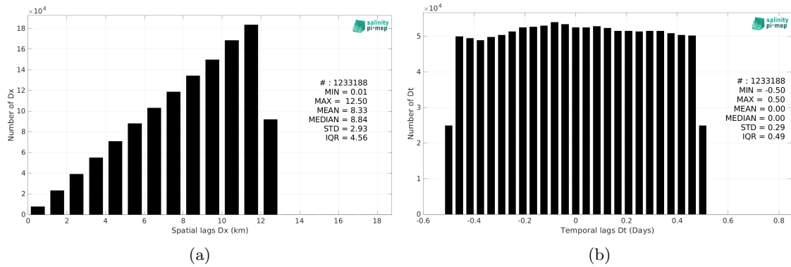
Figure 5: Histograms of the spatial (a) and temporal (b) lags between the location/time of the TSG (LEGOS-DM) measurement and the date of the corresponding CCI SSS L4 POLAR NH Merged-OI v4.4 - 7-day running (ESA) SSS pixel.
