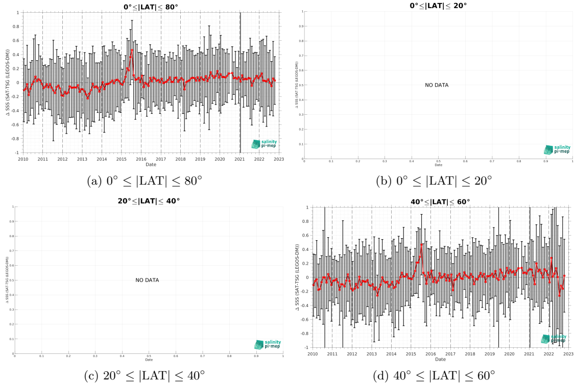
Figure 10: Monthly median (red curves) of \Delta SSS (Satellite - in situ ) between CCI SSS L4 POLAR NH Merged-OI v4.4 - 7-day running (ESA) and TSG (LEGOS-DM) SSS as function of time for all the collected Pi-MEP match-up pairs estimated over the Global Ocean Pi-MEP region and for the full satellite product period are shown for different latitude bands: (a) 80^\circ\text{S}-80^\circ\text{N} , (b) 20^\circ\text{S}-20^\circ\text{N} , (c) 40^\circ\text{S}-20^\circ\text{S} and 20^\circ\text{N}-40^\circ\text{N} and (d) 60^\circ\text{S}-40^\circ\text{S} and 40^\circ\text{N}-60^\circ\text{N} .
