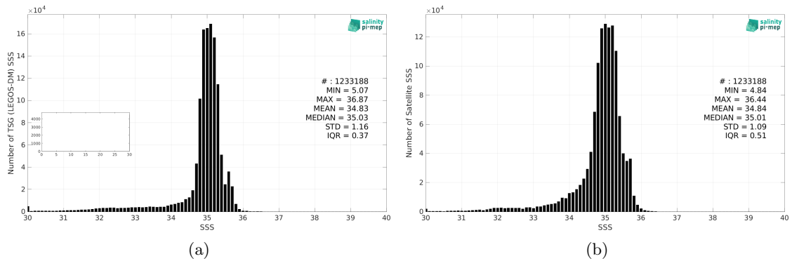
Figure 2: Histograms of SSS from TSG (LEGOS-DM) (a) and CCI SSS L4 POLAR NH Merged-OI v4.4 - 7-day running (ESA) (b) considering all match-up pairs per bins of 0.1 over the Global Ocean Pi-MEP region and for the full satellite product period.
