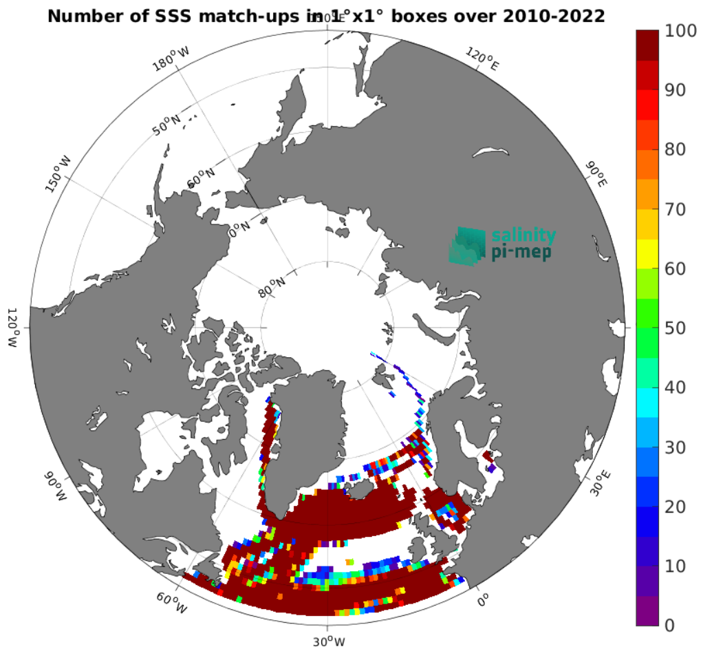
Figure 4: Number of SSS match-ups between TSG (LEGOS-DM) SSS and the CCI SSS L4 POLAR NH Merged-OI v4.4 - 7-day running (ESA) SSS product for the Global Ocean Pi-MEP region over 1^{\circ} \times 1^{\circ} boxes and for the full satellite product period.
