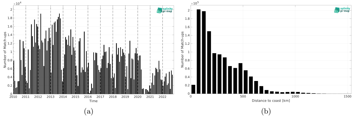
Figure 1: Number of match-ups between TSG (LEGOS-DM) and CCI SSS L4 POLAR NH Merged-OI v4.4 - 7-day running (ESA) SSS as a function of time (a) and as function of the distance to coast (b) over the Global Ocean Pi-MEP region and for the full satellite product period.
