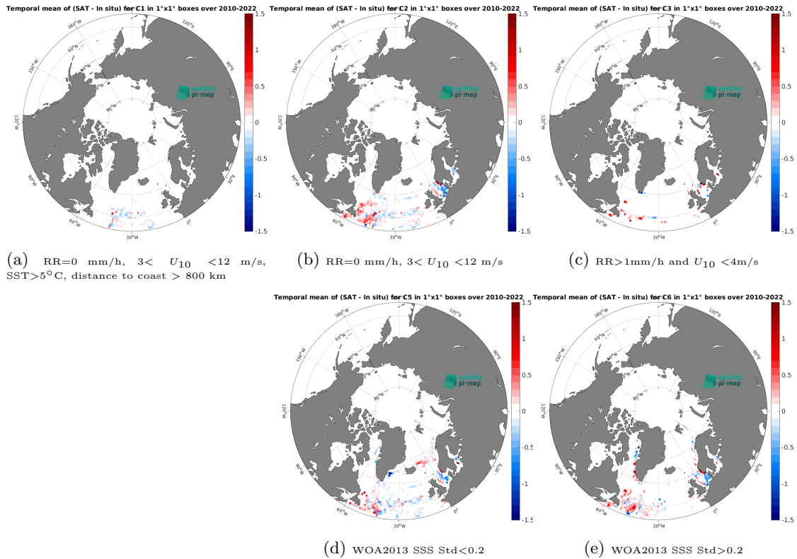
Figure 12: Temporal mean gridded over spatial boxes of size 1^{\circ}\times 1^{\circ} of \Delta\text{SSS} (CCI SSS L4 POLAR NH Merged-OI v4.4 - 7-day running (ESA) - TSG (LEGOS-DM)) for 5 different subdatasets corresponding to:RR=0 mm/h, 3 < U_{10} < 12 m/s, SST > 5^{\circ}\text{C} , distance to coast > 800 km (a), RR=0 mm/h, 3 < U_{10} < 12 m/s (b), RR > 1 mm/h and U_{10} < 4 m/s (c), WOA2013 SSS Std < 0.2 (d), WOA2013 SSS Std > 0.2 (e).
