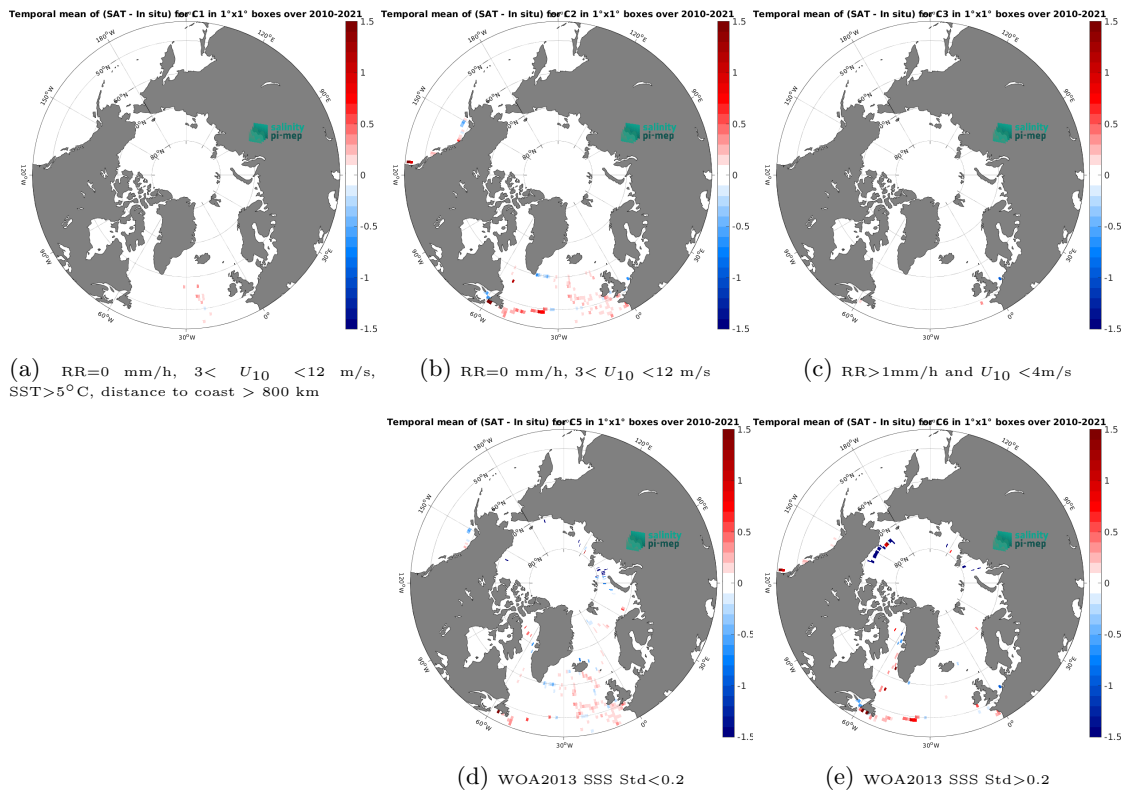
Figure 12: Temporal mean gridded over spatial boxes of size 1°x1° of \Delta SSS (CCI SSS L4 POLAR NH Merged-OI v4.4 - 7-day running (ESA) - TSG (GOSUD-Sailing-ship)) for 5 different subdatasets corresponding to:RR=0 mm/h, 3 < U_{10} < 12 m/s, SST>5°C, distance to coast > 800 km (a), RR=0 mm/h, 3 < U_{10} < 12 m/s (b), RR>1mm/h and U_{10} < 4 m/s (c), WOA2013 SSS Std<0.2 (d), WOA2013 SSS Std>0.2 (e).
