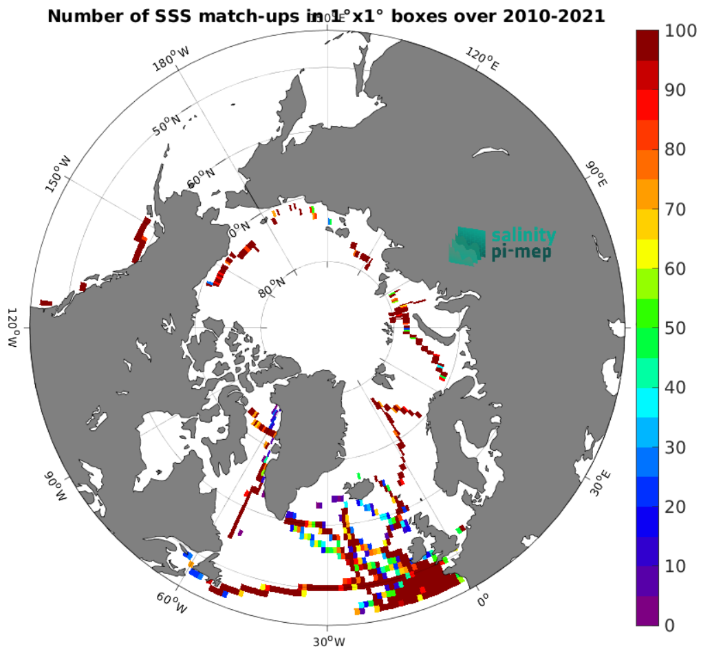
Figure 4: Number of SSS match-ups between TSG (GOSUD-Sailing-ship) SSS and the CCI SSS L4 POLAR NH Merged-OI v4.4 - 7-day running (ESA) SSS product for the Global Ocean Pi-MEP region over 1^{\circ} \times 1^{\circ} boxes and for the full satellite product period.
