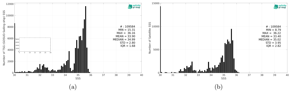
Figure 2: Histograms of SSS from TSG (GOSUD-Sailing-ship) (a) and CCI SSS L4 POLAR NH Merged-OI v4.4 - 7-day running (ESA) (b) considering all match-up pairs per bins of 0.1 over the Global Ocean Pi-MEP region and for the full satellite product period.
