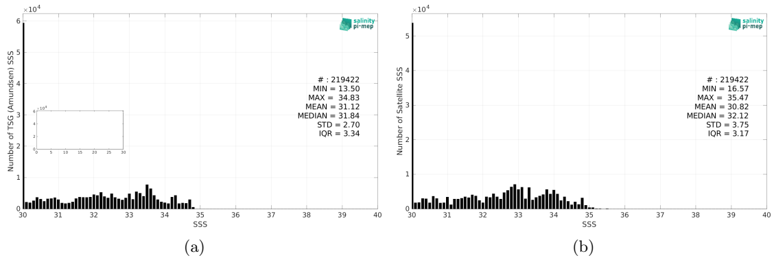
Figure 2: Histograms of SSS from TSG (Amundsen) (a) and CCI SSS L4 POLAR NH Merged-OI v4.4 - 7-day running (ESA) (b) considering all match-up pairs per bins of 0.1 over the Global Ocean Pi-MEP region and for the full satellite product period.
