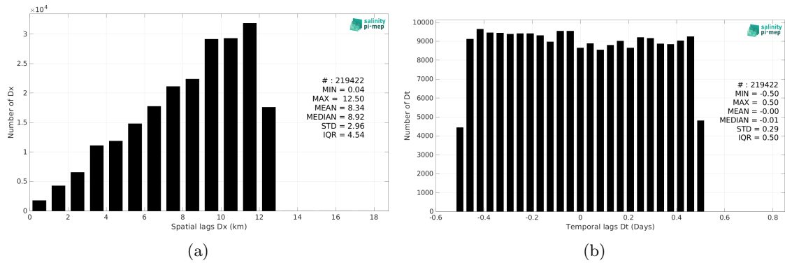
Figure 5: Histograms of the spatial (a) and temporal (b) lags between the location/time of the TSG (Amundsen) measurement and the date of the corresponding CCI SSS L4 POLAR NH Merged-OI v4.4 - 7-day running (ESA) SSS pixel.
