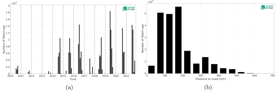
Figure 1: Number of match-ups between TSG (Amundsen) and CCI SSS L4 POLAR NH Merged-OI v4.4 - 7-day running (ESA) SSS as a function of time (a) and as function of the distance to coast (b) over the Global Ocean Pi-MEP region and for the full satellite product period.
