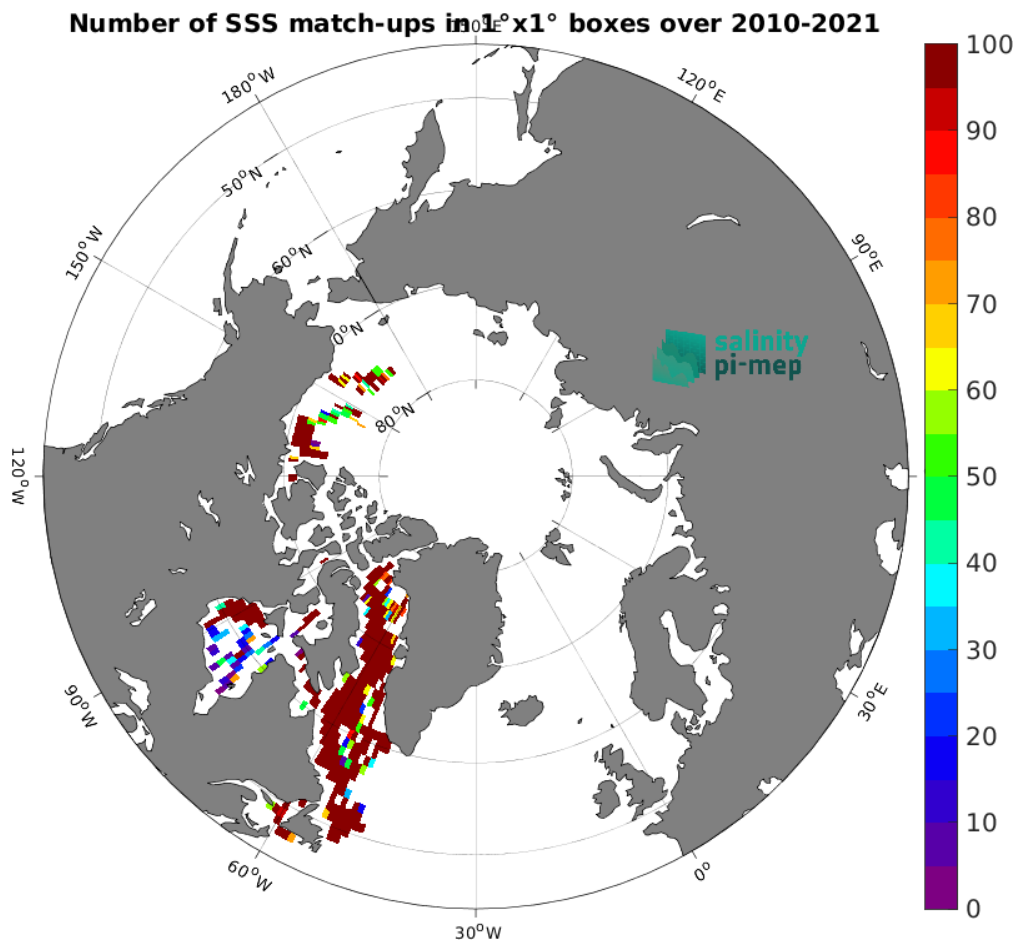
Figure 4: Number of SSS match-ups between TSG (Amundsen) SSS and the CCI SSS L4 POLAR NH Merged-OI v4.4 - 7-day running (ESA) SSS product for the Global Ocean Pi-MEP region over 1^{\circ} \times 1^{\circ} boxes and for the full satellite product period.
