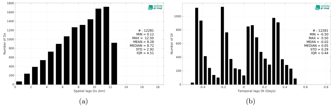
Figure 5: Histograms of the spatial (a) and temporal (b) lags between the location/time of the Marine mammals measurement and the date of the corresponding CCI SSS L4 POLAR NH Merged-OI v4.4 - 7-day running (ESA) SSS pixel.
