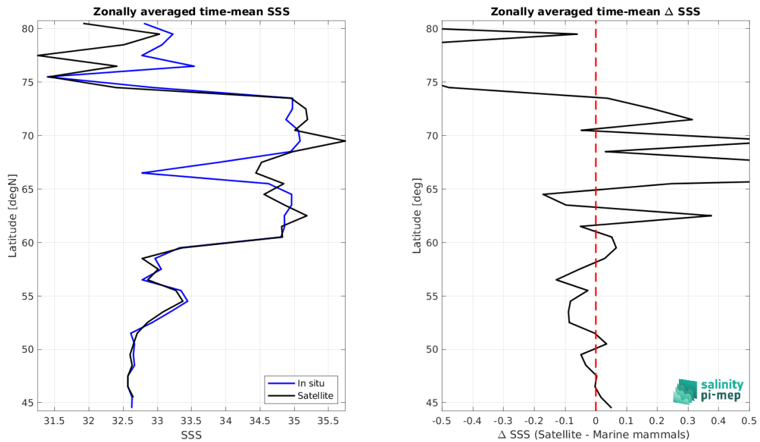
Figure 8: Left panel: Zonal mean SSS from CCI SSS L4 POLAR NH Merged-OI v4.4 - 7-day running (ESA) satellite product (black) and from Marine mammals (blue). Right panel: Zonal mean of \Delta SSS (Satellite - Marine mammals) for all the collected Pi-MEP match-up pairs estimated over the full satellite product period.
