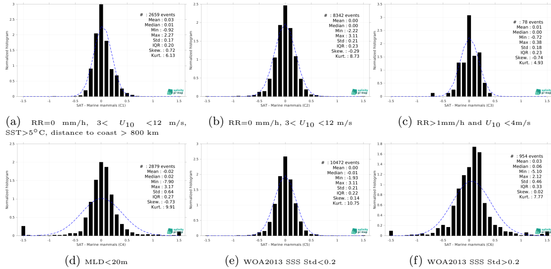
Figure 13: Normalized histogram of \Delta SSS (CCI SSS L4 POLAR NH Merged-OI v4.4 - 7-day running (ESA) - Marine mammals) for 6 different subdatasets corresponding to: RR=0 mm/h, 3 < U_{10} < 12 m/s, SST>5°C, distance to coast > 800 km (a), RR=0 mm/h, 3 < U_{10} < 12 m/s (b), RR>1mm/h and U_{10} < 4 m/s (c), MLD<20m (d), WOA2013 SSS Std<0.2 (e), WOA2013 SSS Std>0.2 (f).
