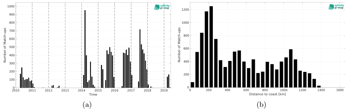
Figure 1: Number of match-ups between Marine mammals and CCI SSS L4 POLAR NH Merged-OI v4.4 - 7-day running (ESA) SSS as a function of time (a) and as function of the distance to coast (b) over the Global Ocean Pi-MEP region and for the full satellite product period.
