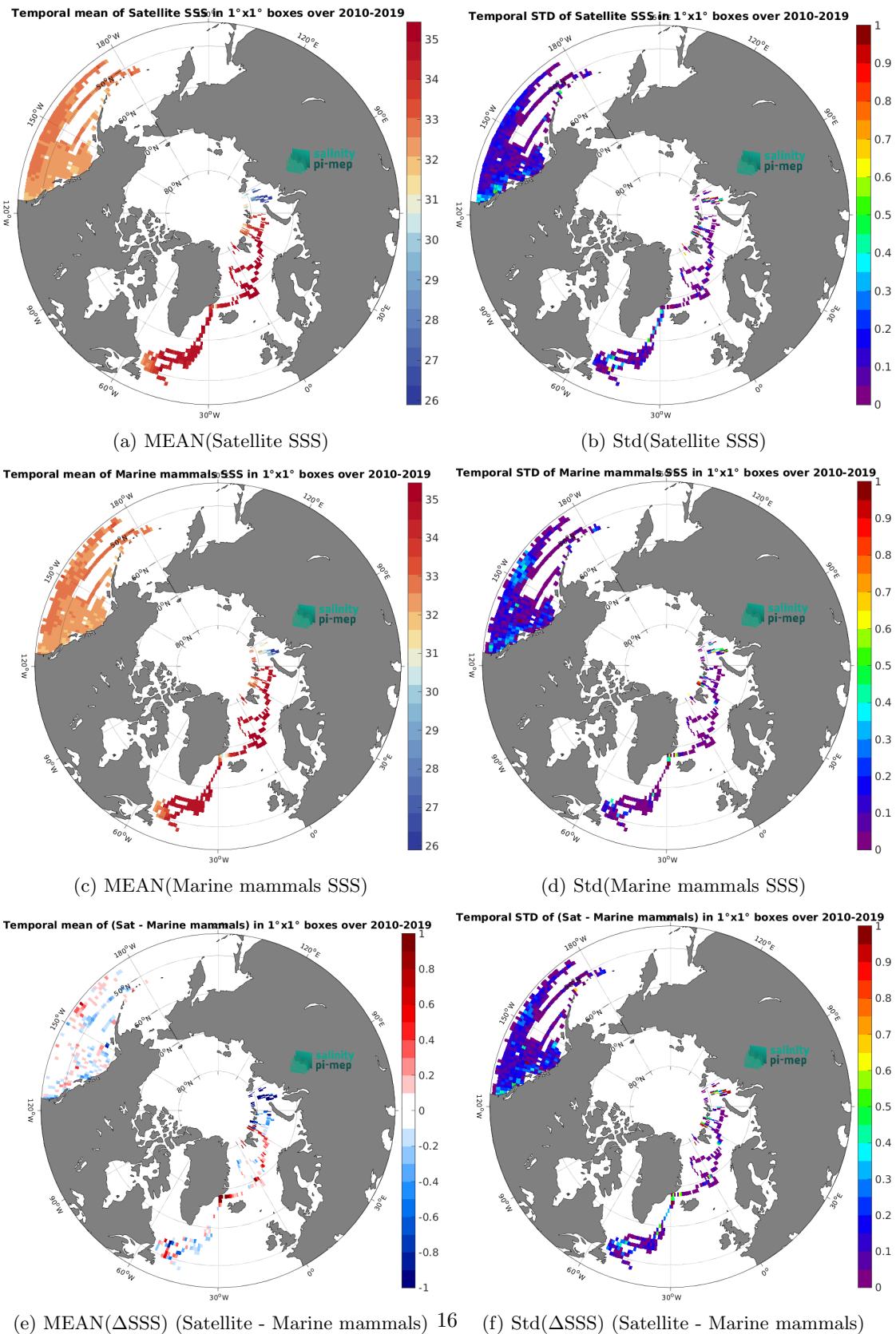
Figure 6: Temporal mean (left) and Std (right) of SSS from CCI SSS L4 POLAR NH Merged-OI v4.4 - 7-day running (ESA) (top), Marine mammals (middle), and of \Delta SSS (Satellite - Marine mammals). Only match-up pairs are used to generate these maps.
