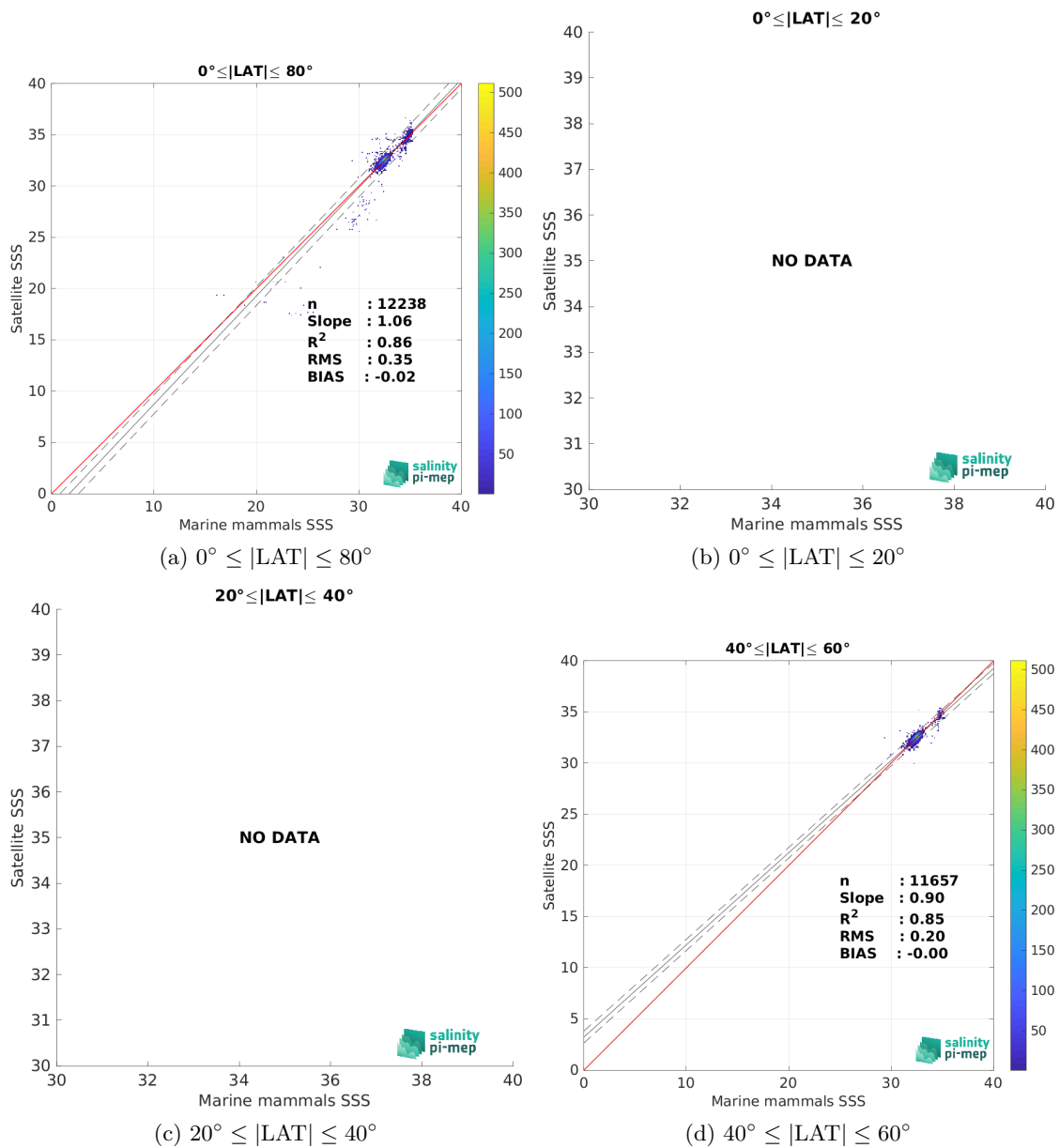
Figure 9: Contour maps of the concentration of CCI SSS L4 POLAR NH Merged-OI v4.4 - 7-day running (ESA) SSS (y-axis) versus Marine mammals SSS (x-axis) at match-up pairs for different latitude bands. For each plot, the red line shows x=y . The black thin and dashed lines indicate a linear fit through the data cloud and the \pm 95\% confidence levels, respectively. The number match-up pairs n , the slope and R^2 coefficient of the linear fit, the root mean square (RMS) and the mean bias between satellite and in situ data are indicated for each latitude band in each plots.
