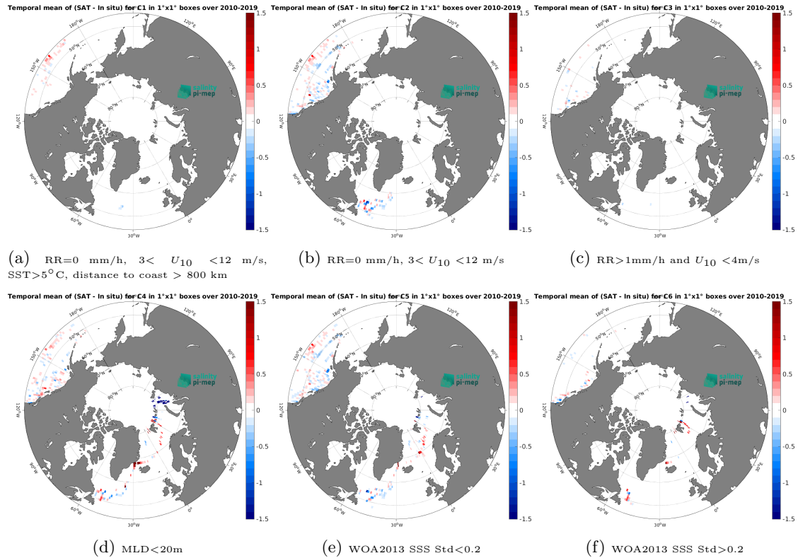
Figure 12: Temporal mean gridded over spatial boxes of size 1^{\circ}\times 1^{\circ} of \Delta\text{SSS} (CCI SSS L4 POLAR NH Merged-OI v4.4 - 7-day running (ESA) - Marine mammals) for 6 different subdatasets corresponding to:RR=0 mm/h, 3 < U_{10} < 12 m/s, SST > 5^{\circ}\text{C} , distance to coast > 800 km (a), RR=0 mm/h, 3 < U_{10} < 12 m/s (b), RR > 1 mm/h and U_{10} < 4 m/s (c),MLD < 20 m (d),WOA2013 SSS Std < 0.2 (e),WOA2013 SSS Std > 0.2 (f).
