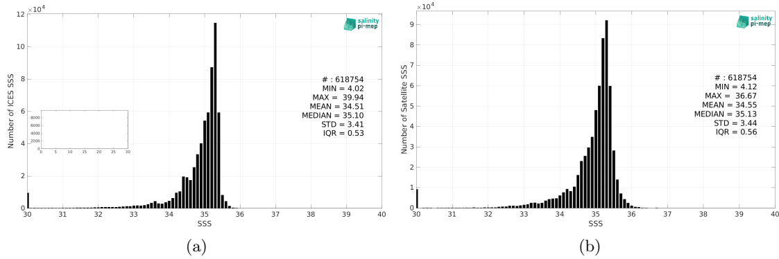
Figure 2: Histograms of SSS from ICES (a) and CCI SSS L4 POLAR NH Merged-OI v4.4 - 7-day running (ESA) (b) considering all match-up pairs per bins of 0.1 over the Global Ocean Pi-MEP region and for the full satellite product period.
