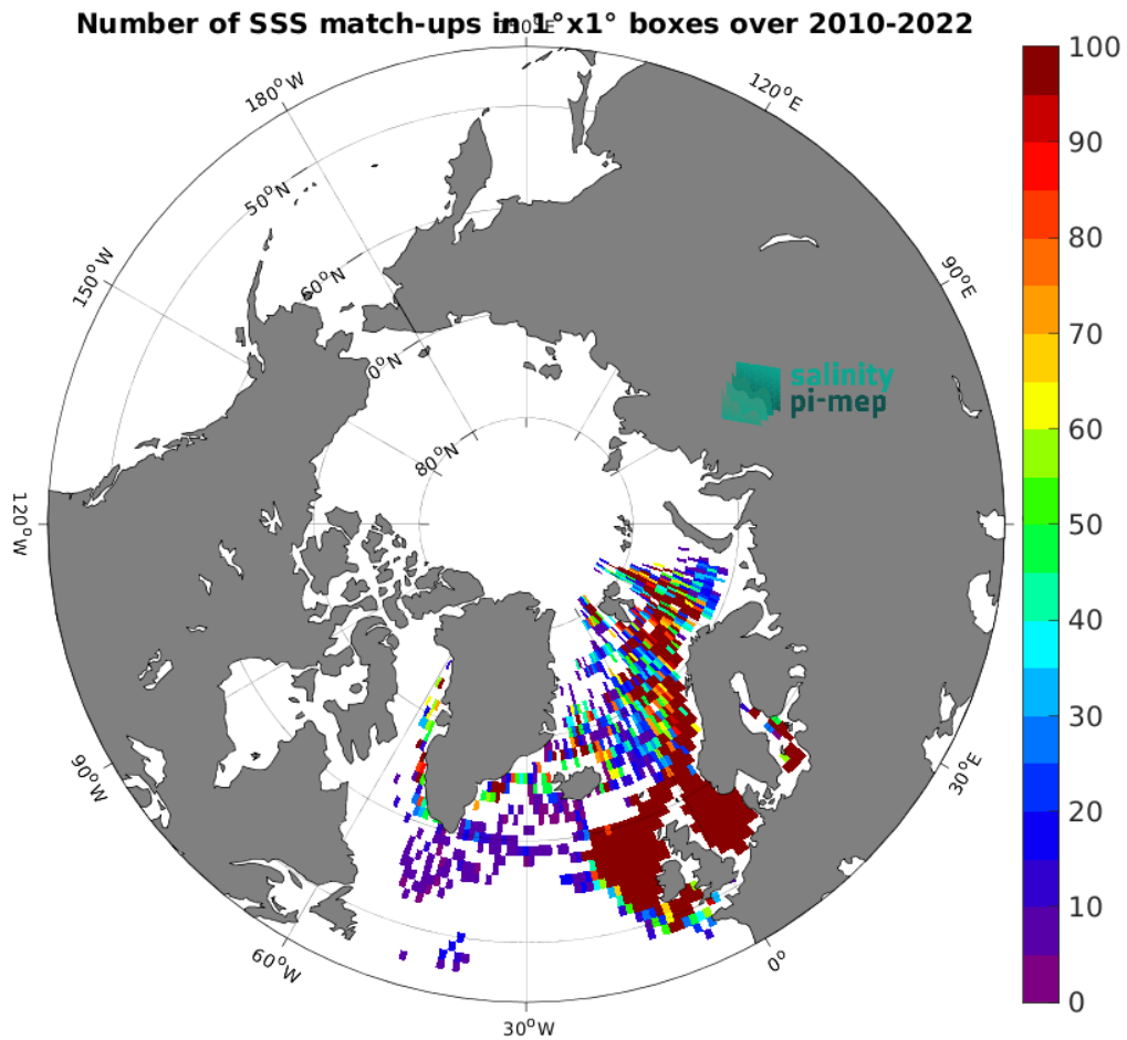
Figure 4: Number of SSS match-ups between ICES SSS and the CCI SSS L4 POLAR NH Merged-OI v4.4 - 7-day running (ESA) SSS product for the Global Ocean Pi-MEP region over 1^{\circ} \times 1^{\circ} boxes and for the full satellite product period.
