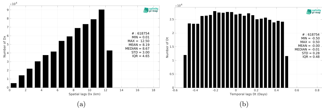
Figure 5: Histograms of the spatial (a) and temporal (b) lags between the location/time of the ICES measurement and the date of the corresponding CCI SSS L4 POLAR NH Merged-OI v4.4 - 7-day running (ESA) SSS pixel.
