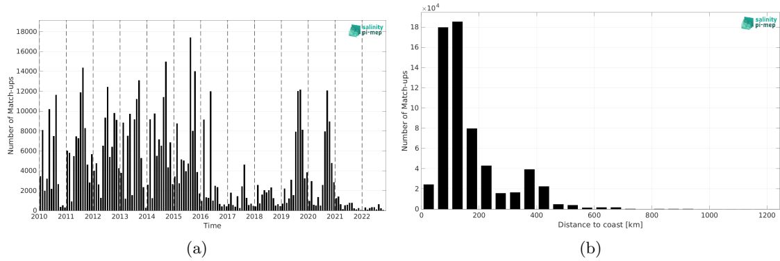
Figure 1: Number of match-ups between ICES and CCI SSS L4 POLAR NH Merged-OI v4.4 - 7-day running (ESA) SSS as a function of time (a) and as function of the distance to coast (b) over the Global Ocean Pi-MEP region and for the full satellite product period.
