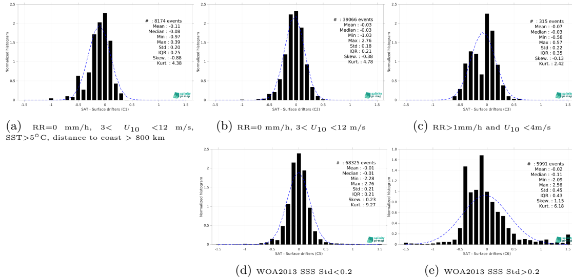
Figure 12: Normalized histogram of \Delta SSS (CCI SSS L4 POLAR NH Merged-OI v4.4 - 7-day running (ESA) - Surface drifters) for 5 different subdatasets corresponding to: RR=0 mm/h, 3 < U_{10} < 12 m/s, SST > 5°C, distance to coast > 800 km (a), RR=0 mm/h, 3 < U_{10} < 12 m/s (b), RR > 1mm/h and U_{10} < 4 m/s (c), WOA2013 SSS Std < 0.2 (d), WOA2013 SSS Std > 0.2 (e).
