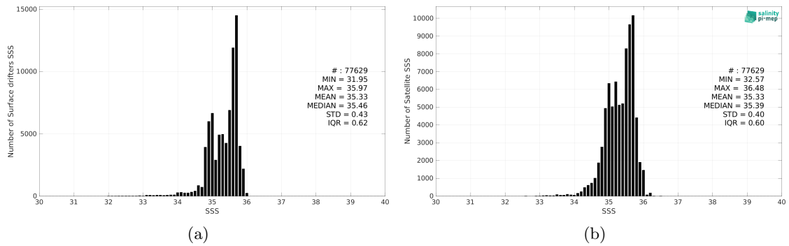
Figure 2: Histograms of SSS from Surface drifters (a) and CCI SSS L4 POLAR NH Merged-OI v4.4 - 7-day running (ESA) (b) considering all match-up pairs per bins of 0.1 over the Global Ocean Pi-MEP region and for the full satellite product period.
