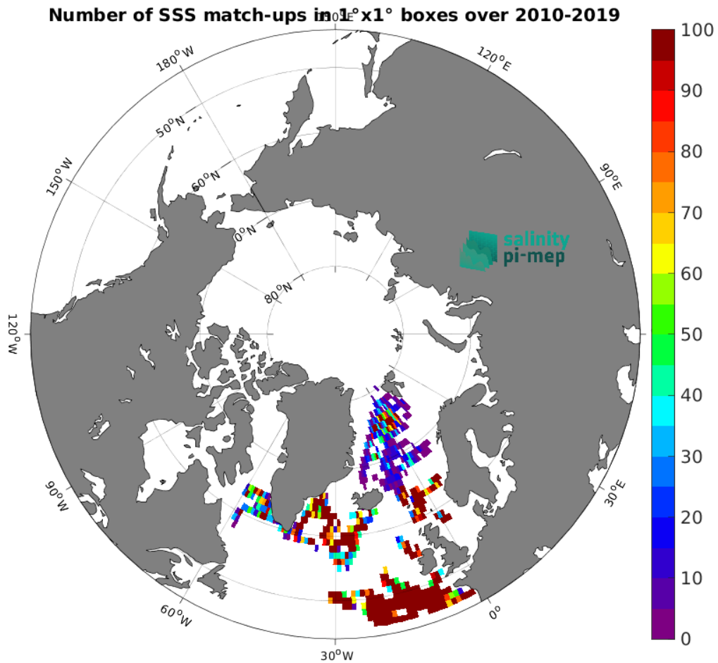
Figure 3: Number of SSS match-ups between Surface drifters SSS and the CCI SSS L4 POLAR NH Merged-OI v4.4 - 7-day running (ESA) SSS product for the Global Ocean Pi-MEP region over 1^{\circ} \times 1^{\circ} boxes and for the full satellite product period.
