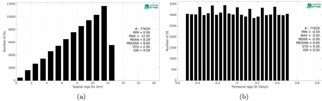
Figure 4: Histograms of the spatial (a) and temporal (b) lags between the location/time of the Surface drifters measurement and the date of the corresponding CCI SSS L4 POLAR NH Merged-OI v4.4 - 7-day running (ESA) SSS pixel.
