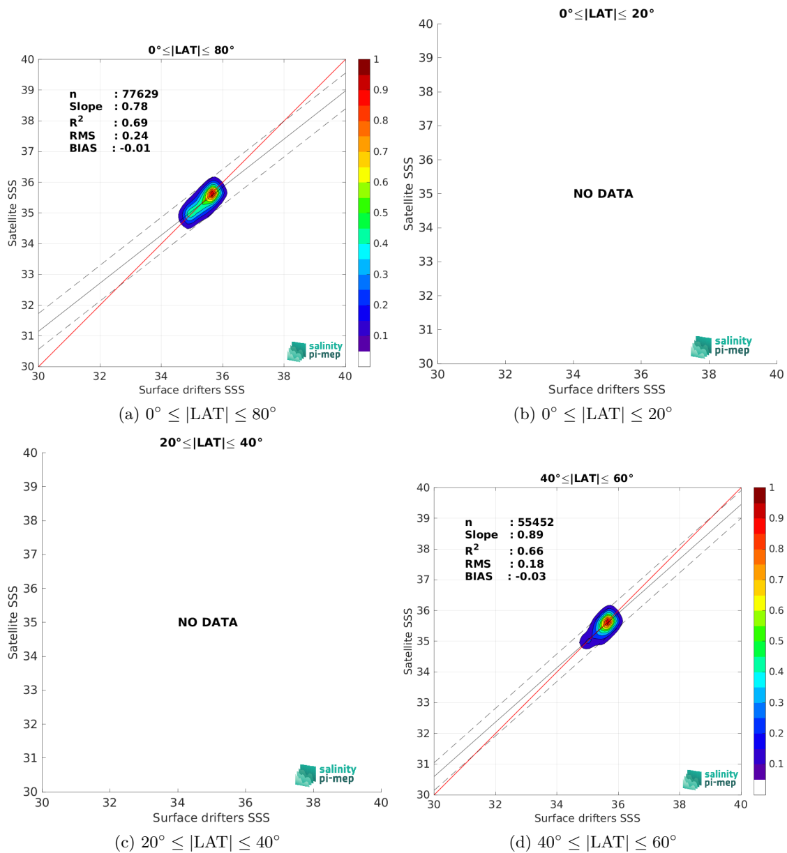
Figure 8: Contour maps of the concentration of CCI SSS L4 POLAR NH Merged-OI v4.4 - 7-day running (ESA) SSS (y-axis) versus Surface drifters SSS (x-axis) at match-up pairs for different latitude bands. For each plot, the red line shows x=y . The black thin and dashed lines indicate a linear fit through the data cloud and the \pm 95\% confidence levels, respectively. The number match-up pairs n , the slope and R^2 coefficient of the linear fit, the root mean square (RMS) and the mean bias between satellite and in situ data are indicated for each latitude band in each plots.
