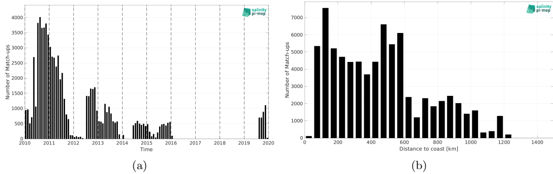
Figure 1: Number of match-ups between Surface drifters and CCI SSS L4 POLAR NH Merged-OI v4.4 - 7-day running (ESA) SSS as a function of time (a) and as function of the distance to coast (b) over the Global Ocean Pi-MEP region and for the full satellite product period.
