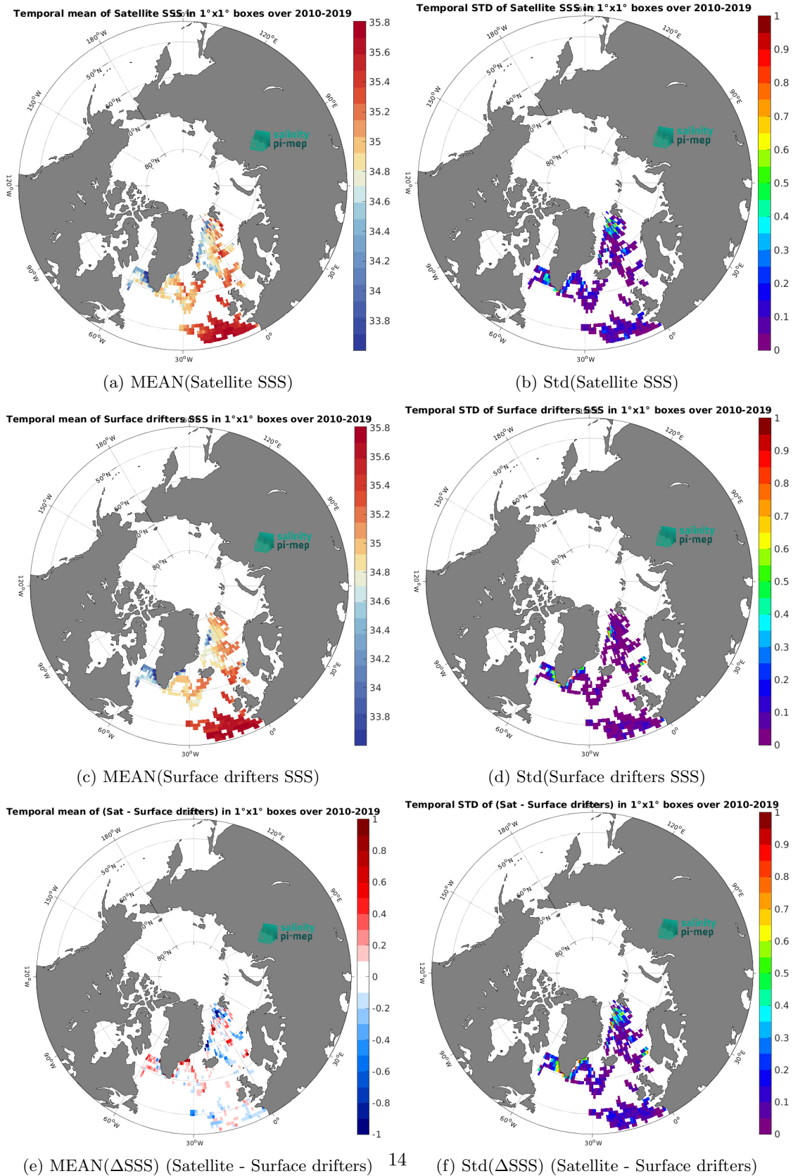
Figure 5: Temporal mean (left) and Std (right) of SSS from CCI SSS L4 POLAR NH Merged-OI v4.4 - 7-day running (ESA) (top), Surface drifters (middle), and of \Delta SSS (Satellite - Surface drifters). Only match-up pairs are used to generate these maps.
