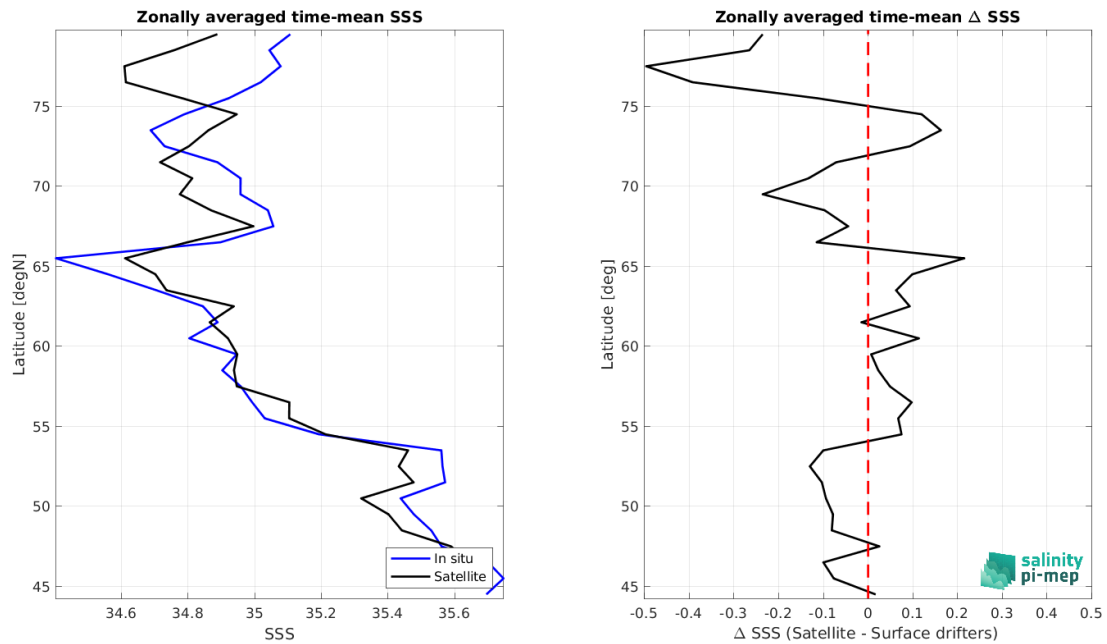
Figure 7: Left panel: Zonal mean SSS from CCI SSS L4 POLAR NH Merged-OI v4.4 - 7-day running (ESA) satellite product (black) and from Surface drifters (blue). Right panel: Zonal mean of \Delta SSS (Satellite - Surface drifters) for all the collected Pi-MEP match-up pairs estimated over the full satellite product period.
