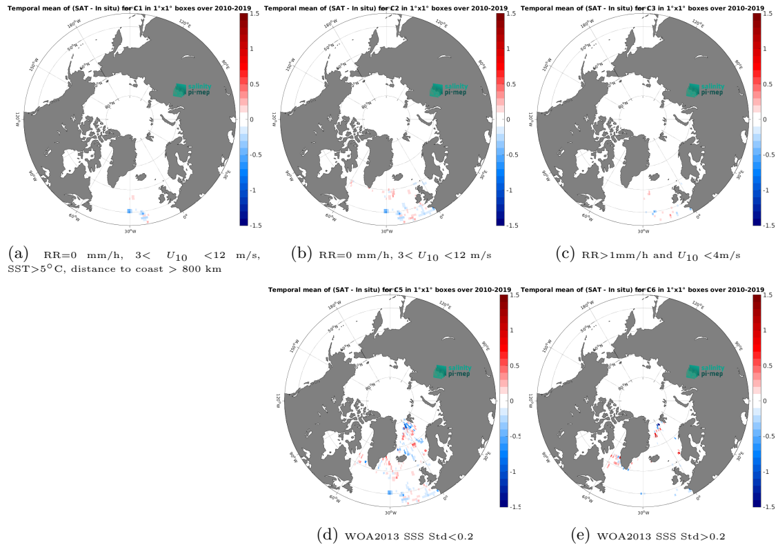
Figure 11: Temporal mean gridded over spatial boxes of size 1^{\circ}\times 1^{\circ} of \Delta\text{SSS} (CCI SSS L4 POLAR NH Merged-OI v4.4 - 7-day running (ESA) - Surface drifters) for 5 different subdatasets corresponding to:RR=0 mm/h, 3 < U_{10} < 12 m/s, SST >5^{\circ}\text{C} , distance to coast > 800 km (a), RR=0 mm/h, 3 < U_{10} < 12 m/s (b), RR >1 mm/h and U_{10} < 4 m/s (c), WOA2013 SSS Std <0.2 (d), WOA2013 SSS Std >0.2 (e).
