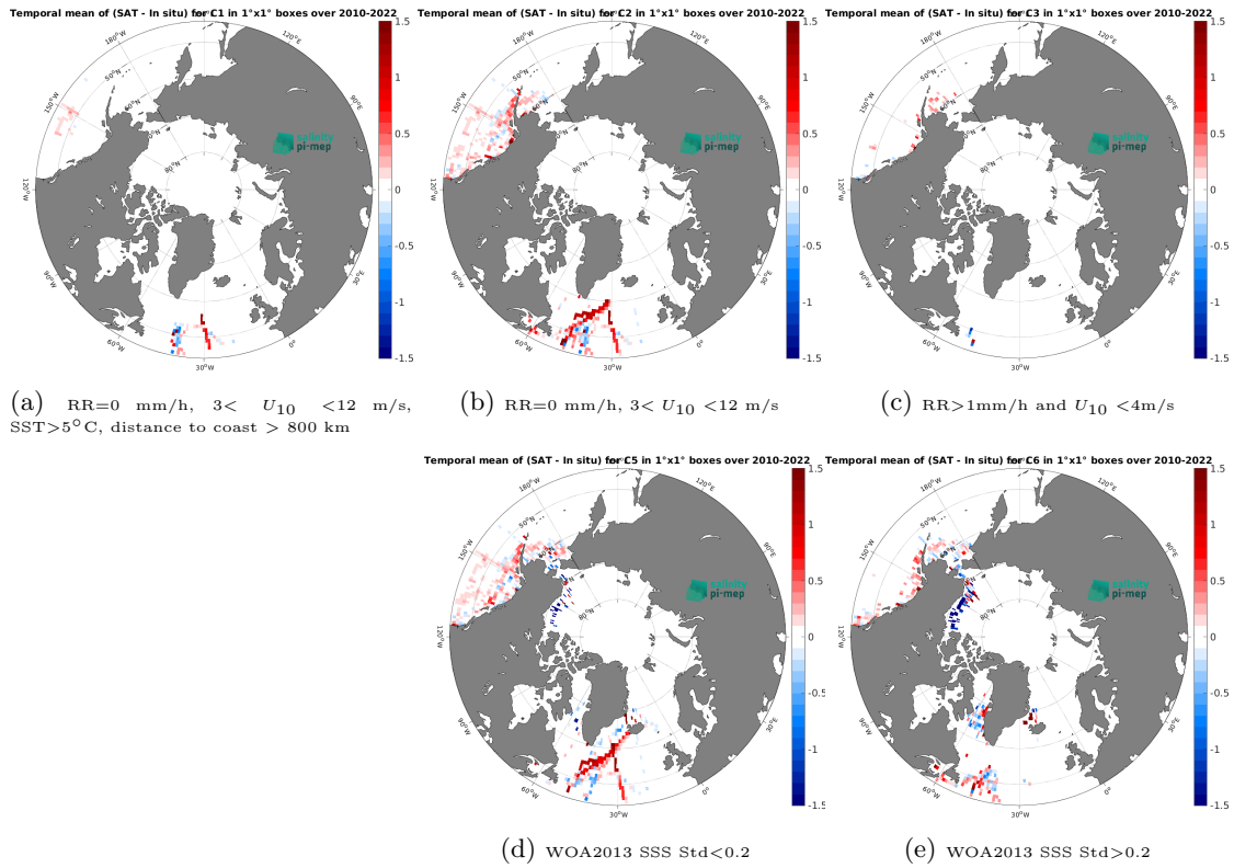
Figure 12: Temporal mean gridded over spatial boxes of size 1^{\circ}\times 1^{\circ} of \Delta\text{SSS} (CCI SSS L4 POLAR NH Merged-OI v4.4 - 30-day running (ESA) - TSG (SAMOS)) for 5 different subdatasets corresponding to:RR=0 mm/h, 3 < U_{10} < 12 m/s, SST > 5^{\circ}\text{C} , distance to coast > 800 km (a), RR=0 mm/h, 3 < U_{10} < 12 m/s (b), RR > 1 mm/h and U_{10} < 4 m/s (c), WOA2013 SSS Std < 0.2 (d), WOA2013 SSS Std > 0.2 (e).
