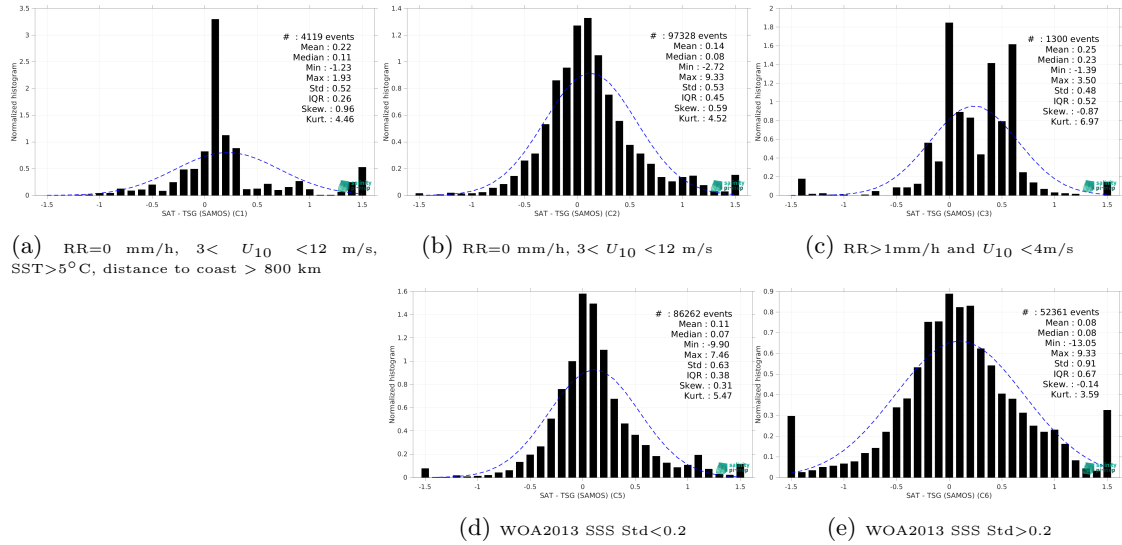
Figure 13: Normalized histogram of \Delta SSS (CCI SSS L4 POLAR NH Merged-OI v4.4 - 30-day running (ESA) - TSG (SAMOS)) for 5 different subdatasets corresponding to: RR=0 mm/h, 3 < U_{10} < 12 m/s, SST>5°C, distance to coast > 800 km (a), RR=0 mm/h, 3 < U_{10} < 12 m/s (b), RR>1mm/h and U_{10} < 4 m/s (c), WOA2013 SSS Std<0.2 (d), WOA2013 SSS Std>0.2 (e).
