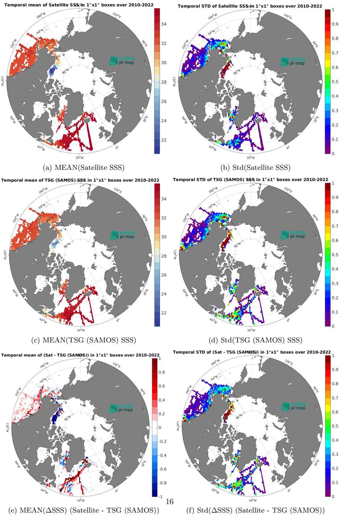
Figure 6: Temporal mean (left) and Std (right) of SSS from CCI SSS L4 POLAR NH Merged-OI v4.4 - 30-day running (ESA) (top), TSG (SAMOS) (middle), and of \Delta SSS (Satellite - TSG (SAMOS)). Only match-up pairs are used to generate these maps.
