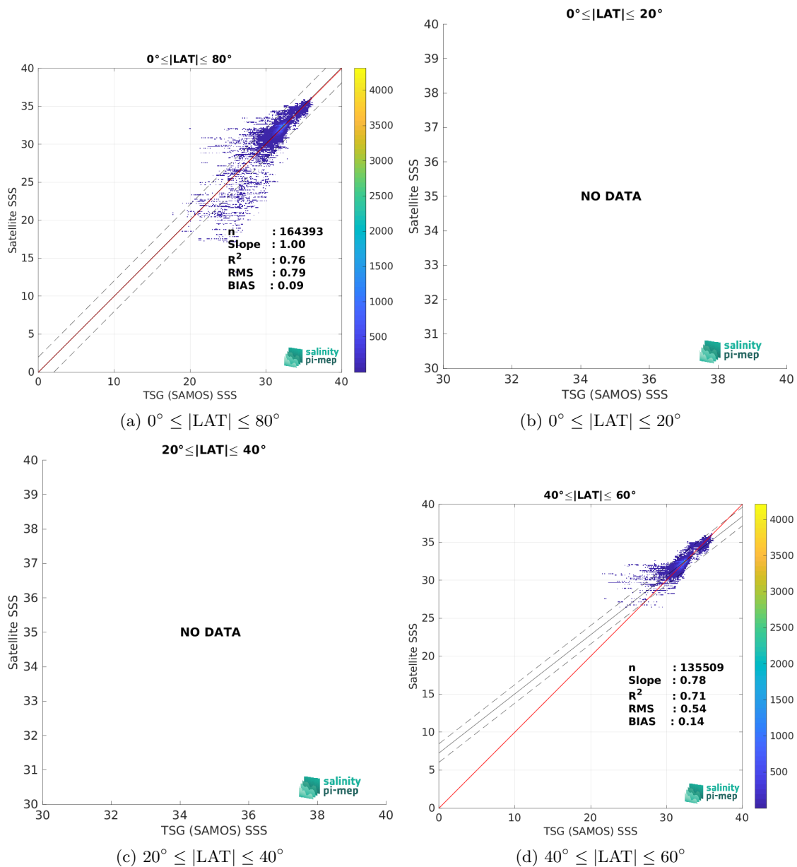
Figure 9: Contour maps of the concentration of CCI SSS L4 POLAR NH Merged-OI v4.4 - 30-day running (ESA) SSS (y-axis) versus TSG (SAMOS) SSS (x-axis) at match-up pairs for different latitude bands. For each plot, the red line shows x=y . The black thin and dashed lines indicate a linear fit through the data cloud and the \pm 95\% confidence levels, respectively. The number match-up pairs n , the slope and R^2 coefficient of the linear fit, the root mean square (RMS) and the mean bias between satellite and in situ data are indicated for each latitude band in each plots.
