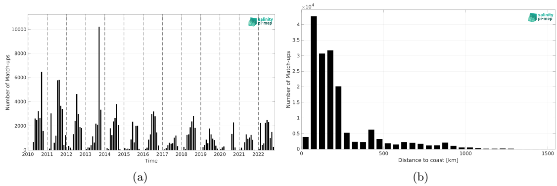
Figure 1: Number of match-ups between TSG (SAMOS) and CCI SSS L4 POLAR NH Merged-OI v4.4 - 30-day running (ESA) SSS as a function of time (a) and as function of the distance to coast (b) over the Global Ocean Pi-MEP region and for the full satellite product period.
