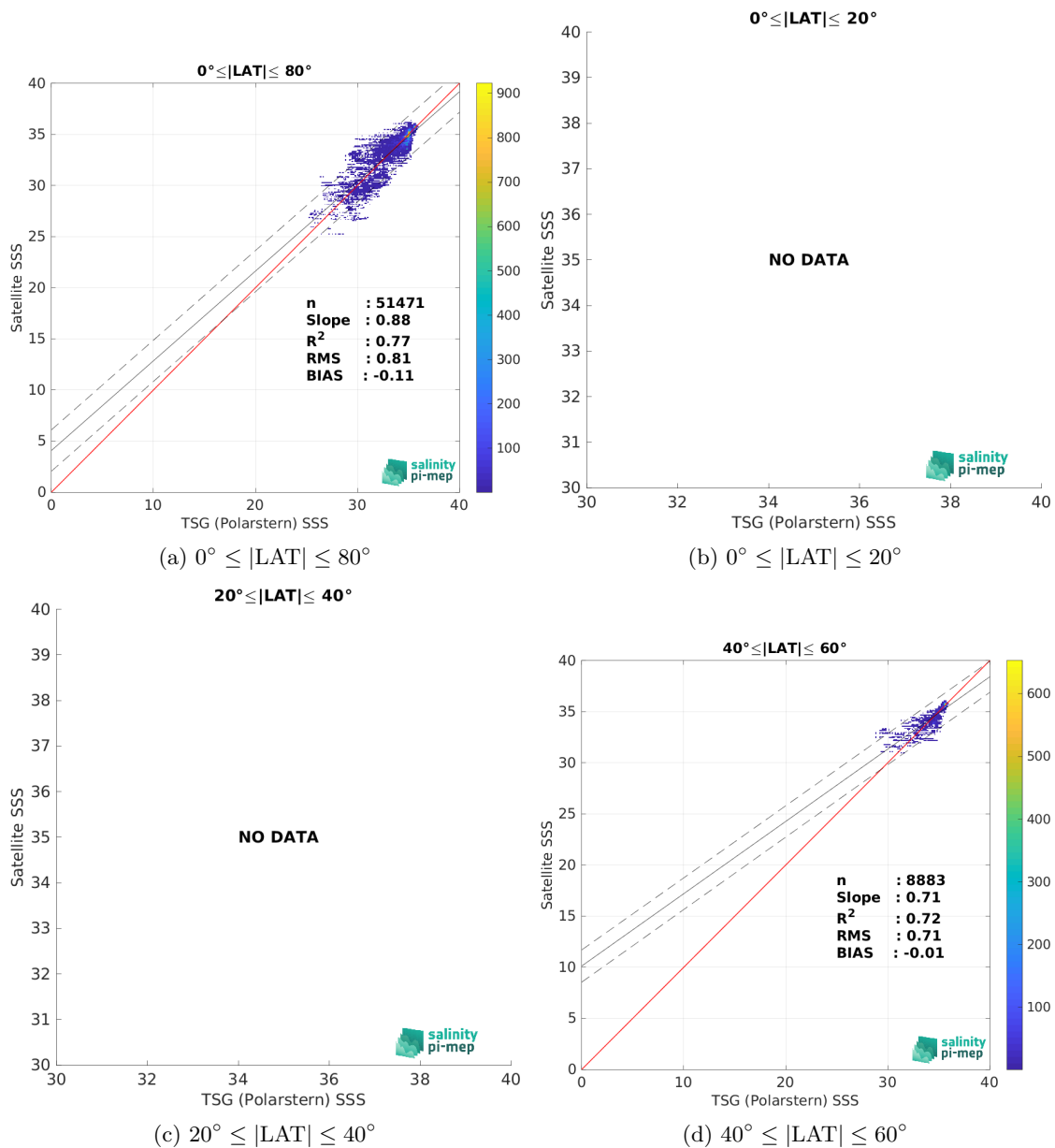
Figure 9: Contour maps of the concentration of CCI SSS L4 POLAR NH Merged-OI v4.4 - 30-day running (ESA) SSS (y-axis) versus TSG (Polarstern) SSS (x-axis) at match-up pairs for different latitude bands. For each plot, the red line shows x=y . The black thin and dashed lines indicate a linear fit through the data cloud and the \pm 95\% confidence levels, respectively. The number match-up pairs n , the slope and R^2 coefficient of the linear fit, the root mean square (RMS) and the mean bias between satellite and in situ data are indicated for each latitude band in each plots.
