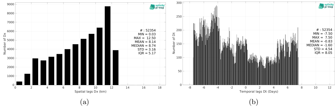
Figure 5: Histograms of the spatial (a) and temporal (b) lags between the location/time of the TSG (Polarstern) measurement and the date of the corresponding CCI SSS L4 POLAR NH Merged-OI v4.4 - 30-day running (ESA) SSS pixel.
