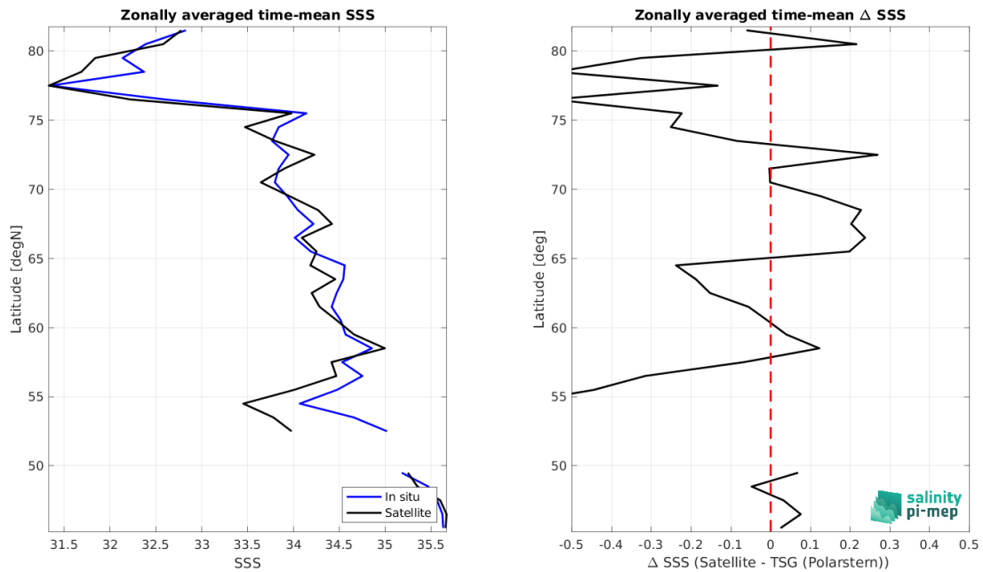
Figure 8: Left panel: Zonal mean SSS from CCI SSS L4 POLAR NH Merged-OI v4.4 - 30-day running (ESA) satellite product (black) and from TSG (Polarstern) (blue). Right panel: Zonal mean of \Delta SSS (Satellite - TSG (Polarstern)) for all the collected Pi-MEP match-up pairs estimated over the full satellite product period.
