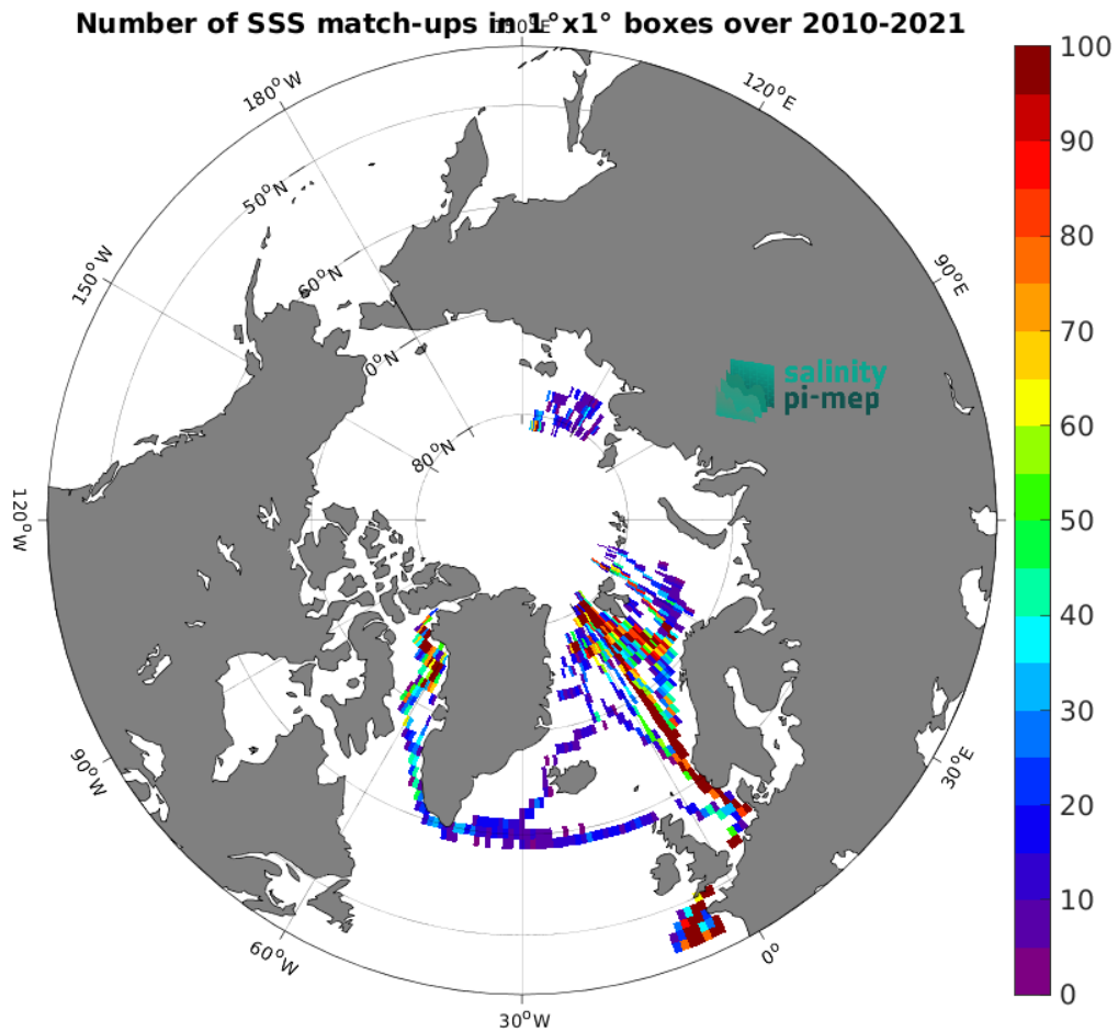
Figure 4: Number of SSS match-ups between TSG (Polarstern) SSS and the CCI SSS L4 POLAR NH Merged-OI v4.4 - 30-day running (ESA) SSS product for the Global Ocean Pi-MEP region over 1^{\circ} \times 1^{\circ} boxes and for the full satellite product period.
