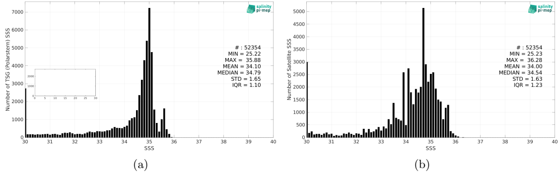
Figure 2: Histograms of SSS from TSG (Polarstern) (a) and CCI SSS L4 POLAR NH Merged-OI v4.4 - 30-day running (ESA) (b) considering all match-up pairs per bins of 0.1 over the Global Ocean Pi-MEP region and for the full satellite product period.
