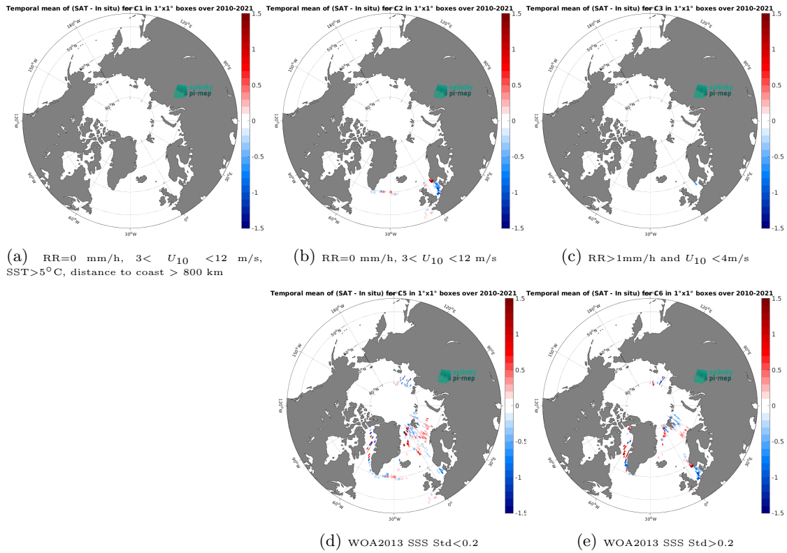
Figure 12: Temporal mean gridded over spatial boxes of size 1^{\circ}\times 1^{\circ} of \Delta\text{SSS} (CCI SSS L4 POLAR NH Merged-OI v4.4 - 30-day running (ESA) - TSG (Polarstern)) for 5 different subdatasets corresponding to:RR=0 mm/h, 3 < U_{10} < 12 m/s, SST > 5^{\circ}\text{C} , distance to coast > 800 km (a), RR=0 mm/h, 3 < U_{10} < 12 m/s (b), RR > 1 mm/h and U_{10} < 4 m/s (c), WOA2013 SSS Std < 0.2 (d), WOA2013 SSS Std > 0.2 (e).
