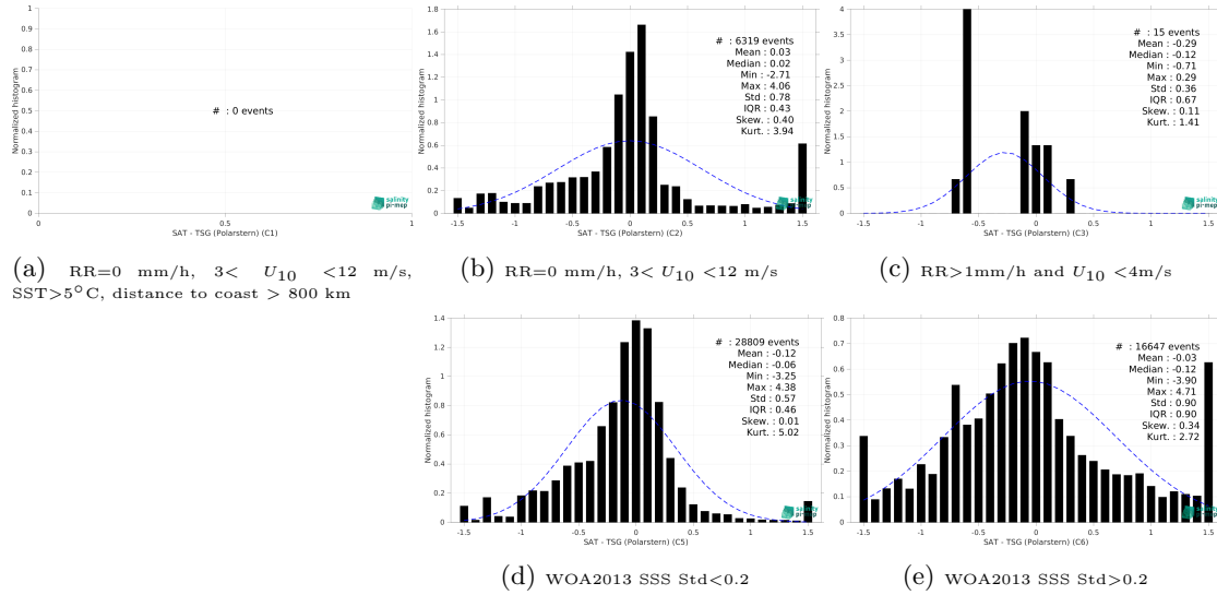
Figure 13: Normalized histogram of \Delta SSS (CCI SSS L4 POLAR NH Merged-OI v4.4 - 30-day running (ESA) - TSG (Polarstern)) for 5 different subdatasets corresponding to: RR=0 mm/h, 3 < U_{10} < 12 m/s, SST > 5°C, distance to coast > 800 km (a), RR=0 mm/h, 3 < U_{10} < 12 m/s (b), RR > 1mm/h and U_{10} < 4 m/s (c), WOA2013 SSS Std < 0.2 (d), WOA2013 SSS Std > 0.2 (e).
