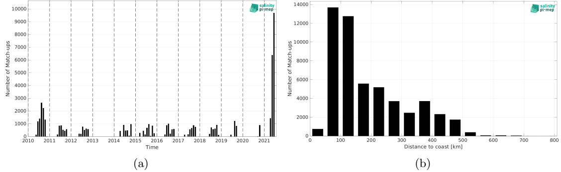
Figure 1: Number of match-ups between TSG (Polarstern) and CCI SSS L4 POLAR NH Merged-OI v4.4 - 30-day running (ESA) SSS as a function of time (a) and as function of the distance to coast (b) over the Global Ocean Pi-MEP region and for the full satellite product period.
