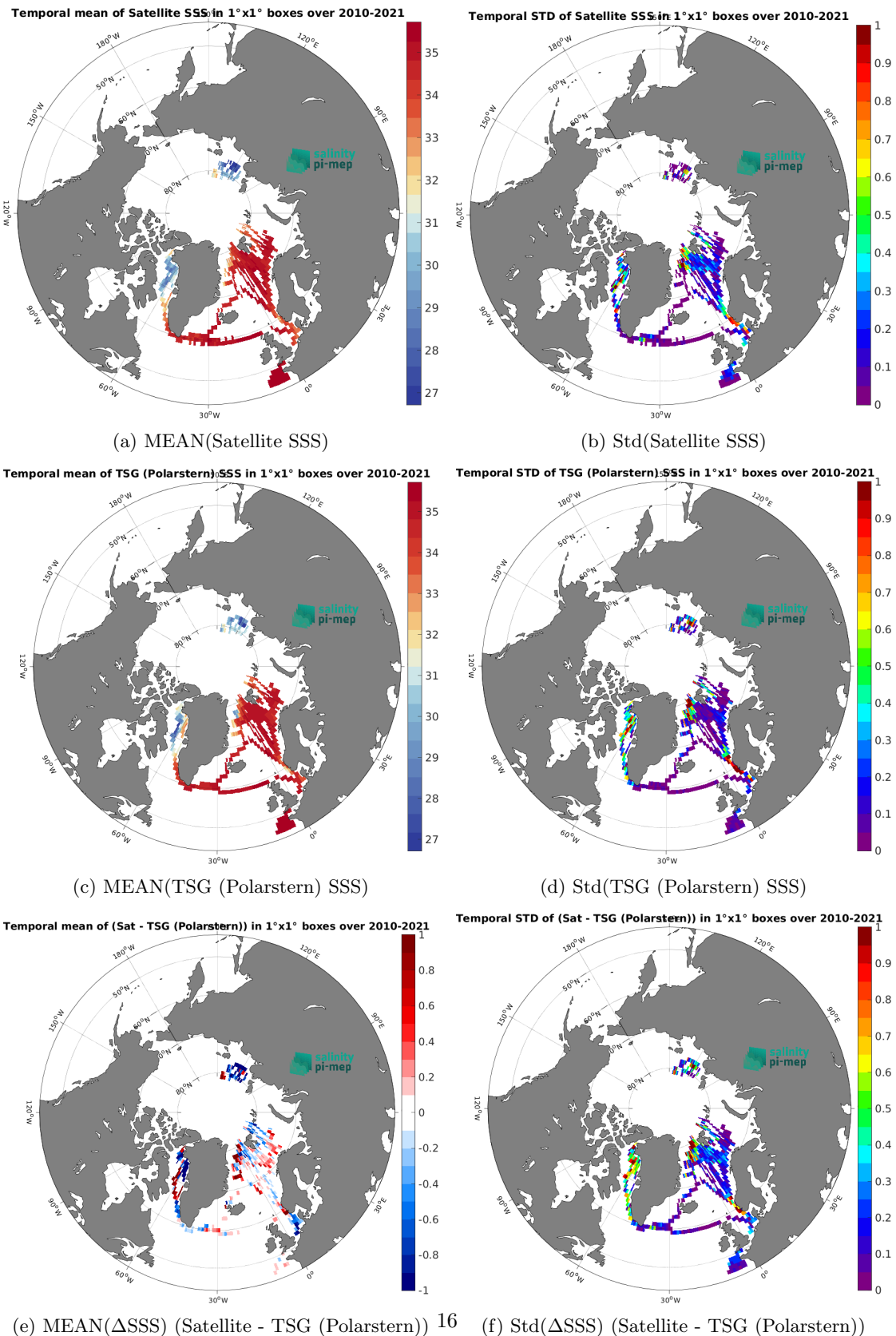
Figure 6: Temporal mean (left) and Std (right) of SSS from CCI SSS L4 POLAR NH Merged-OI v4.4 - 30-day running (ESA) (top), TSG (Polarstern) (middle), and of \Delta SSS (Satellite - TSG (Polarstern)). Only match-up pairs are used to generate these maps.
