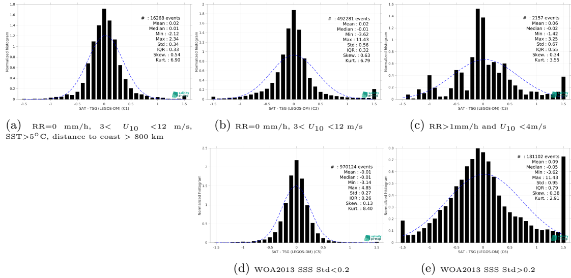
Figure 13: Normalized histogram of \Delta SSS (CCI SSS L4 POLAR NH Merged-OI v4.4 - 30-day running (ESA) - TSG (LEGOS-DM)) for 5 different subdatasets corresponding to: RR=0 mm/h, 3 < U_{10} < 12 m/s, SST>5°C, distance to coast > 800 km (a), RR=0 mm/h, 3 < U_{10} < 12 m/s (b), RR>1mm/h and U_{10} < 4 m/s (c), WOA2013 SSS Std<0.2 (d), WOA2013 SSS Std>0.2 (e).
