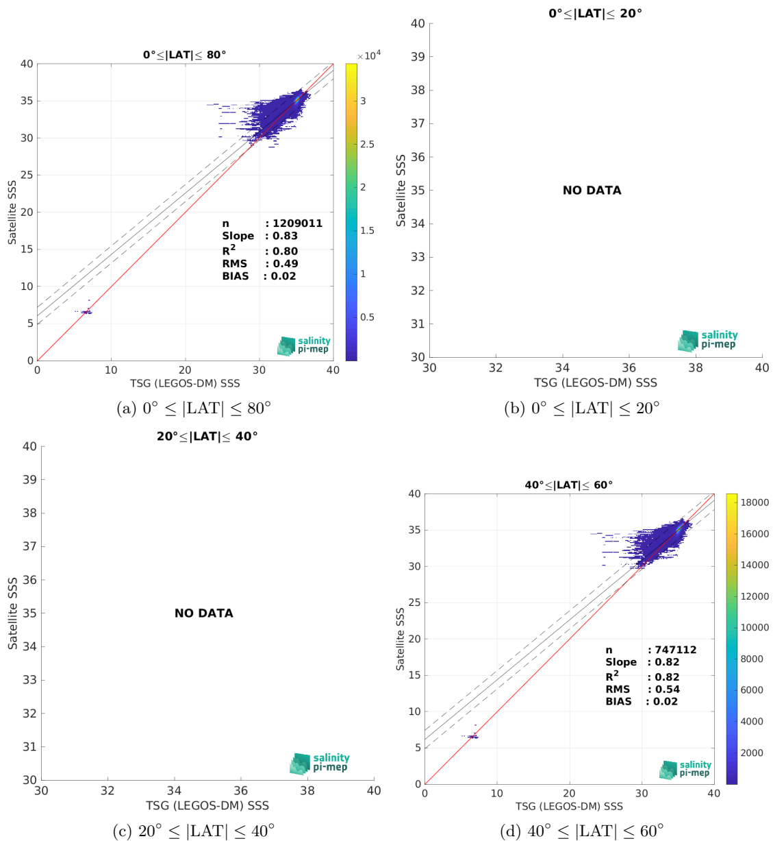
Figure 9: Contour maps of the concentration of CCI SSS L4 POLAR NH Merged-OI v4.4 - 30-day running (ESA) SSS (y-axis) versus TSG (LEGOS-DM) SSS (x-axis) at match-up pairs for different latitude bands. For each plot, the red line shows x=y . The black thin and dashed lines indicate a linear fit through the data cloud and the \pm 95\% confidence levels, respectively. The number match-up pairs n , the slope and R^2 coefficient of the linear fit, the root mean square (RMS) and the mean bias between satellite and in situ data are indicated for each latitude band in each plots.
