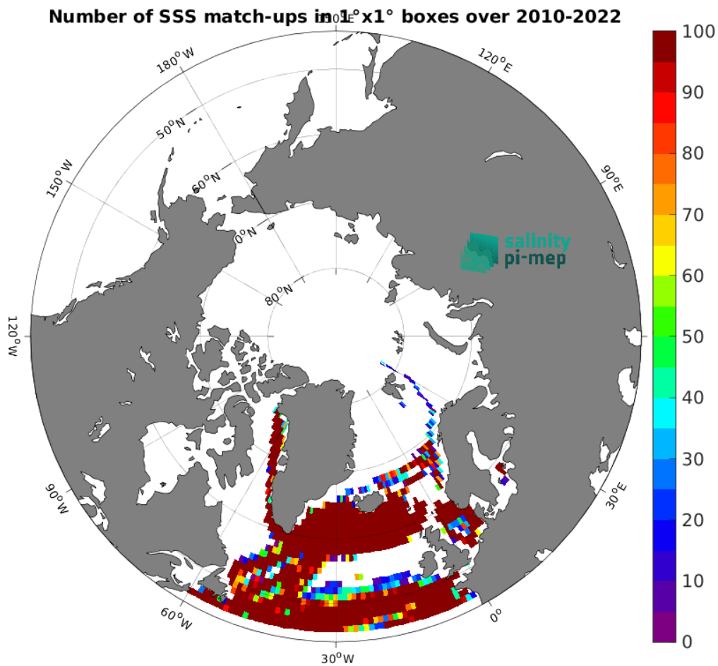
Figure 4: Number of SSS match-ups between TSG (LEGOS-DM) SSS and the CCI SSS L4 POLAR NH Merged-OI v4.4 - 30-day running (ESA) SSS product for the Global Ocean Pi-MEP region over 1^{\circ} \times 1^{\circ} boxes and for the full satellite product period.
