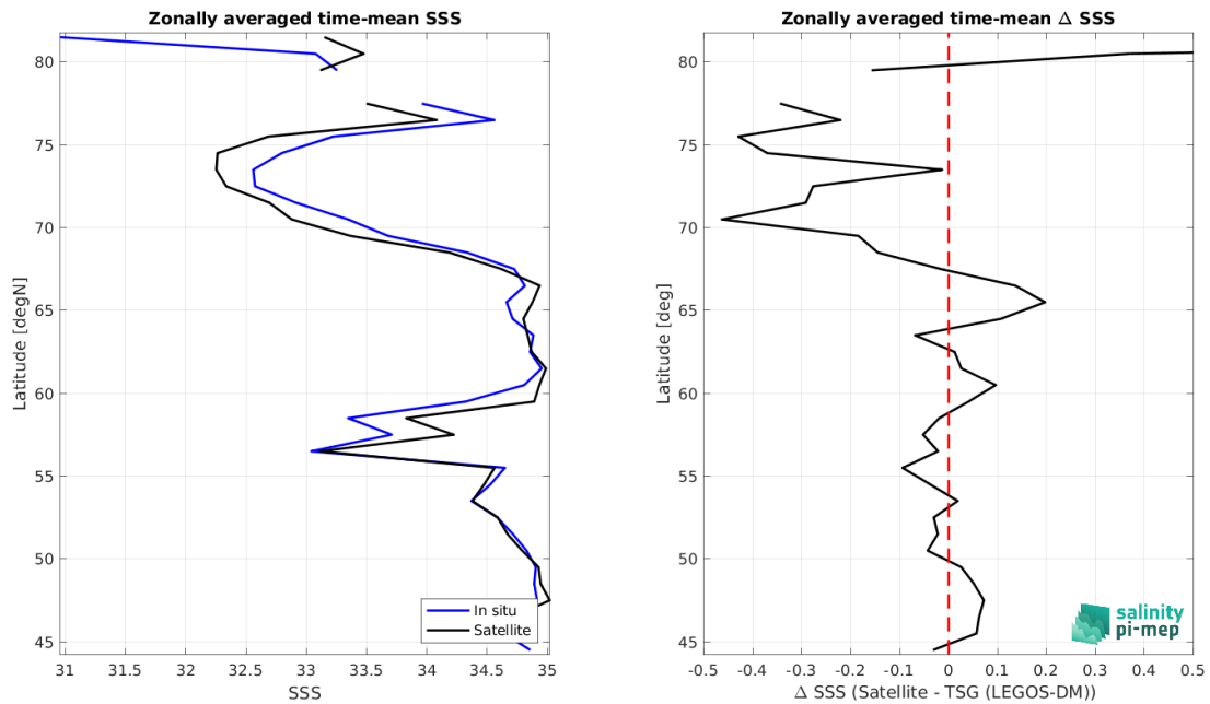
Figure 8: Left panel: Zonal mean SSS from CCI SSS L4 POLAR NH Merged-OI v4.4 - 30-day running (ESA) satellite product (black) and from TSG (LEGOS-DM) (blue). Right panel: Zonal mean of \Delta SSS (Satellite - TSG (LEGOS-DM)) for all the collected Pi-MEP match-up pairs estimated over the full satellite product period.
