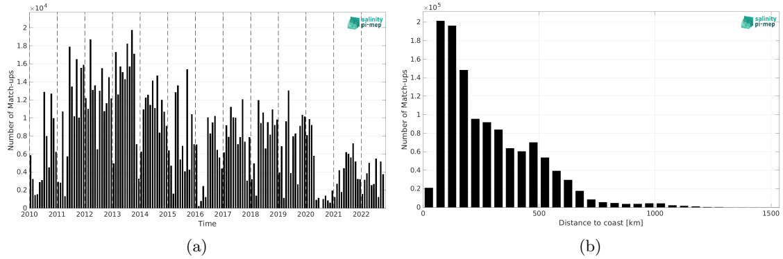
Figure 1: Number of match-ups between TSG (LEGOS-DM) and CCI SSS L4 POLAR NH Merged-OI v4.4 - 30-day running (ESA) SSS as a function of time (a) and as function of the distance to coast (b) over the Global Ocean Pi-MEP region and for the full satellite product period.
