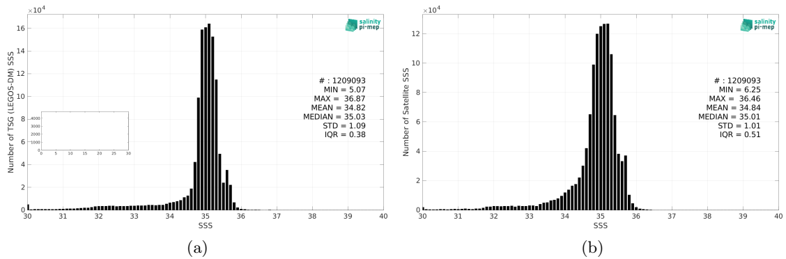
Figure 2: Histograms of SSS from TSG (LEGOS-DM) (a) and CCI SSS L4 POLAR NH Merged-OI v4.4 - 30-day running (ESA) (b) considering all match-up pairs per bins of 0.1 over the Global Ocean Pi-MEP region and for the full satellite product period.
