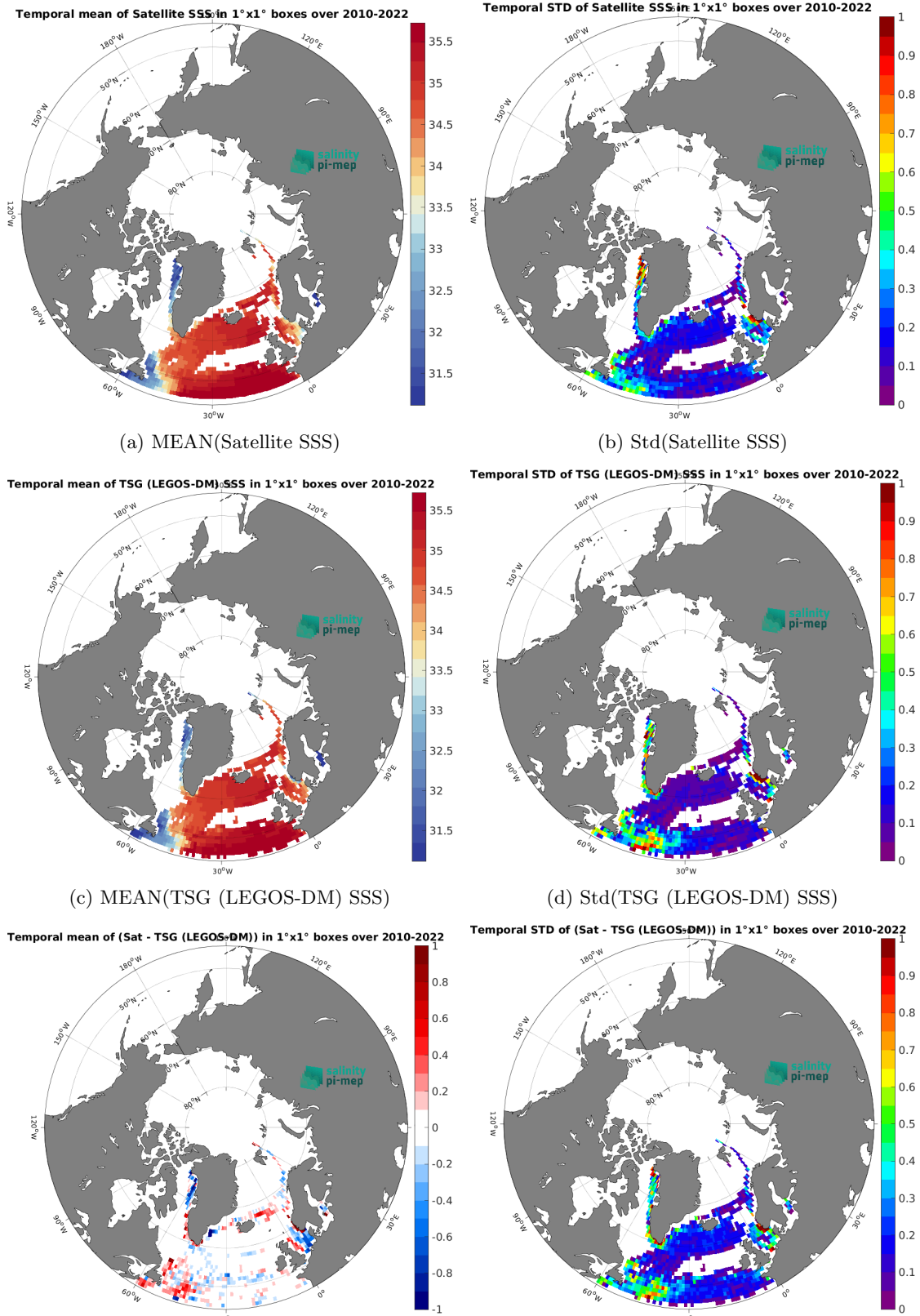
Figure 6: Temporal mean (left) and Std (right) of SSS from CCI SSS L4 POLAR NH Merged-OI v4.4 - 30-day running (ESA) (top), TSG (LEGOS-DM) (middle), and of \Delta SSS (Satellite - TSG (LEGOS-DM)). Only match-up pairs are used to generate these maps.
