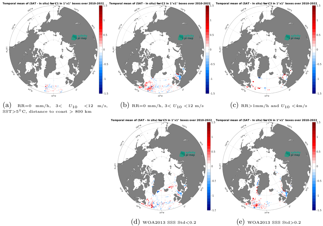
Figure 12: Temporal mean gridded over spatial boxes of size 1^{\circ}\times 1^{\circ} of \Delta\text{SSS} (CCI SSS L4 POLAR NH Merged-OI v4.4 - 30-day running (ESA) - TSG (LEGOS-DM)) for 5 different subdatasets corresponding to:RR=0 mm/h, 3 < U_{10} < 12 m/s, SST >5^{\circ}\text{C} , distance to coast > 800 km (a), RR=0 mm/h, 3 < U_{10} < 12 m/s (b), RR >1 mm/h and U_{10} < 4 m/s (c), WOA2013 SSS Std <0.2 (d), WOA2013 SSS Std >0.2 (e).
