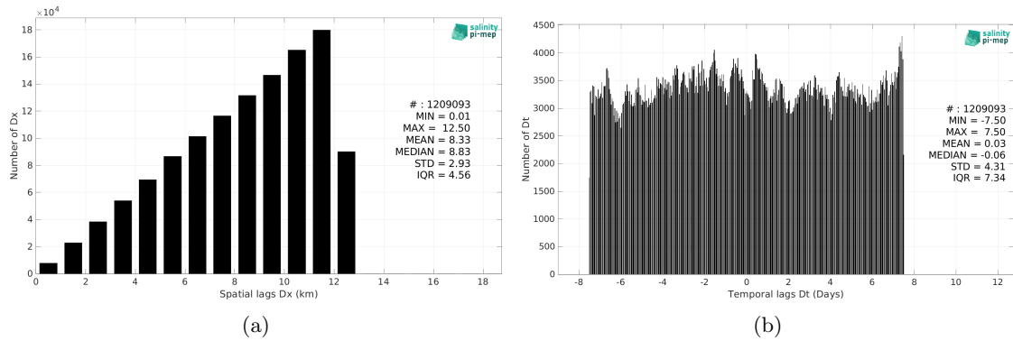
Figure 5: Histograms of the spatial (a) and temporal (b) lags between the location/time of the TSG (LEGOS-DM) measurement and the date of the corresponding CCI SSS L4 POLAR NH Merged-OI v4.4 - 30-day running (ESA) SSS pixel.
