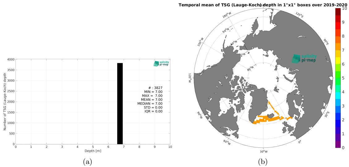
Figure 3: Histograms of the depth of the upper level SSS measurements from TSG (Lauge-Koch) in the Match-up DataBase for the Global Ocean Pi-MEP region (a) and temporal mean spatial distribution of pressure of the in situ SSS data over 1^\circ \times 1^\circ boxes and for the full satellite product period (b).
