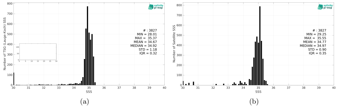
Figure 2: Histograms of SSS from TSG (Lauge-Koch) (a) and CCI SSS L4 POLAR NH Merged-OI v4.4 - 30-day running (ESA) (b) considering all match-up pairs per bins of 0.1 over the Global Ocean Pi-MEP region and for the full satellite product period.
