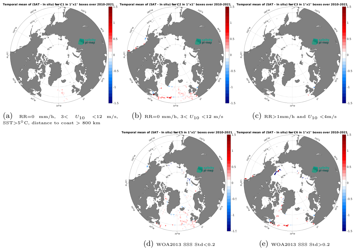
Figure 12: Temporal mean gridded over spatial boxes of size 1^\circ \times 1^\circ of \Delta SSS (CCI SSS L4 POLAR NH Merged-OI v4.4 - 30-day running (ESA) - TSG (GOSUD-Sailing-ship)) for 5 different subdatasets corresponding to: RR=0 mm/h, 3 < U_{10} < 12 m/s, SST>5°C, distance to coast > 800 km (a), RR=0 mm/h, 3 < U_{10} < 12 m/s (b), RR>1mm/h and U_{10} < 4 m/s (c), WOA2013 SSS Std<0.2 (d), WOA2013 SSS Std>0.2 (e).
