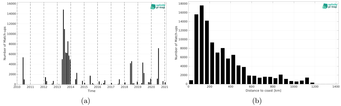
Figure 1: Number of match-ups between TSG (GOSUD-Sailing-ship) and CCI SSS L4 POLAR NH Merged-OI v4.4 - 30-day running (ESA) SSS as a function of time (a) and as function of the distance to coast (b) over the Global Ocean Pi-MEP region and for the full satellite product period.
