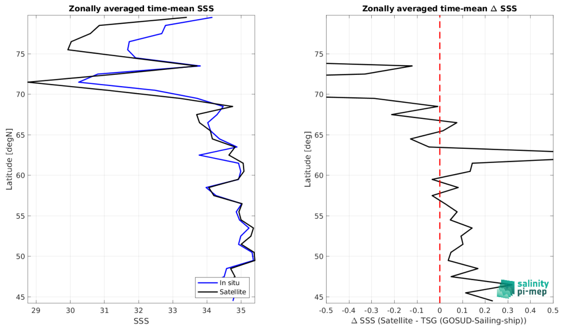
Figure 8: Left panel: Zonal mean SSS from CCI SSS L4 POLAR NH Merged-OI v4.4 - 30-day running (ESA) satellite product (black) and from TSG (GOSUD-Sailing-ship) (blue). Right panel: Zonal mean of \Delta SSS (Satellite - TSG (GOSUD-Sailing-ship)) for all the collected Pi-MEP match-up pairs estimated over the full satellite product period.
