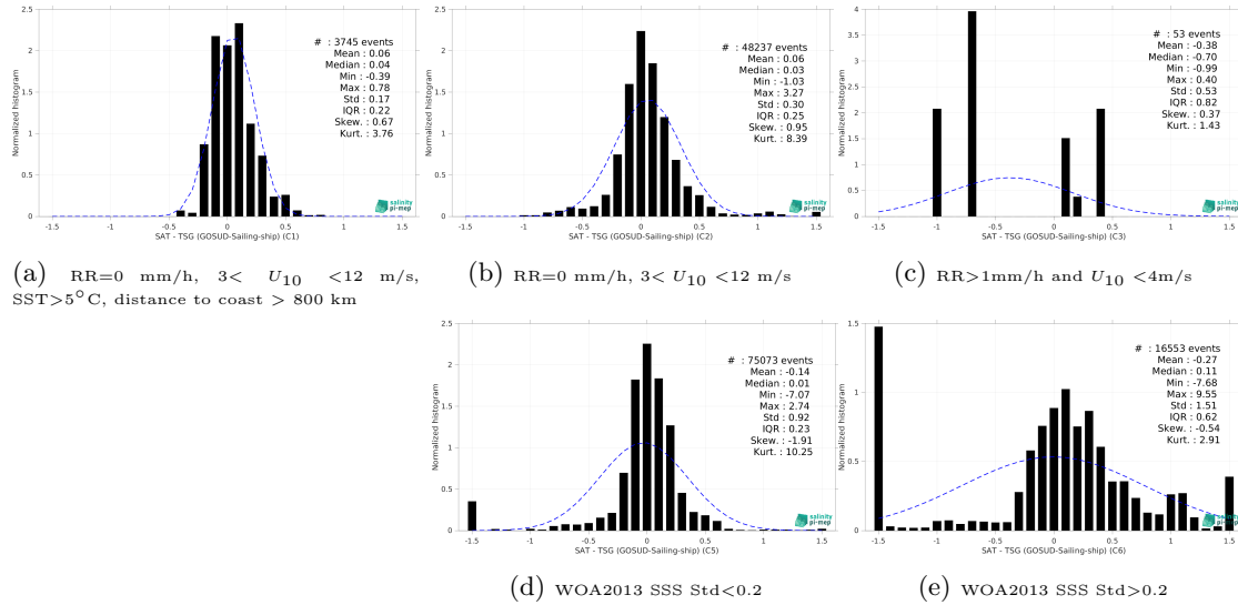
Figure 13: Normalized histogram of \Delta SSS (CCI SSS L4 POLAR NH Merged-OI v4.4 - 30-day running (ESA) - TSG (GOSUD-Sailing-ship)) for 5 different subdatasets corresponding to: RR=0 mm/h, 3 < U_{10} < 12 m/s, SST >5^{\circ} C, distance to coast > 800 km (a), RR=0 mm/h, 3 < U_{10} < 12 m/s (b), RR >1 mm/h and U_{10} < 4 m/s (c), WOA2013 SSS Std <0.2 (d), WOA2013 SSS Std >0.2 (e).
