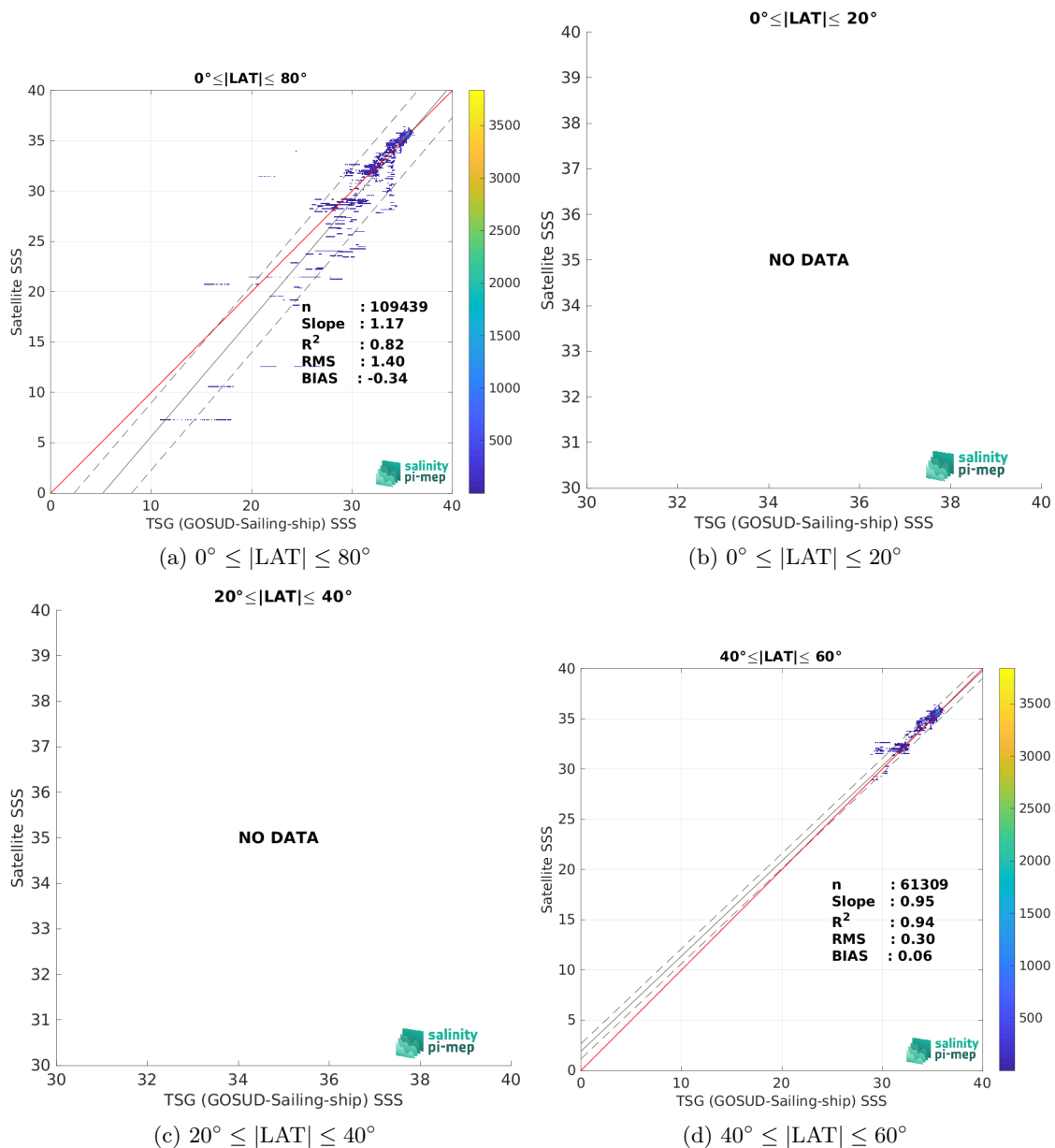
Figure 9: Contour maps of the concentration of CCI SSS L4 POLAR NH Merged-OI v4.4 - 30-day running (ESA) SSS (y-axis) versus TSG (GOSUD-Sailing-ship) SSS (x-axis) at match-up pairs for different latitude bands. For each plot, the red line shows x=y . The black thin and dashed lines indicate a linear fit through the data cloud and the \pm 95\% confidence levels, respectively. The number match-up pairs n , the slope and R^2 coefficient of the linear fit, the root mean square (RMS) and the mean bias between satellite and in situ data are indicated for each latitude band in each plots.
