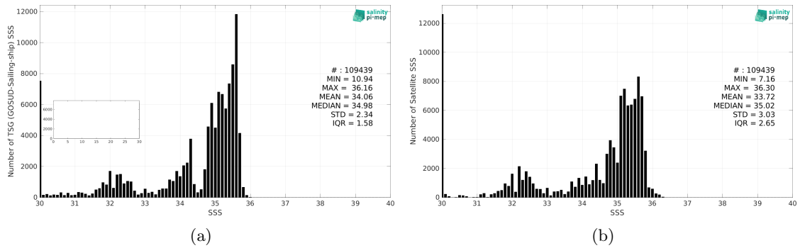
Figure 2: Histograms of SSS from TSG (GOSUD-Sailing-ship) (a) and CCI SSS L4 POLAR NH Merged-OI v4.4 - 30-day running (ESA) (b) considering all match-up pairs per bins of 0.1 over the Global Ocean Pi-MEP region and for the full satellite product period.
