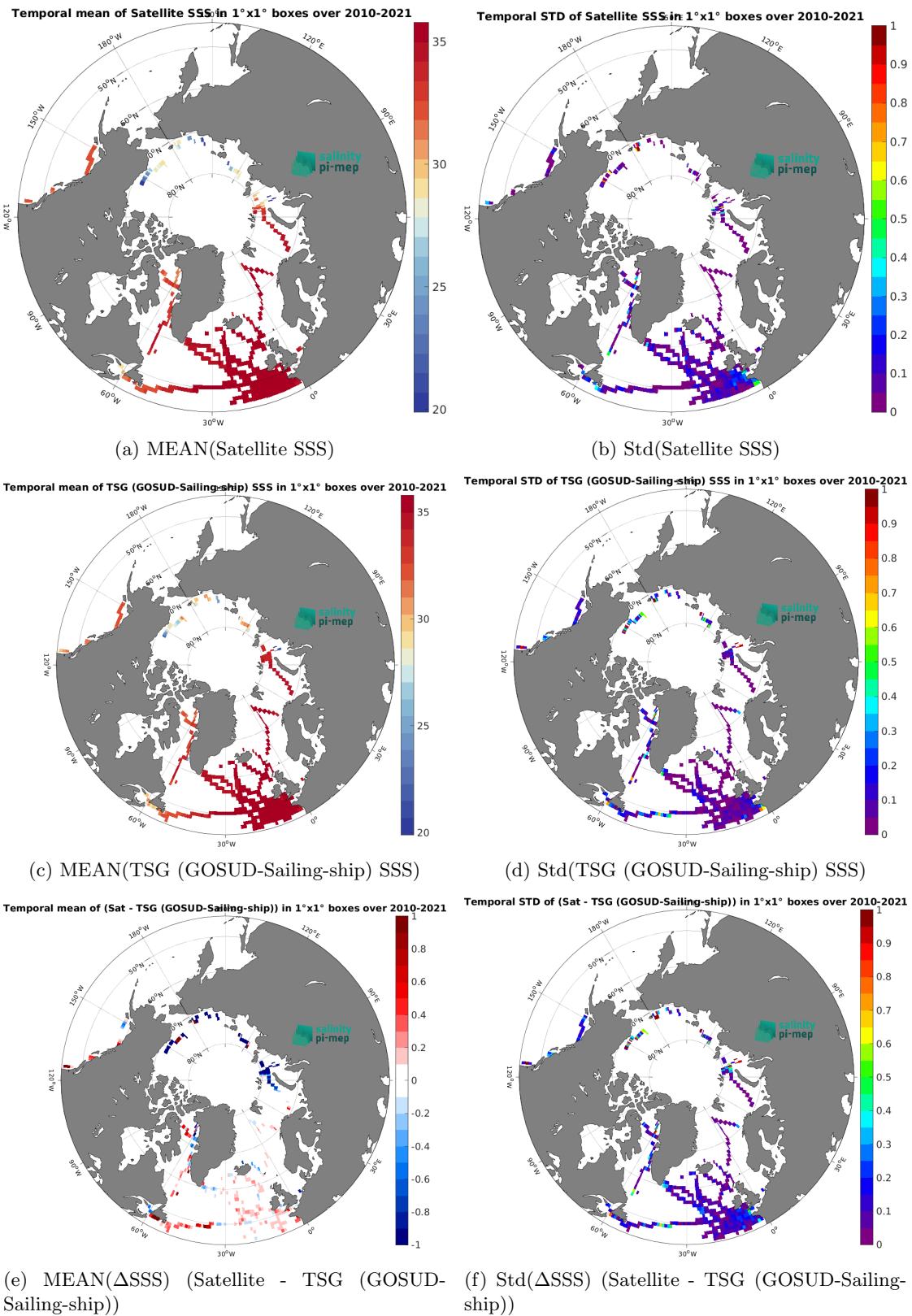
Figure 6: Temporal mean (left) and Std (right) of SSS from CCI SSS L4 POLAR NH Merged-OI v4.4 - 30-day running (ESA) (top), TSG (GOSUD-Sailing-ship) (middle), and of \Delta SSS (Satellite - TSG (GOSUD-Sailing-ship)). Only match-up pairs are used to generate these maps.
