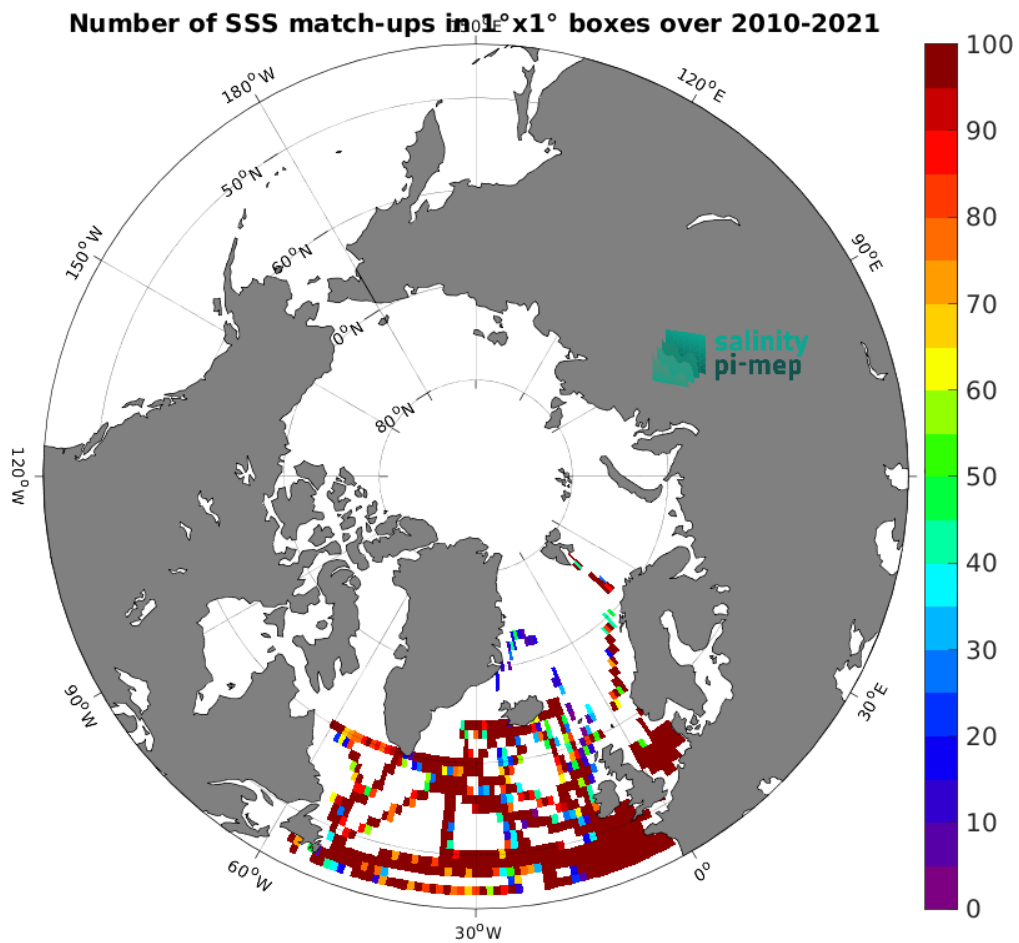
Figure 4: Number of SSS match-ups between TSG (GOSUD-Research-vessel) SSS and the CCI SSS L4 POLAR NH Merged-OI v4.4 - 30-day running (ESA) SSS product for the Global Ocean Pi-MEP region over 1^{\circ} \times 1^{\circ} boxes and for the full satellite product period.
