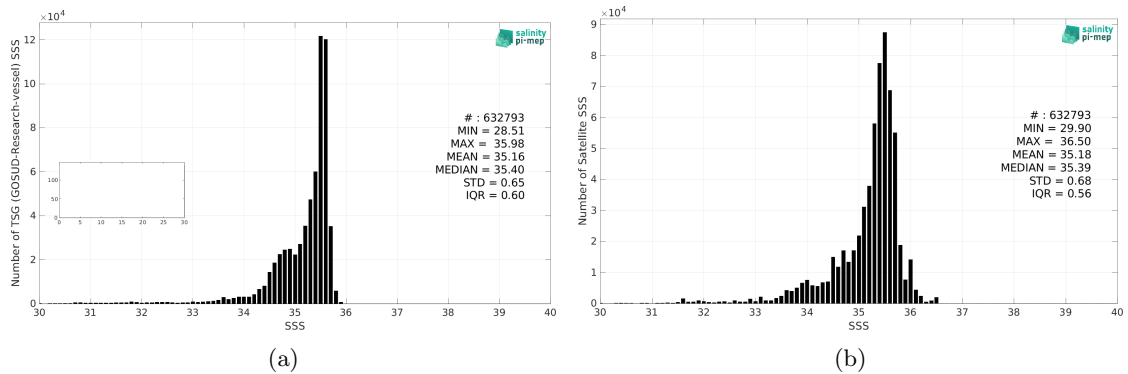
Figure 2: Histograms of SSS from TSG (GOSUD-Research-vessel) (a) and CCI SSS L4 POLAR NH Merged-OI v4.4 - 30-day running (ESA) (b) considering all match-up pairs per bins of 0.1 over the Global Ocean Pi-MEP region and for the full satellite product period.
