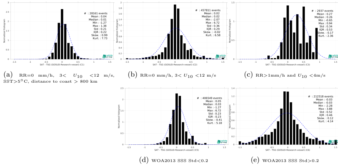
Figure 13: Normalized histogram of \Delta SSS (CCI SSS L4 POLAR NH Merged-OI v4.4 - 30-day running (ESA) - TSG (GOSUD-Research-vessel)) for 5 different subdatasets corresponding to: RR=0 mm/h, 3 < U_{10} < 12 m/s, SST>5°C, distance to coast > 800 km (a), RR=0 mm/h, 3 < U_{10} < 12 m/s (b), RR>1mm/h and U_{10} < 4 m/s (c), WOA2013 SSS Std<0.2 (d), WOA2013 SSS Std>0.2 (e).
