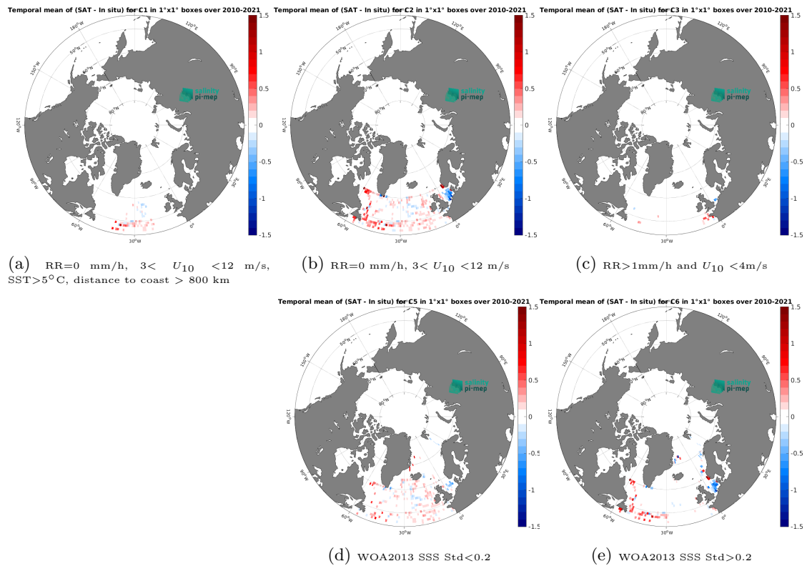
Figure 12: Temporal mean gridded over spatial boxes of size 1^\circ \times 1^\circ of \Delta SSS (CCI SSS L4 POLAR NH Merged-OI v4.4 - 30-day running (ESA) - TSG (GOSUD-Research-vessel)) for 5 different subdatasets corresponding to: RR=0 mm/h, 3 < U_{10} < 12 m/s, SST > 5°C, distance to coast > 800 km (a), RR=0 mm/h, 3 < U_{10} < 12 m/s (b), RR > 1mm/h and U_{10} < 4 m/s (c), WOA2013 SSS Std < 0.2 (d), WOA2013 SSS Std > 0.2 (e).
