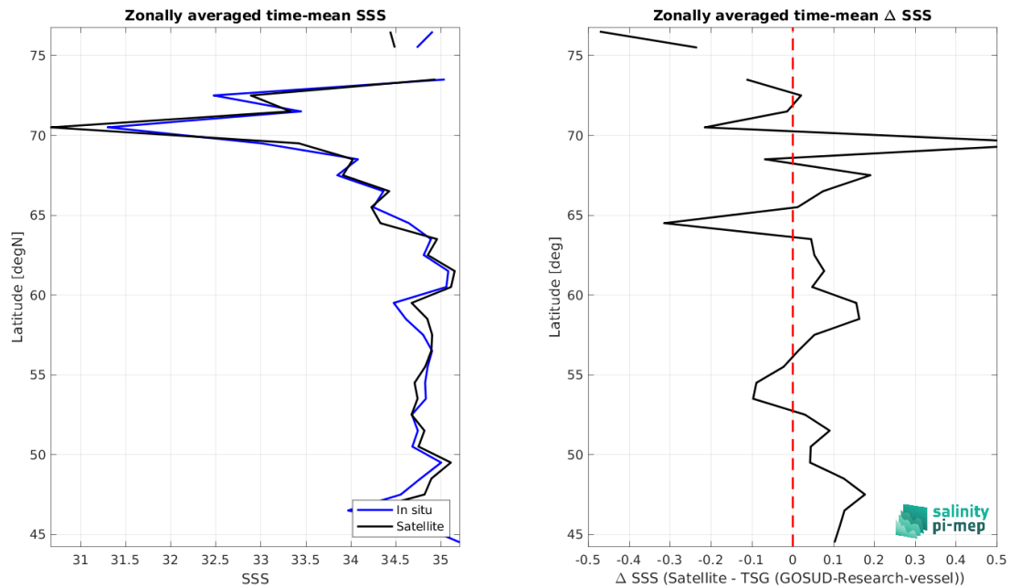
Figure 8: Left panel: Zonal mean SSS from CCI SSS L4 POLAR NH Merged-OI v4.4 - 30-day running (ESA) satellite product (black) and from TSG (GOSUD-Research-vessel) (blue). Right panel: Zonal mean of \Delta SSS (Satellite - TSG (GOSUD-Research-vessel)) for all the collected Pi-MEP match-up pairs estimated over the full satellite product period.
