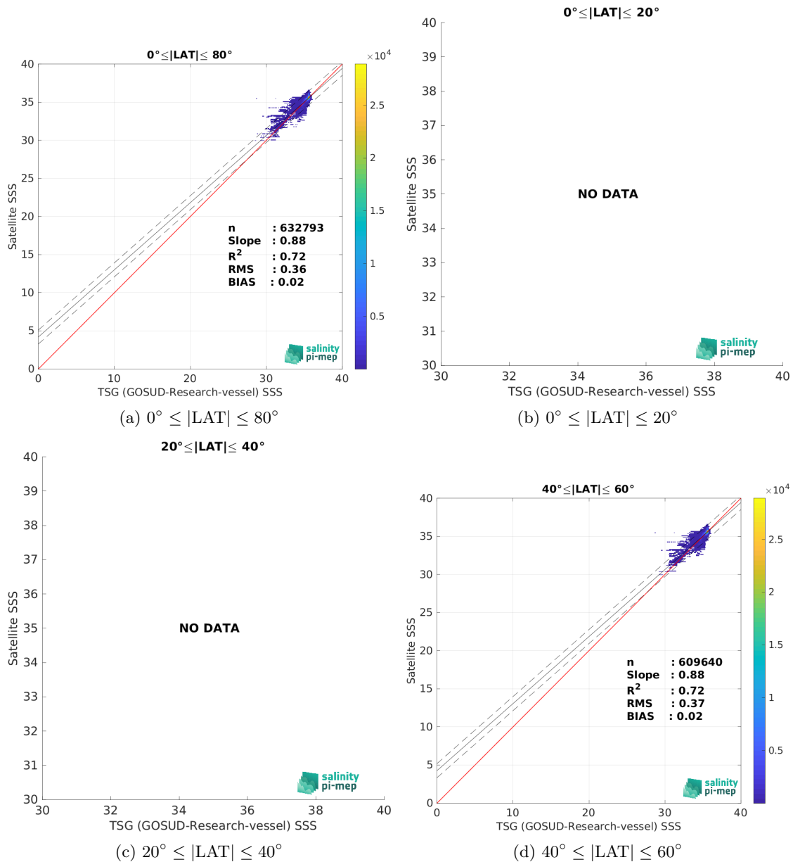
Figure 9: Contour maps of the concentration of CCI SSS L4 POLAR NH Merged-OI v4.4 - 30-day running (ESA) SSS (y-axis) versus TSG (GOSUD-Research-vessel) SSS (x-axis) at match-up pairs for different latitude bands. For each plot, the red line shows x=y . The black thin and dashed lines indicate a linear fit through the data cloud and the \pm 95\% confidence levels, respectively. The number match-up pairs n , the slope and R^2 coefficient of the linear fit, the root mean square (RMS) and the mean bias between satellite and in situ data are indicated for each latitude band in each plots.
