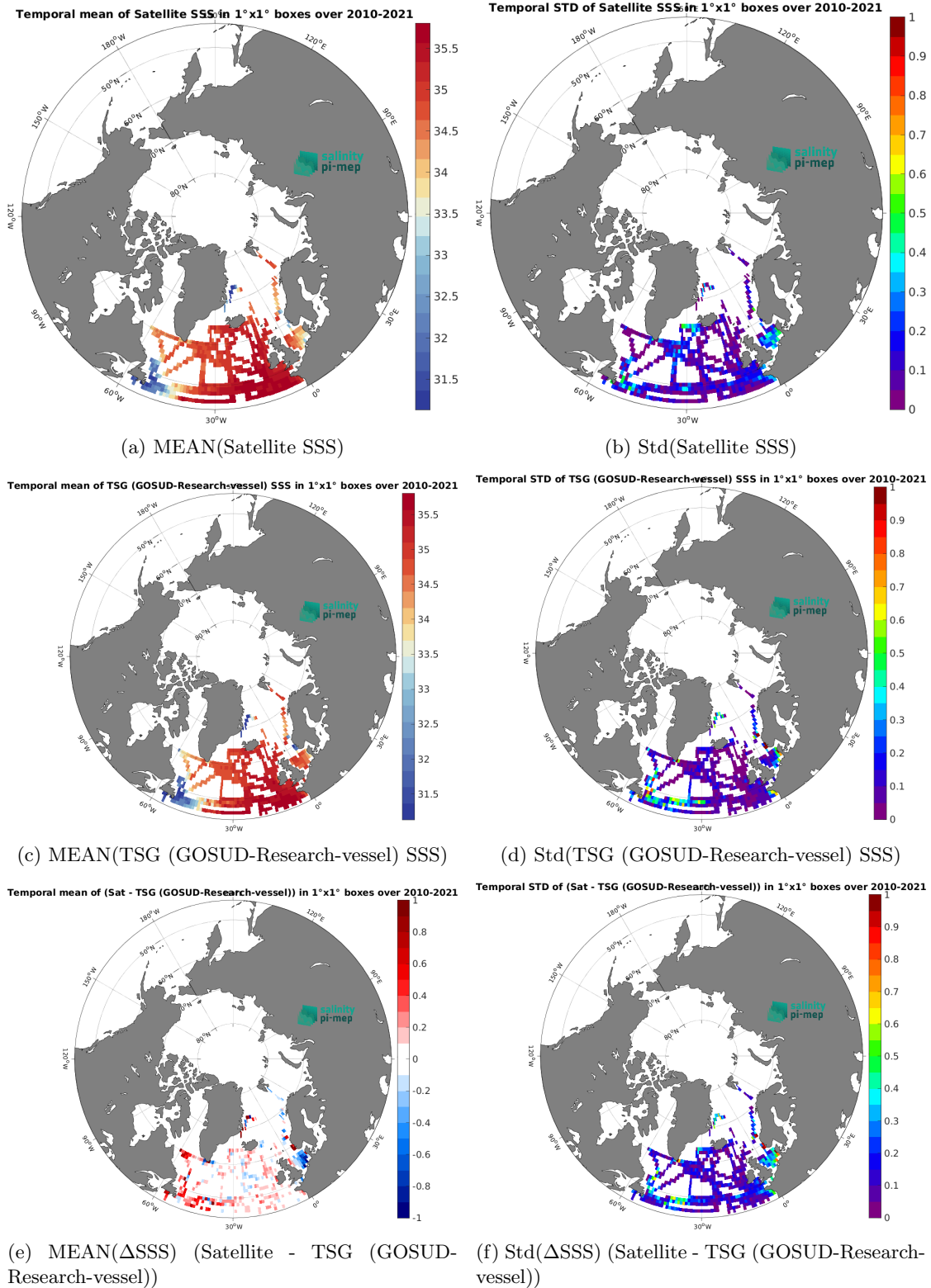
Figure 6: Temporal mean (left) and Std (right) of SSS from CCI SSS L4 POLAR NH Merged-OI v4.4 - 30-day running (ESA) (top), TSG (GOSUD-Research-vessel) (middle), and of \Delta SSS (Satellite - TSG (GOSUD-Research-vessel)). Only match-up pairs are used to generate these maps.
