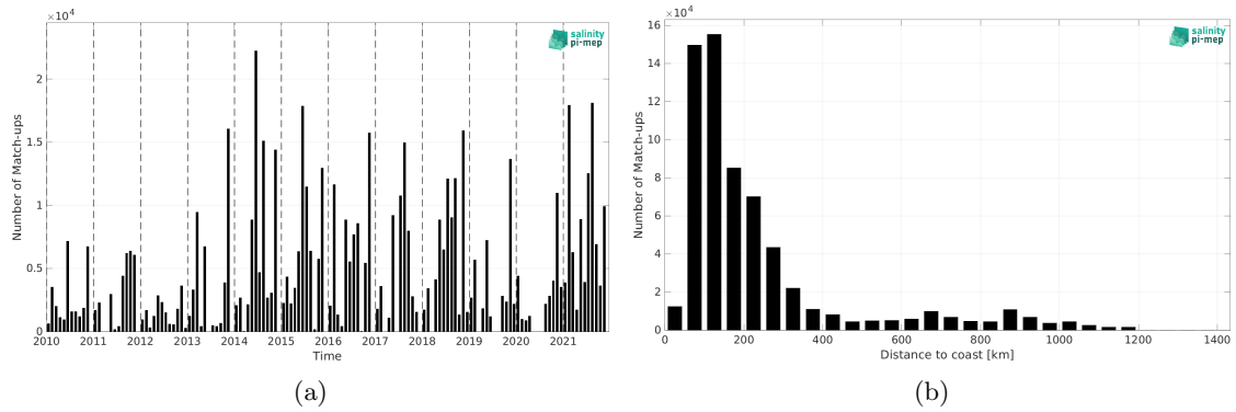
Figure 1: Number of match-ups between TSG (GOSUD-Research-vessel) and CCI SSS L4 POLAR NH Merged-OI v4.4 - 30-day running (ESA) SSS as a function of time (a) and as function of the distance to coast (b) over the Global Ocean Pi-MEP region and for the full satellite product period.
