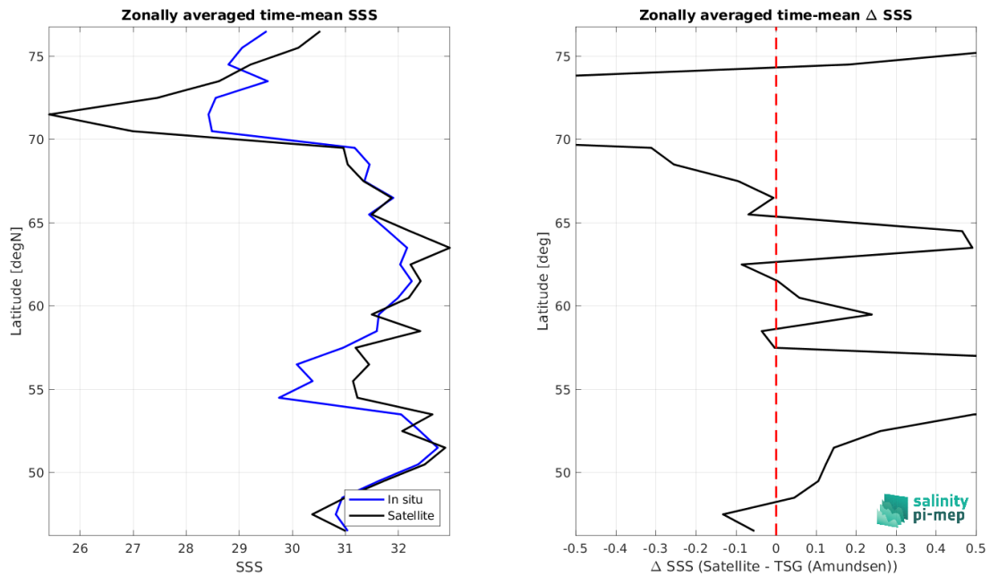
Figure 8: Left panel: Zonal mean SSS from CCI SSS L4 POLAR NH Merged-OI v4.4 - 30-day running (ESA) satellite product (black) and from TSG (Amundsen) (blue). Right panel: Zonal mean of \Delta SSS (Satellite - TSG (Amundsen)) for all the collected Pi-MEP match-up pairs estimated over the full satellite product period.
