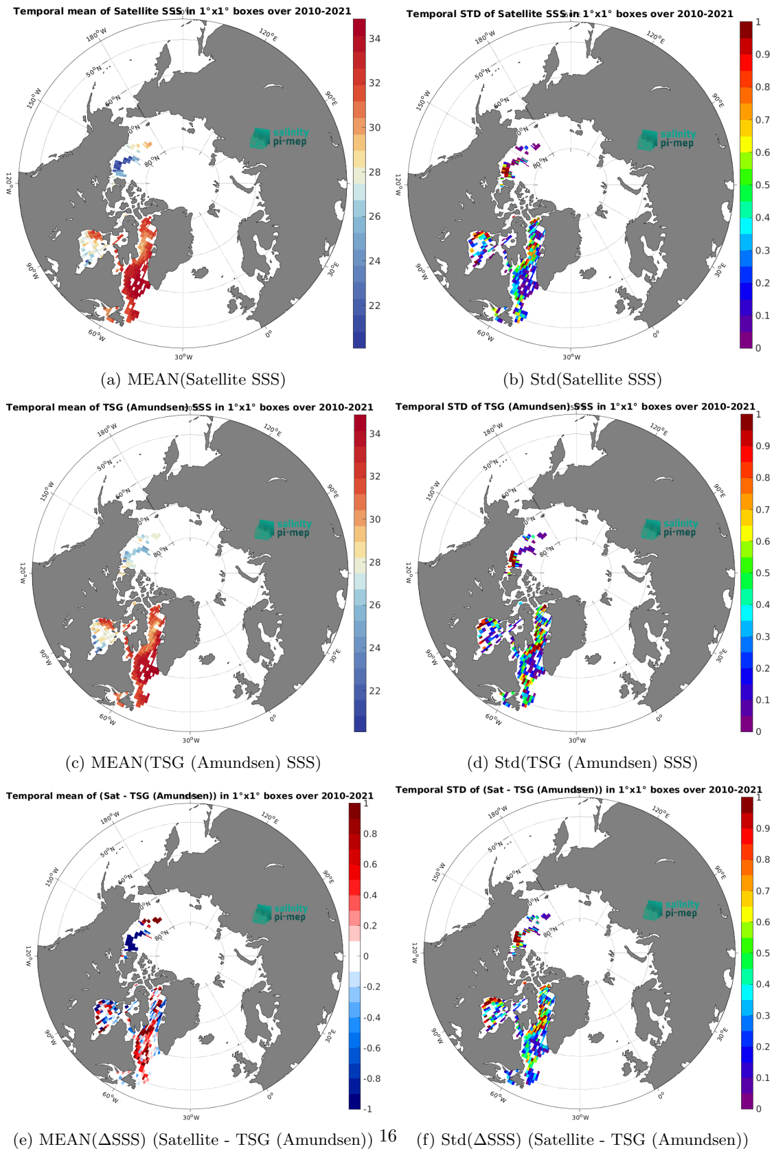
Figure 6: Temporal mean (left) and Std (right) of SSS from CCI SSS L4 POLAR NH Merged-OI v4.4 - 30-day running (ESA) (top), TSG (Amundsen) (middle), and of \Delta SSS (Satellite - TSG (Amundsen)). Only match-up pairs are used to generate these maps.
