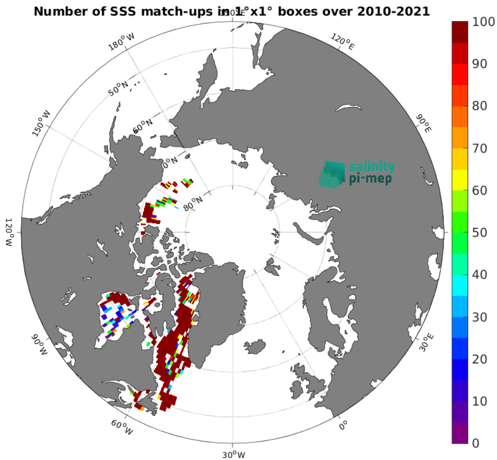
Figure 4: Number of SSS match-ups between TSG (Amundsen) SSS and the CCI SSS L4 POLAR NH Merged-OI v4.4 - 30-day running (ESA) SSS product for the Global Ocean Pi-MEP region over 1^{\circ} \times 1^{\circ} boxes and for the full satellite product period.
