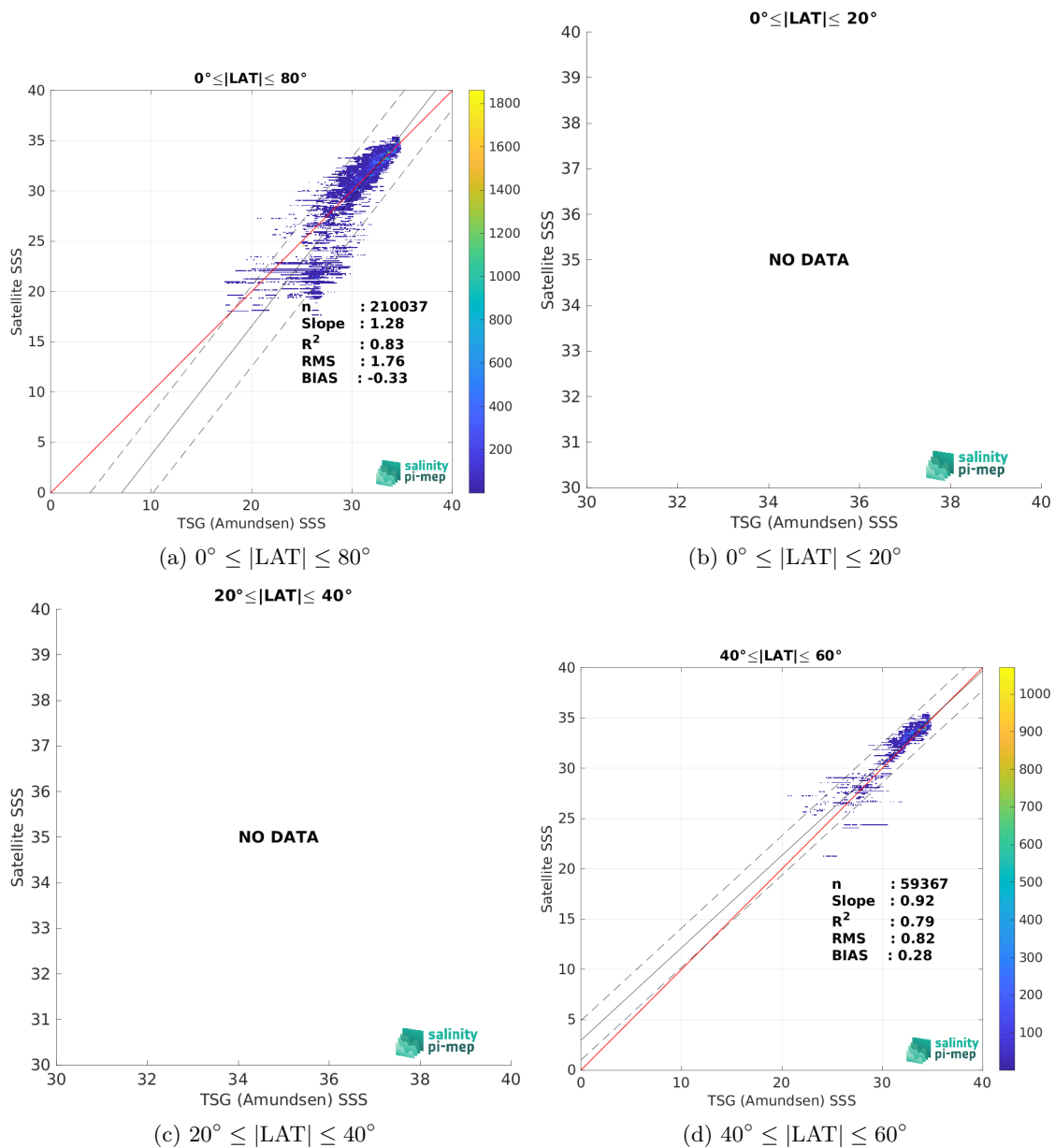
Figure 9: Contour maps of the concentration of CCI SSS L4 POLAR NH Merged-OI v4.4 - 30-day running (ESA) SSS (y-axis) versus TSG (Amundsen) SSS (x-axis) at match-up pairs for different latitude bands. For each plot, the red line shows x=y . The black thin and dashed lines indicate a linear fit through the data cloud and the \pm 95\% confidence levels, respectively. The number match-up pairs n , the slope and R^2 coefficient of the linear fit, the root mean square (RMS) and the mean bias between satellite and in situ data are indicated for each latitude band in each plots.
