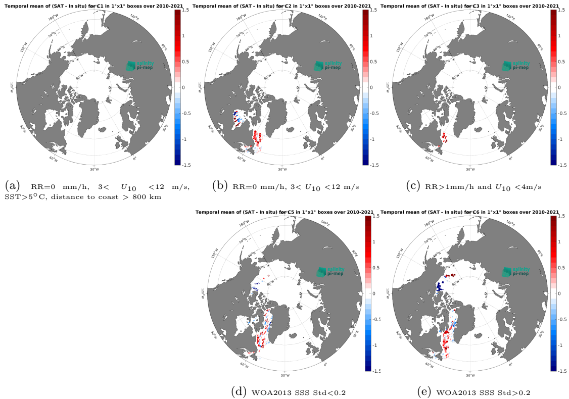
Figure 12: Temporal mean gridded over spatial boxes of size 1^{\circ}\times 1^{\circ} of \Delta\text{SSS} (CCI SSS L4 POLAR NH Merged-OI v4.4 - 30-day running (ESA) - TSG (Amundsen)) for 5 different subdatasets corresponding to:RR=0 mm/h, 3 < U_{10} < 12 m/s, SST >5^{\circ}\text{C} , distance to coast > 800 km (a), RR=0 mm/h, 3 < U_{10} < 12 m/s (b), RR >1 mm/h and U_{10} < 4 m/s (c), WOA2013 SSS Std <0.2 (d), WOA2013 SSS Std >0.2 (e).
