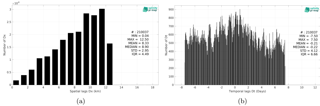
Figure 5: Histograms of the spatial (a) and temporal (b) lags between the location/time of the TSG (Amundsen) measurement and the date of the corresponding CCI SSS L4 POLAR NH Merged-OI v4.4 - 30-day running (ESA) SSS pixel.
