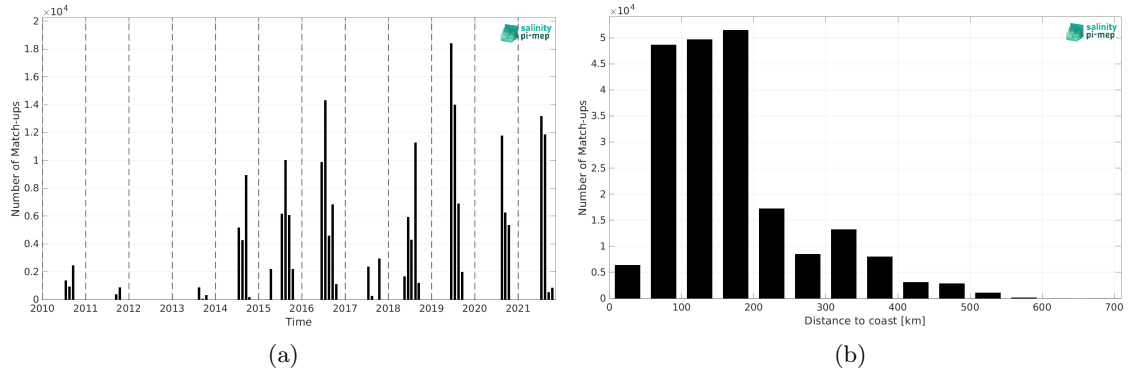
Figure 1: Number of match-ups between TSG (Amundsen) and CCI SSS L4 POLAR NH Merged-OI v4.4 - 30-day running (ESA) SSS as a function of time (a) and as function of the distance to coast (b) over the Global Ocean Pi-MEP region and for the full satellite product period.
