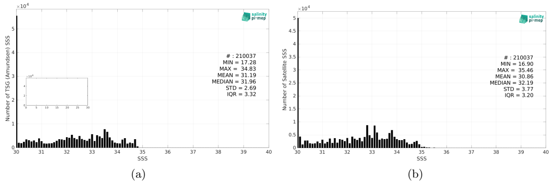
Figure 2: Histograms of SSS from TSG (Amundsen) (a) and CCI SSS L4 POLAR NH Merged-OI v4.4 - 30-day running (ESA) (b) considering all match-up pairs per bins of 0.1 over the Global Ocean Pi-MEP region and for the full satellite product period.
