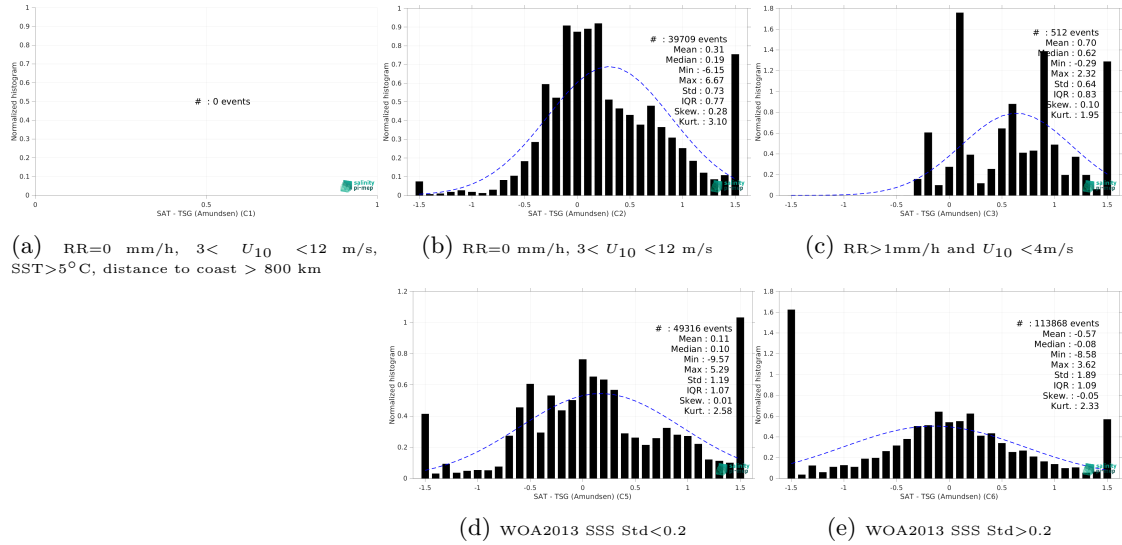
Figure 13: Normalized histogram of \Delta SSS (CCI SSS L4 POLAR NH Merged-OI v4.4 - 30-day running (ESA) - TSG (Amundsen)) for 5 different subdatasets corresponding to: RR=0 mm/h, 3 < U_{10} < 12 m/s, SST > 5°C, distance to coast > 800 km (a), RR=0 mm/h, 3 < U_{10} < 12 m/s (b), RR > 1mm/h and U_{10} < 4 m/s (c), WOA2013 SSS Std < 0.2 (d), WOA2013 SSS Std > 0.2 (e).
