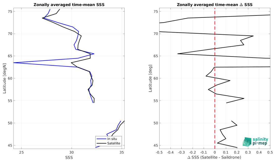
Figure 8: Left panel: Zonal mean SSS from CCI SSS L4 POLAR NH Merged-OI v4.4 - 30-day running (ESA) satellite product (black) and from Saildrone (blue). Right panel: Zonal mean of \Delta SSS (Satellite - Saildrone) for all the collected Pi-MEP match-up pairs estimated over the full satellite product period.
