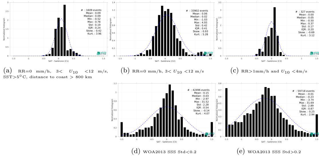
Figure 13: Normalized histogram of \Delta SSS (CCI SSS L4 POLAR NH Merged-OI v4.4 - 30-day running (ESA) - Saildrone) for 5 different subdatasets corresponding to: RR=0 mm/h, 3 < U_{10} < 12 m/s, SST>5°C, distance to coast > 800 km (a), RR=0 mm/h, 3 < U_{10} < 12 m/s (b), RR>1mm/h and U_{10} < 4 m/s (c), WOA2013 SSS Std<0.2 (d), WOA2013 SSS Std>0.2 (e).
