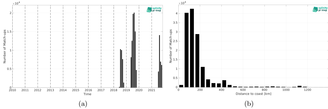
Figure 1: Number of match-ups between Saildrone and CCI SSS L4 POLAR NH Merged-OI v4.4 - 30-day running (ESA) SSS as a function of time (a) and as function of the distance to coast (b) over the Global Ocean Pi-MEP region and for the full satellite product period.
