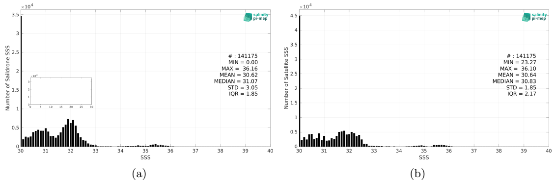
Figure 2: Histograms of SSS from Saildrone (a) and CCI SSS L4 POLAR NH Merged-OI v4.4 - 30-day running (ESA) (b) considering all match-up pairs per bins of 0.1 over the Global Ocean Pi-MEP region and for the full satellite product period.
