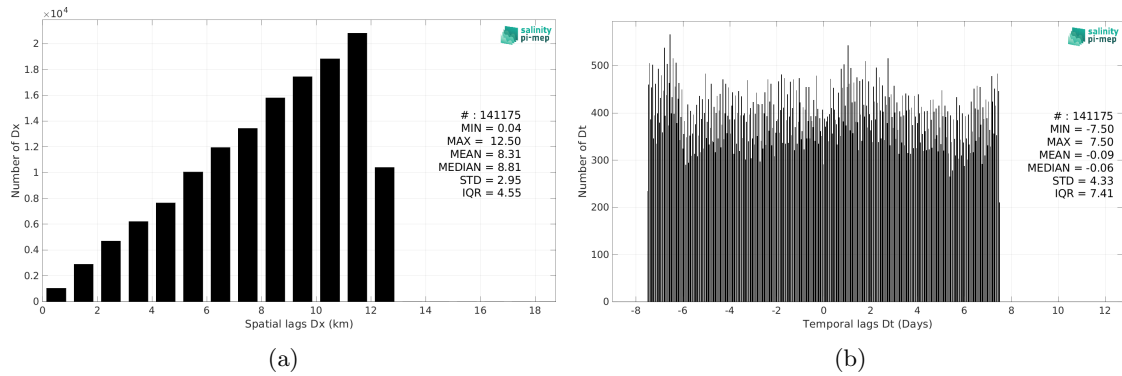
Figure 5: Histograms of the spatial (a) and temporal (b) lags between the location/time of the Saildrone measurement and the date of the corresponding CCI SSS L4 POLAR NH Merged-OI v4.4 - 30-day running (ESA) SSS pixel.
