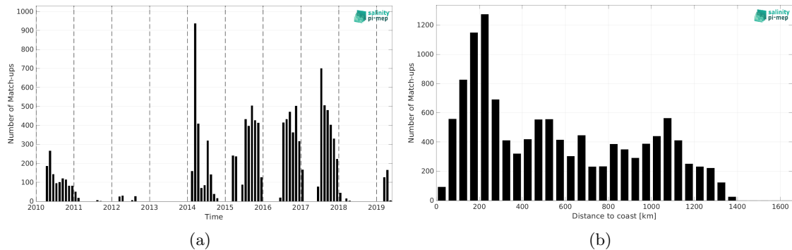
Figure 1: Number of match-ups between Marine mammals and CCI SSS L4 POLAR NH Merged-OI v4.4 - 30-day running (ESA) SSS as a function of time (a) and as function of the distance to coast (b) over the Global Ocean Pi-MEP region and for the full satellite product period.
