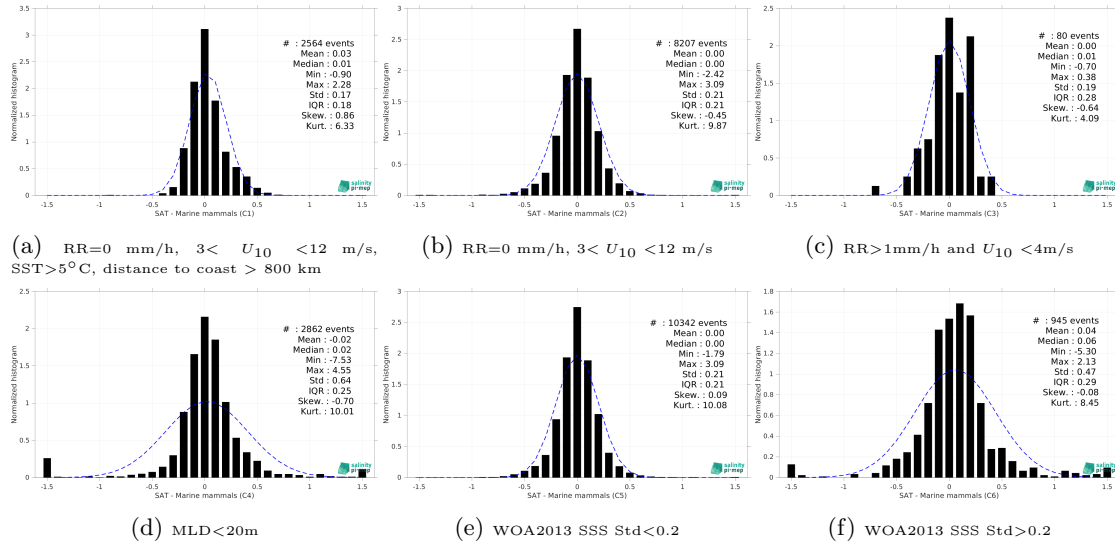
Figure 13: Normalized histogram of \Delta SSS (CCI SSS L4 POLAR NH Merged-OI v4.4 - 30-day running (ESA) - Marine mammals) for 6 different subdatasets corresponding to: RR=0 mm/h, 3 < U_{10} < 12 m/s, SST>5°C, distance to coast > 800 km (a), RR=0 mm/h, 3 < U_{10} < 12 m/s (b), RR>1mm/h and U_{10} < 4 m/s (c), MLD<20m (d), WOA2013 SSS Std<0.2 (e), WOA2013 SSS Std>0.2 (f).
