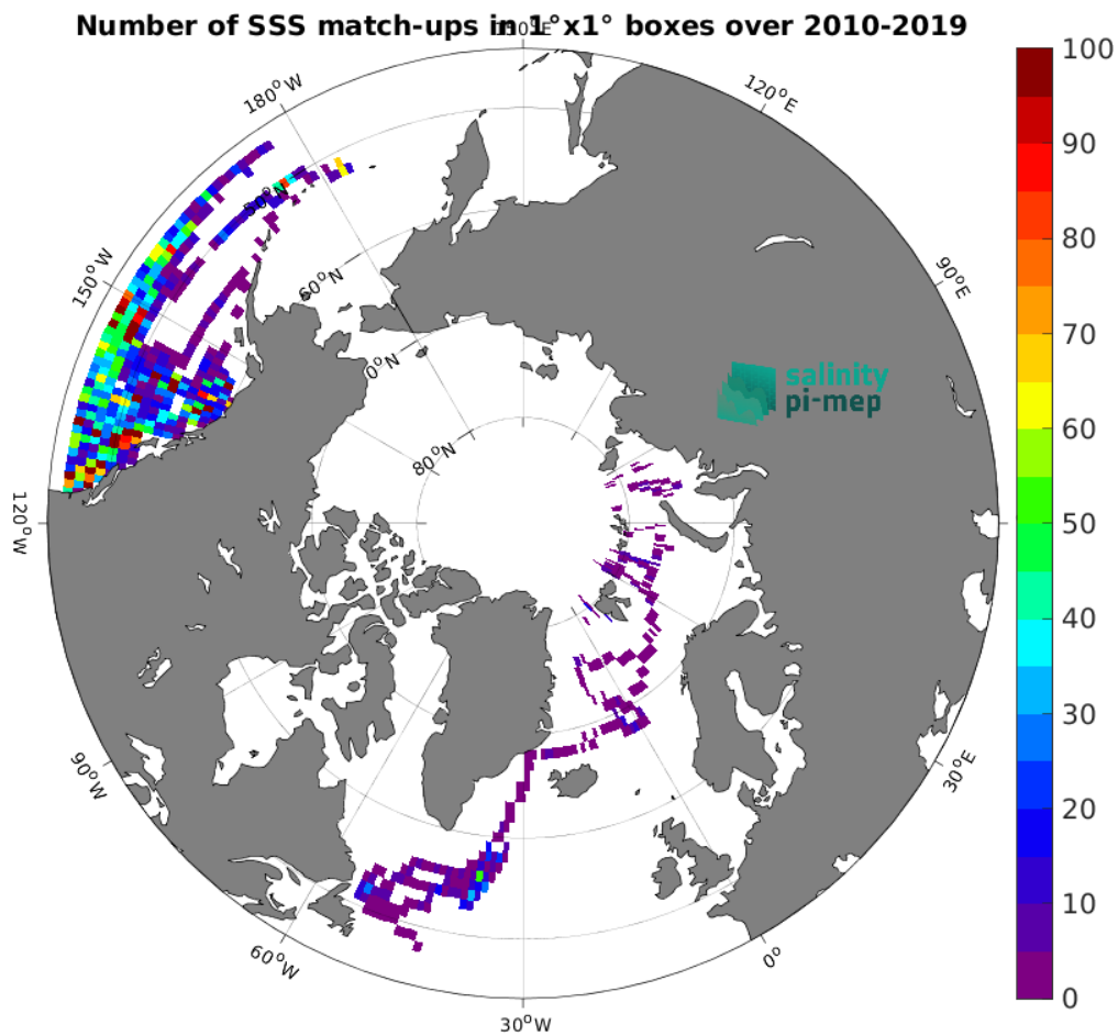
Figure 4: Number of SSS match-ups between Marine mammals SSS and the CCI SSS L4 POLAR NH Merged-OI v4.4 - 30-day running (ESA) SSS product for the Global Ocean Pi-MEP region over 1^{\circ} \times 1^{\circ} boxes and for the full satellite product period.
