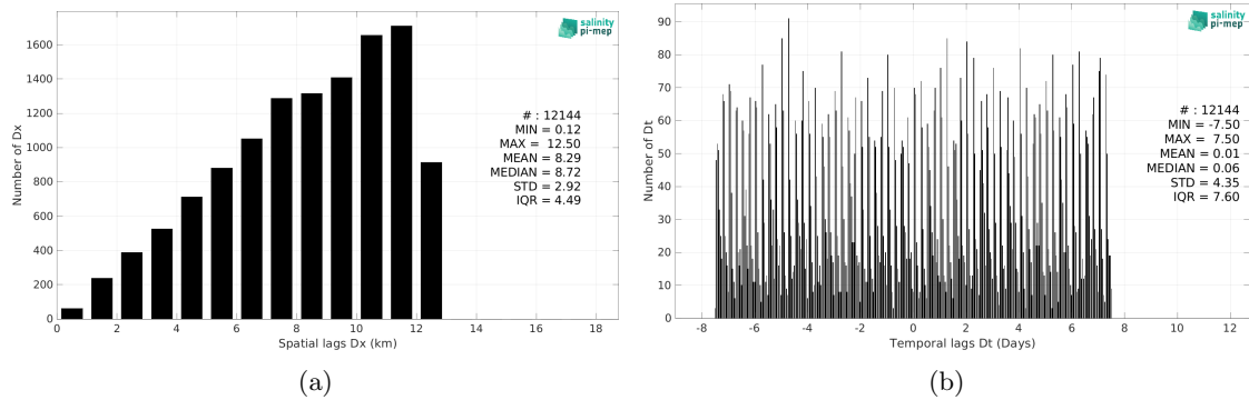
Figure 5: Histograms of the spatial (a) and temporal (b) lags between the location/time of the Marine mammals measurement and the date of the corresponding CCI SSS L4 POLAR NH Merged-OI v4.4 - 30-day running (ESA) SSS pixel.
