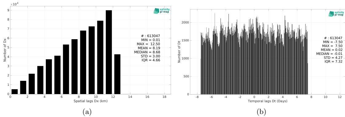
Figure 5: Histograms of the spatial (a) and temporal (b) lags between the location/time of the ICES measurement and the date of the corresponding CCI SSS L4 POLAR NH Merged-OI v4.4 - 30-day running (ESA) SSS pixel.
