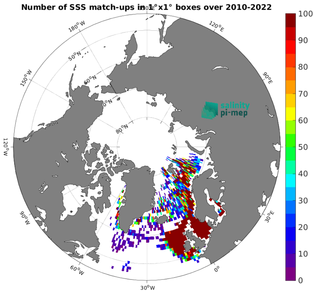
Figure 4: Number of SSS match-ups between ICES SSS and the CCI SSS L4 POLAR NH Merged-OI v4.4 - 30-day running (ESA) SSS product for the Global Ocean Pi-MEP region over 1^\circ \times 1^\circ boxes and for the full satellite product period.
