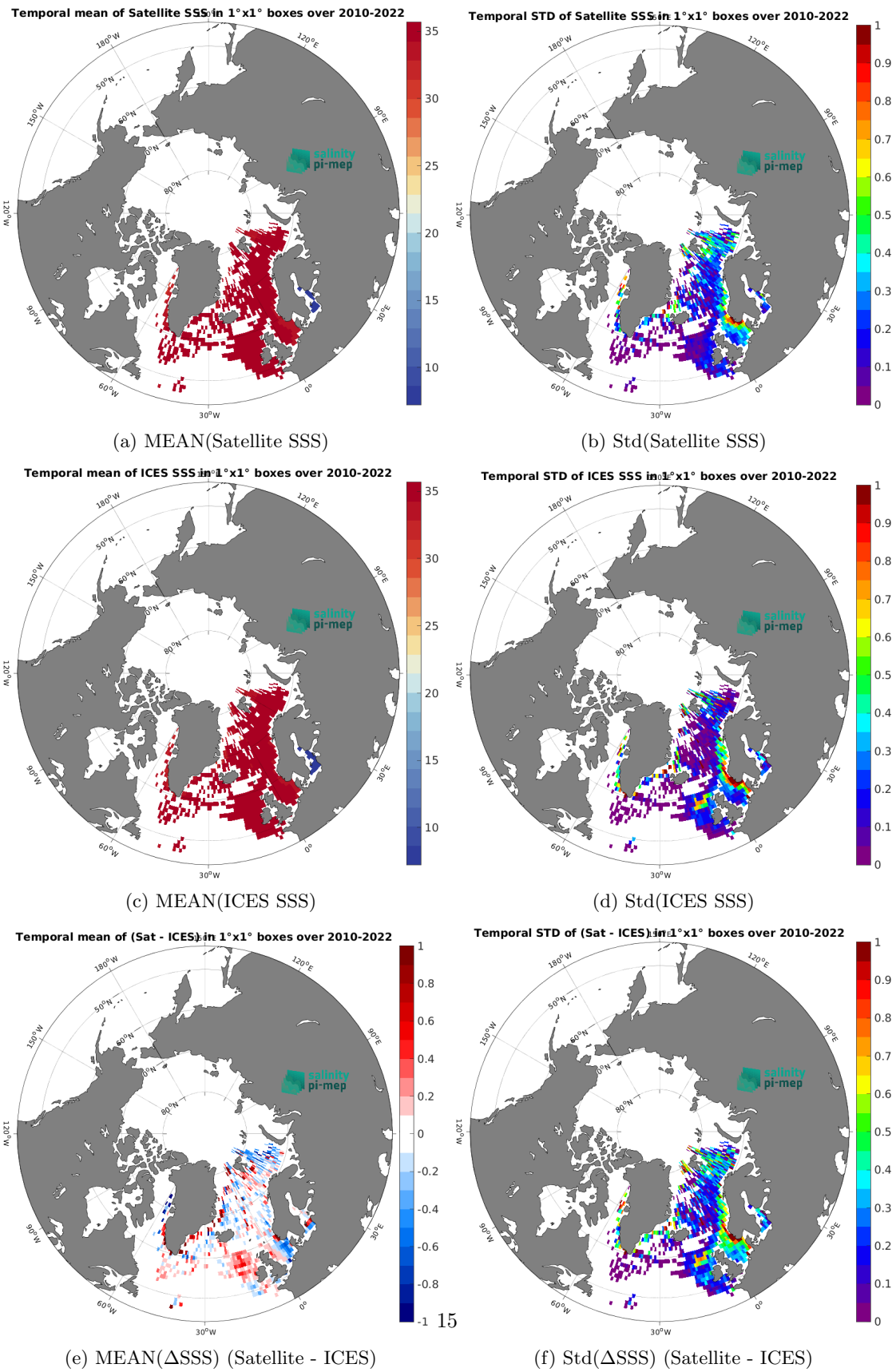
Figure 6: Temporal mean (left) and Std (right) of SSS from CCI SSS L4 POLAR NH Merged-OI v4.4 - 30-day running (ESA) (top), ICES (middle), and of \Delta SSS (Satellite - ICES). Only match-up pairs are used to generate these maps.
