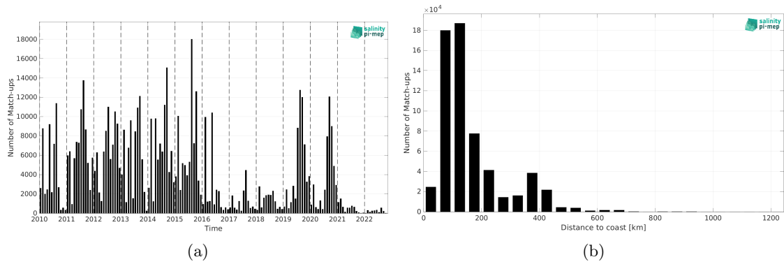
Figure 1: Number of match-ups between ICES and CCI SSS L4 POLAR NH Merged-OI v4.4 - 30-day running (ESA) SSS as a function of time (a) and as function of the distance to coast (b) over the Global Ocean Pi-MEP region and for the full satellite product period.
