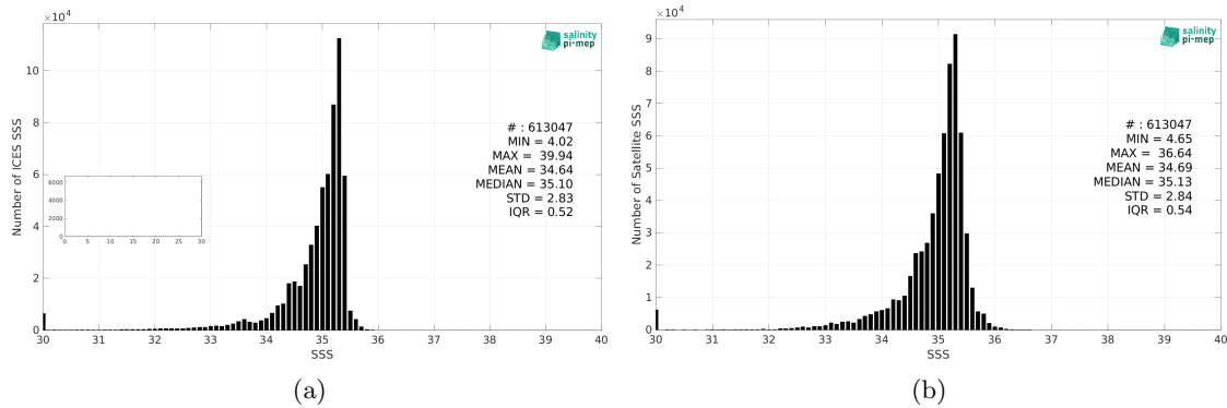
Figure 2: Histograms of SSS from ICES (a) and CCI SSS L4 POLAR NH Merged-OI v4.4 - 30-day running (ESA) (b) considering all match-up pairs per bins of 0.1 over the Global Ocean Pi-MEP region and for the full satellite product period.
