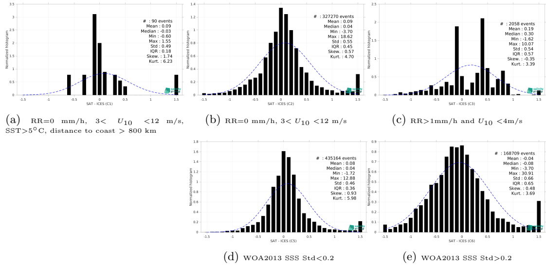
Figure 13: Normalized histogram of \Delta SSS (CCI SSS L4 POLAR NH Merged-OI v4.4 - 30-day running (ESA) - ICES) for 5 different subdatasets corresponding to: RR=0 mm/h, 3 < U_{10} < 12 m/s, SST > 5°C, distance to coast > 800 km (a), RR=0 mm/h, 3 < U_{10} < 12 m/s (b), RR > 1mm/h and U_{10} < 4 m/s (c), WOA2013 SSS Std < 0.2 (d), WOA2013 SSS Std > 0.2 (e).
