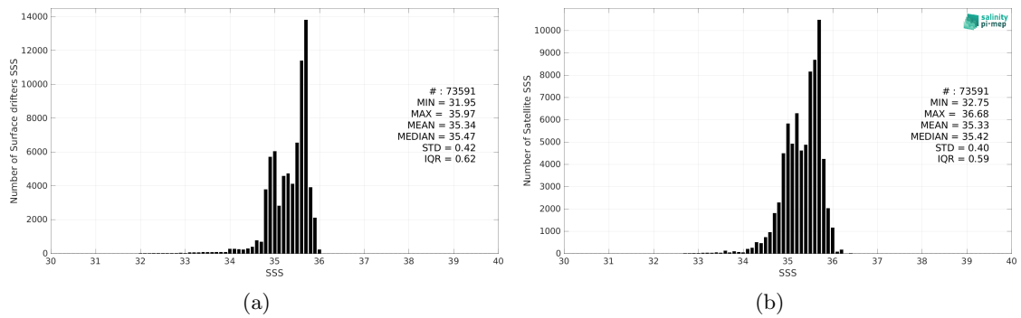
Figure 2: Histograms of SSS from Surface drifters (a) and CCI SSS L4 POLAR NH Merged-OI v4.4 - 30-day running (ESA) (b) considering all match-up pairs per bins of 0.1 over the Global Ocean Pi-MEP region and for the full satellite product period.
