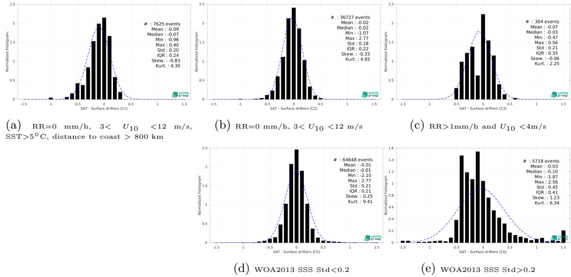
Figure 12: Normalized histogram of \Delta SSS (CCI SSS L4 POLAR NH Merged-OI v4.4 - 30-day running (ESA) - Surface drifters) for 5 different subdatasets corresponding to: RR=0 mm/h, 3 < U_{10} < 12 m/s, SST > 5°C, distance to coast > 800 km (a), RR=0 mm/h, 3 < U_{10} < 12 m/s (b), RR > 1mm/h and U_{10} < 4 m/s (c), WOA2013 SSS Std < 0.2 (d), WOA2013 SSS Std > 0.2 (e).
