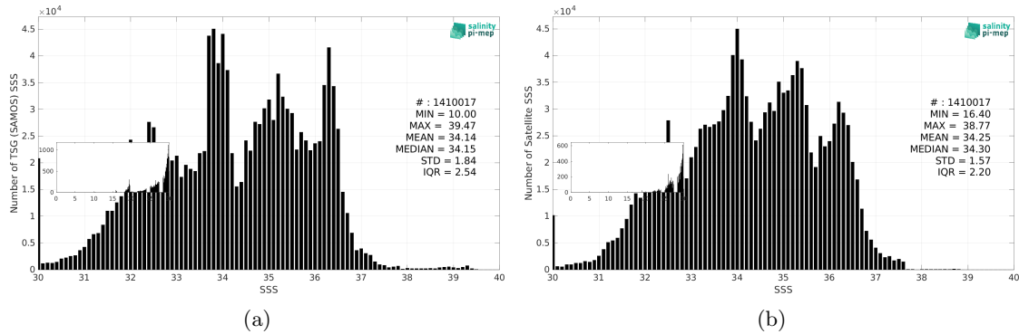
Figure 3: Histograms of SSS from TSG (SAMOS) (a) and CCI SSS L4 Merged-OI v5.5 - 7-day running (ESA) (b) considering all match-up pairs per bins of 0.1 over the Global Ocean Pi-MEP region and for the full satellite product period.
