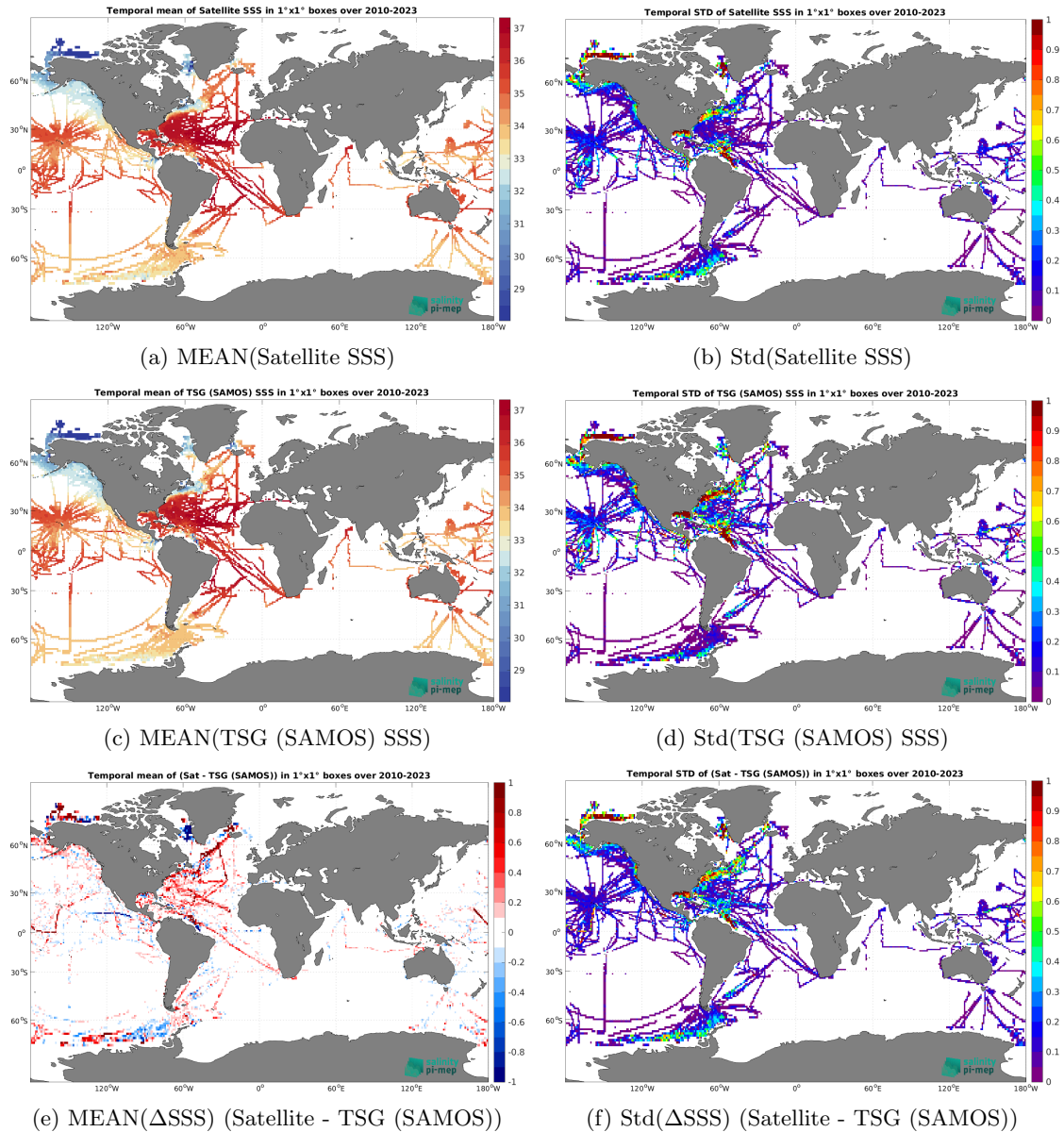
Figure 7: Temporal mean (left) and Std (right) of SSS from CCI SSS L4 Merged-OI v5.5 - 7-day running (ESA) (top), TSG (SAMOS) (middle), and of \Delta SSS (Satellite - TSG (SAMOS)). Only match-up pairs are used to generate these maps.
