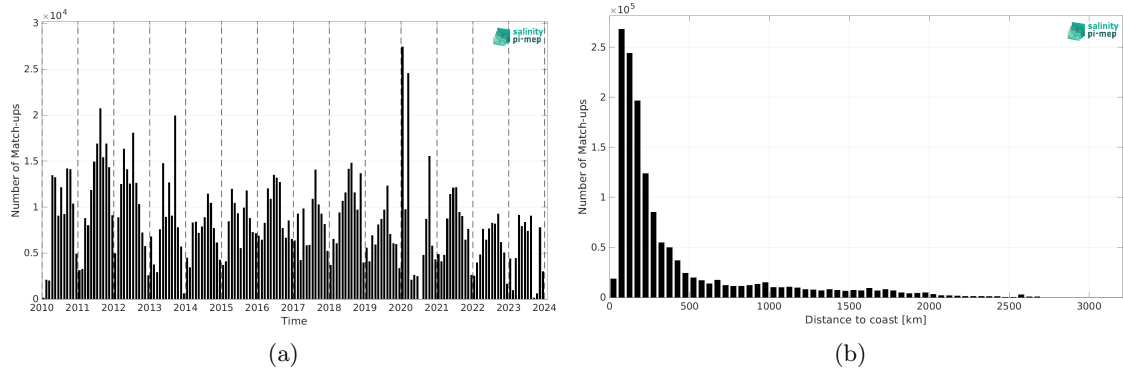
Figure 2: Number of match-ups between TSG (SAMOS) and CCI SSS L4 Merged-OI v5.5 - 7-day running (ESA) SSS as a function of time (a) and as function of the distance to coast (b) over the Global Ocean Pi-MEP region and for the full satellite product period.
