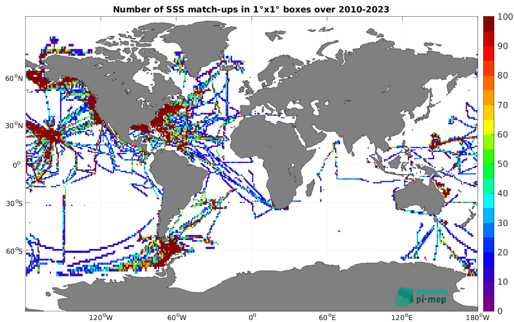
Figure 5: Number of SSS match-ups between TSG (SAMOS) SSS and the CCI SSS L4 Merged-OI v5.5 - 7-day running (ESA) SSS product for the Global Ocean Pi-MEP region over 1^\circ \times 1^\circ boxes and for the full satellite product period.
