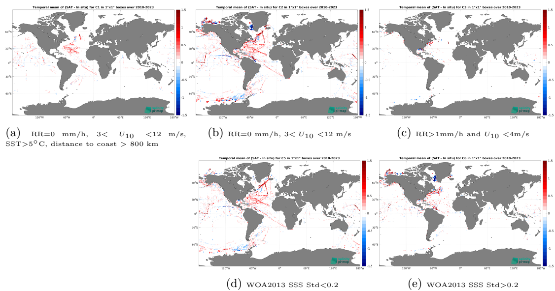
Figure 14: Temporal mean gridded over spatial boxes of size 1^\circ \times 1^\circ of \Delta\text{SSS} (CCI SSS L4 Merged-OI v5.5 - 7-day running (ESA) - TSG (SAMOS)) for 5 different subdatasets corresponding to:RR=0 mm/h, 3 < U_{10} < 12 m/s, SST > 5^\circ\text{C} , distance to coast > 800 km (a), RR=0 mm/h, 3 < U_{10} < 12 m/s (b), RR > 1 mm/h and U_{10} < 4 m/s (c), WOA2013 SSS Std < 0.2 (d), WOA2013 SSS Std > 0.2 (e).
