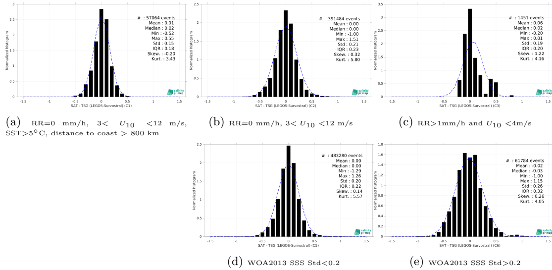
Figure 15: Normalized histogram of \Delta SSS (CCI SSS L4 Merged-OI v5.5 - 7-day running (ESA) - TSG (LEGOS-Survostral)) for 5 different subdatasets corresponding to: RR=0 mm/h, 3 < U_{10} < 12 m/s, SST>5°C, distance to coast > 800 km (a), RR=0 mm/h, 3 < U_{10} < 12 m/s (b), RR>1mm/h and U_{10} < 4 m/s (c), WOA2013 SSS Std<0.2 (d), WOA2013 SSS Std>0.2 (e).
