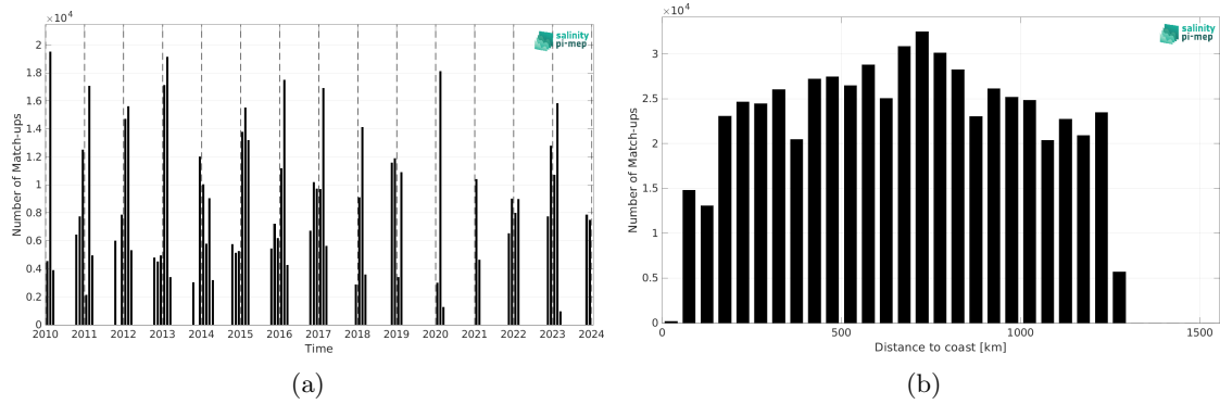
Figure 2: Number of match-ups between TSG (LEGOS-Survostral) and CCI SSS L4 Merged-OI v5.5 - 7-day running (ESA) SSS as a function of time (a) and as function of the distance to coast (b) over the Global Ocean Pi-MEP region and for the full satellite product period.
