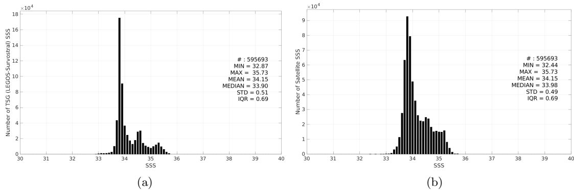
Figure 3: Histograms of SSS from TSG (LEGOS-Survostral) (a) and CCI SSS L4 Merged-OI v5.5 - 7-day running (ESA) (b) considering all match-up pairs per bins of 0.1 over the Global Ocean Pi-MEP region and for the full satellite product period.
