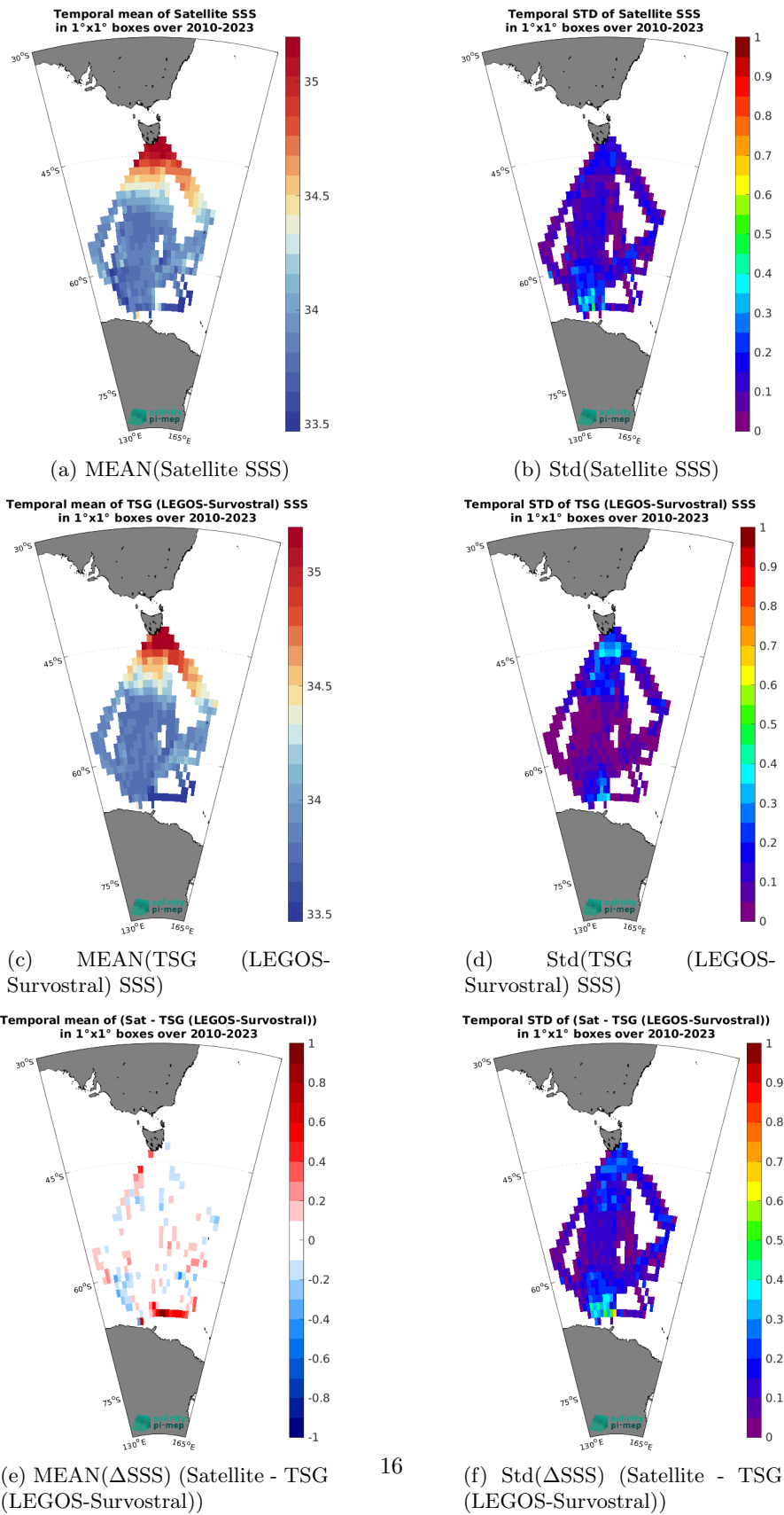
Figure 7: Temporal mean (left) and Std (right) of SSS from CCI SSS L4 Merged-OI v5.5 - 7-day running (ESA) (top), TSG (LEGOS-Survostral) (middle), and of \Delta SSS (Satellite - TSG (LEGOS-Survostral)). Only match-up pairs are used to generate these maps.
