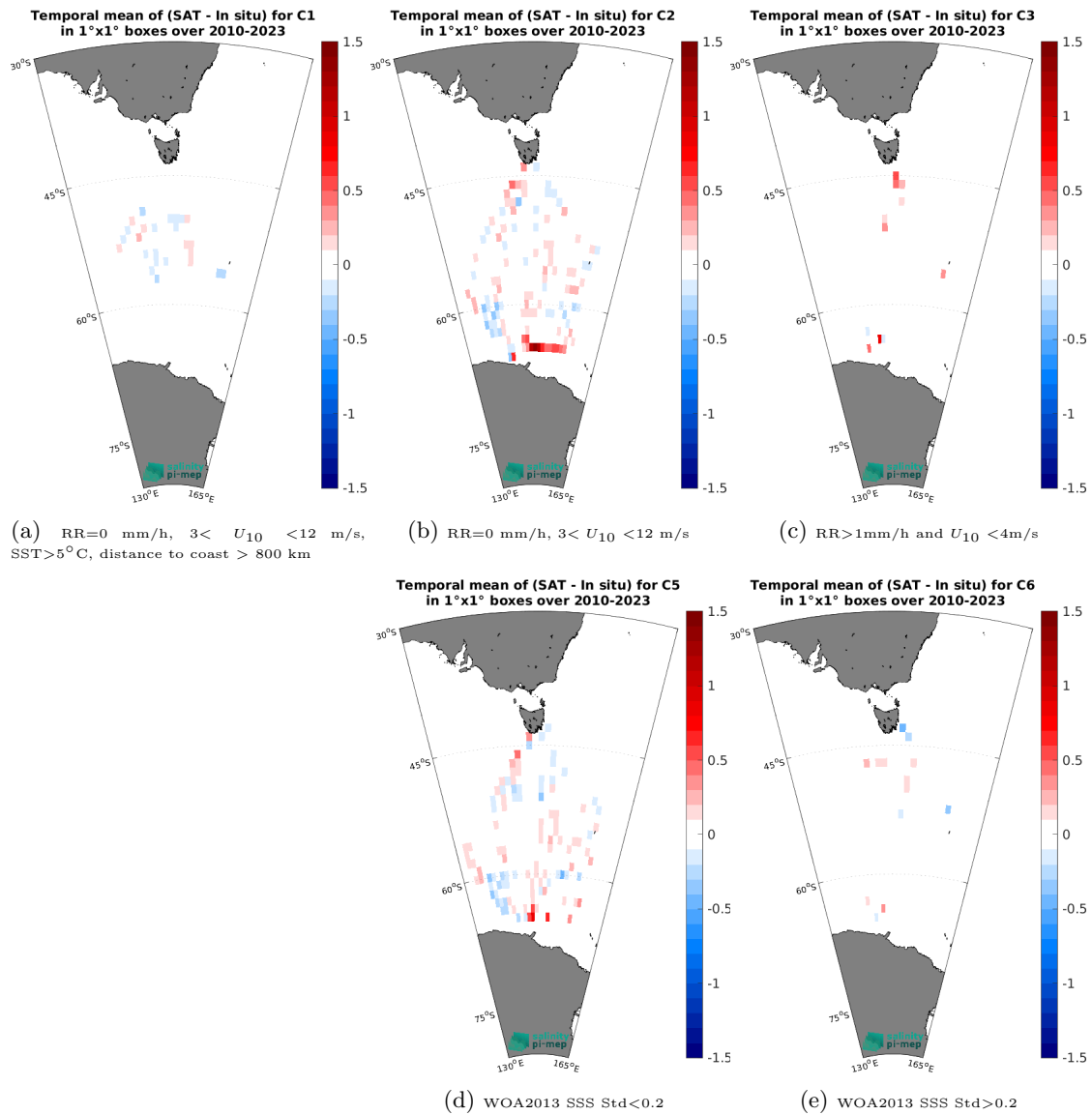
Figure 14: Temporal mean gridded over spatial boxes of size 1^{\circ} \times 1^{\circ} of \Delta\text{SSS} (CCI SSS L4 Merged-OI v5.5 - 7-day running (ESA) - TSG (LEGOS-Survostral)) for 5 different subdatasets corresponding to: RR=0 mm/h, 3 < U_{10} < 12 m/s, SST > 5^{\circ}\text{C} , distance to coast > 800 km (a), RR=0 mm/h, 3 < U_{10} < 12 m/s (b), RR > 1 mm/h and U_{10} < 4 m/s (c), WOA2013 SSS Std < 0.2 (d), WOA2013 SSS Std > 0.2 (e).
