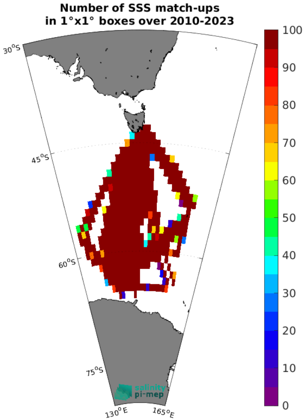
Figure 5: Number of SSS match-ups between TSG (LEGOS-Survostral) SSS and the CCI SSS L4 Merged-OI v5.5 - 7-day running (ESA) SSS product for the Global Ocean Pi-MEP region over 1°x1° boxes and for the full satellite product period.
