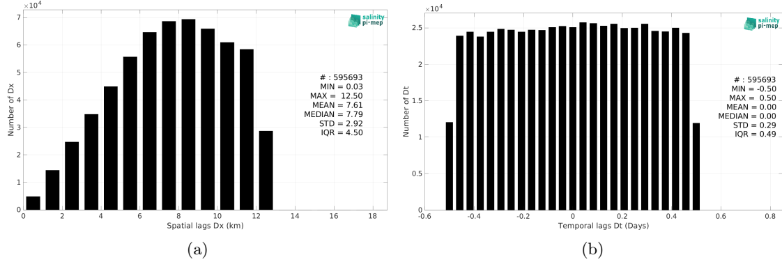
Figure 6: Histograms of the spatial (a) and temporal (b) lags between the location/time of the TSG (LEGOS-Survostral) measurement and the date of the corresponding CCI SSS L4 Merged-OI v5.5 - 7-day running (ESA) SSS pixel.
