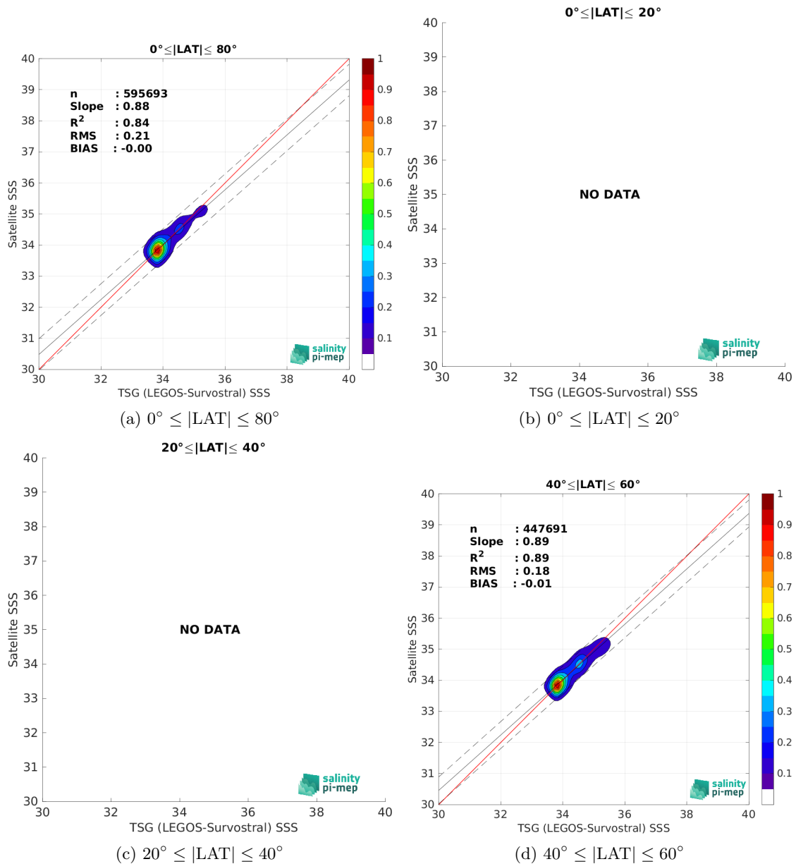
Figure 10: Contour maps of the concentration of CCI SSS L4 Merged-OI v5.5 - 7-day running (ESA) SSS (y-axis) versus TSG (LEGOS-Survostral) SSS (x-axis) at match-up pairs for different latitude bands. For each plot, the red line shows x=y . The black thin and dashed lines indicate a linear fit through the data cloud and the \pm 95\% confidence levels, respectively. The number match-up pairs n , the slope and R^2 coefficient of the linear fit, the root mean square (RMS) and the mean bias between satellite and in situ data are indicated for each latitude band in each plots.
