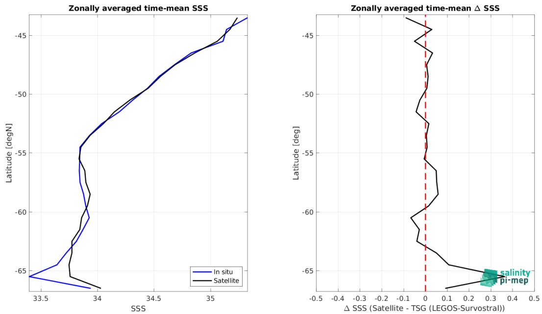
Figure 9: Left panel: Zonal mean SSS from CCI SSS L4 Merged-OI v5.5 - 7-day running (ESA) satellite product (black) and from TSG (LEGOS-Survostral) (blue). Right panel: Zonal mean of \Delta SSS (Satellite - TSG (LEGOS-Survostral)) for all the collected Pi-MEP match-up pairs estimated over the full satellite product period.
