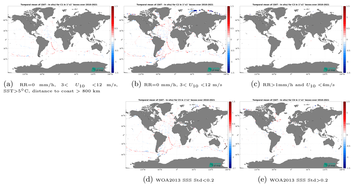
Figure 14: Temporal mean gridded over spatial boxes of size 1^\circ \times 1^\circ of \Delta SSS (CCI SSS L4 Merged-OI v5.5 - 7-day running (ESA) - TSG (GOSUD-Sailing-ship)) for 5 different subdatasets corresponding to:RR=0 mm/h, 3 < U_{10} < 12 m/s, SST > 5^\circ\text{C} , distance to coast > 800 km (a), RR=0 mm/h, 3 < U_{10} < 12 m/s (b), RR > 1 mm/h and U_{10} < 4 m/s (c), WOA2013 SSS Std < 0.2 (d), WOA2013 SSS Std > 0.2 (e).
