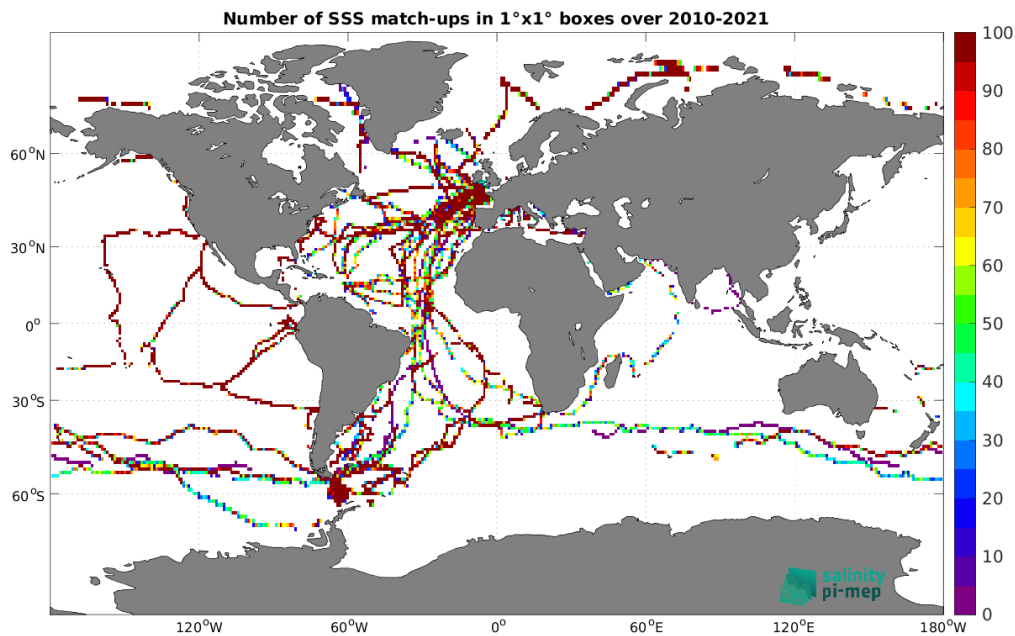
Figure 5: Number of SSS match-ups between TSG (GOSUD-Sailing-ship) SSS and the CCI SSS L4 Merged-OI v5.5 - 7-day running (ESA) SSS product for the Global Ocean Pi-MEP region over 1^\circ \times 1^\circ boxes and for the full satellite product period.
