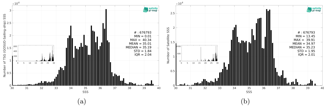
Figure 3: Histograms of SSS from TSG (GOSUD-Sailing-ship) (a) and CCI SSS L4 Merged-OI v5.5 - 7-day running (ESA) (b) considering all match-up pairs per bins of 0.1 over the Global Ocean Pi-MEP region and for the full satellite product period.
