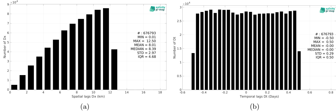
Figure 6: Histograms of the spatial (a) and temporal (b) lags between the location/time of the TSG (GOSUD-Sailing-ship) measurement and the date of the corresponding CCI SSS L4 Merged-OI v5.5 - 7-day running (ESA) SSS pixel.
