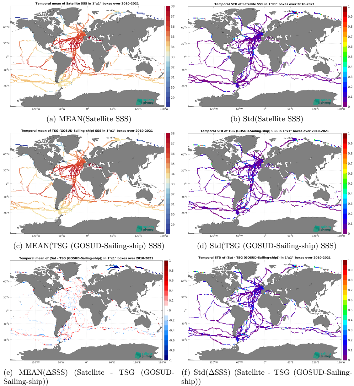
Figure 7: Temporal mean (left) and Std (right) of SSS from CCI SSS L4 Merged-OI v5.5 - 7-day running (ESA) (top), TSG (GOSUD-Sailing-ship) (middle), and of \Delta SSS (Satellite - TSG (GOSUD-Sailing-ship)). Only match-up pairs are used to generate these maps.
