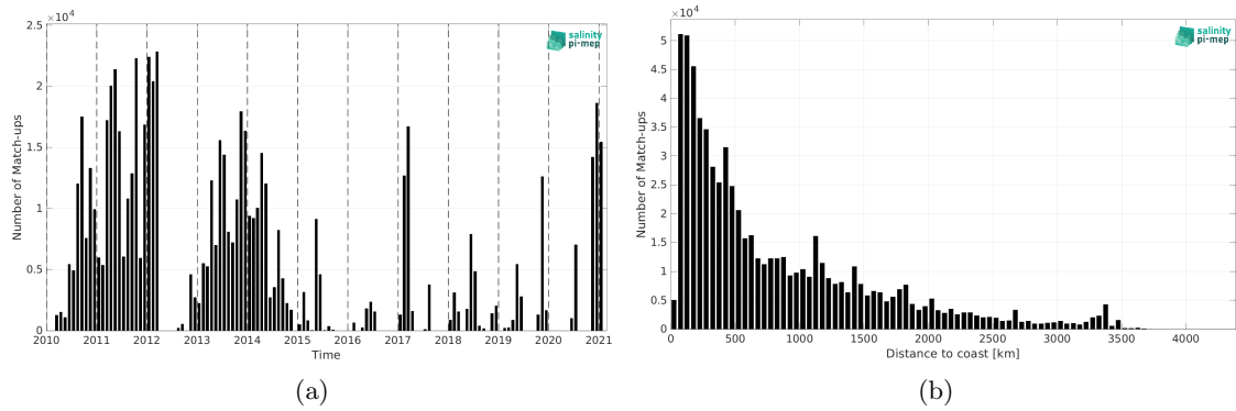
Figure 2: Number of match-ups between TSG (GOSUD-Sailing-ship) and CCI SSS L4 Merged-OI v5.5 - 7-day running (ESA) SSS as a function of time (a) and as function of the distance to coast (b) over the Global Ocean Pi-MEP region and for the full satellite product period.
