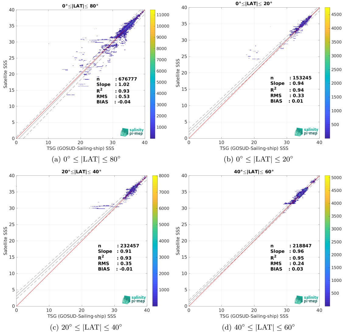
Figure 10: Contour maps of the concentration of CCI SSS L4 Merged-OI v5.5 - 7-day running (ESA) SSS (y-axis) versus TSG (GOSUD-Sailing-ship) SSS (x-axis) at match-up pairs for different latitude bands. For each plot, the red line shows x=y . The black thin and dashed lines indicate a linear fit through the data cloud and the \pm 95\% confidence levels, respectively. The number match-up pairs n , the slope and R^2 coefficient of the linear fit, the root mean square (RMS) and the mean bias between satellite and in situ data are indicated for each latitude band in each plots.
