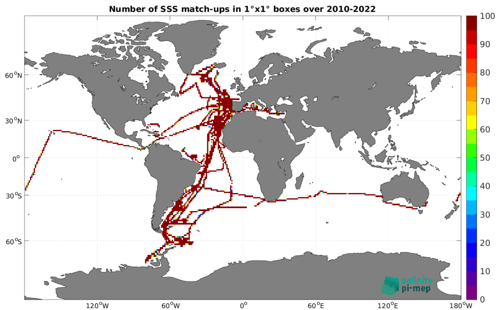
Figure 5: Number of SSS match-ups between TSG (CSIC-UTM) SSS and the CCI SSS L4 Merged-OI v5.5 - 7-day running (ESA) SSS product for the Global Ocean Pi-MEP region over 1^\circ \times 1^\circ boxes and for the full satellite product period.
