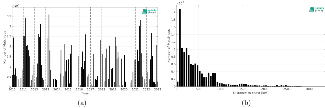
Figure 2: Number of match-ups between TSG (CSIC-UTM) and CCI SSS L4 Merged-OI v5.5 - 7-day running (ESA) SSS as a function of time (a) and as function of the distance to coast (b) over the Global Ocean Pi-MEP region and for the full satellite product period.
