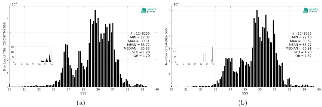
Figure 3: Histograms of SSS from TSG (CSIC-UTM) (a) and CCI SSS L4 Merged-OI v5.5 - 7-day running (ESA) (b) considering all match-up pairs per bins of 0.1 over the Global Ocean Pi-MEP region and for the full satellite product period.
