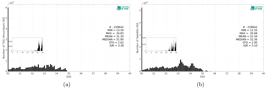
Figure 3: Histograms of SSS from TSG (Amundsen) (a) and CCI SSS L4 Merged-OI v5.5 - 7-day running (ESA) (b) considering all match-up pairs per bins of 0.1 over the Global Ocean Pi-MEP region and for the full satellite product period.
