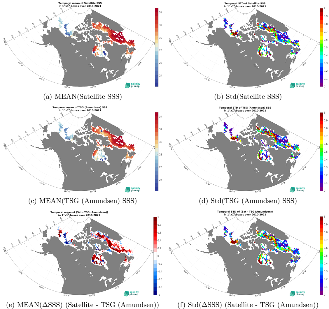
Figure 7: Temporal mean (left) and Std (right) of SSS from CCI SSS L4 Merged-OI v5.5 - 7-day running (ESA) (top), TSG (Amundsen) (middle), and of \Delta SSS (Satellite - TSG (Amundsen)). Only match-up pairs are used to generate these maps.
