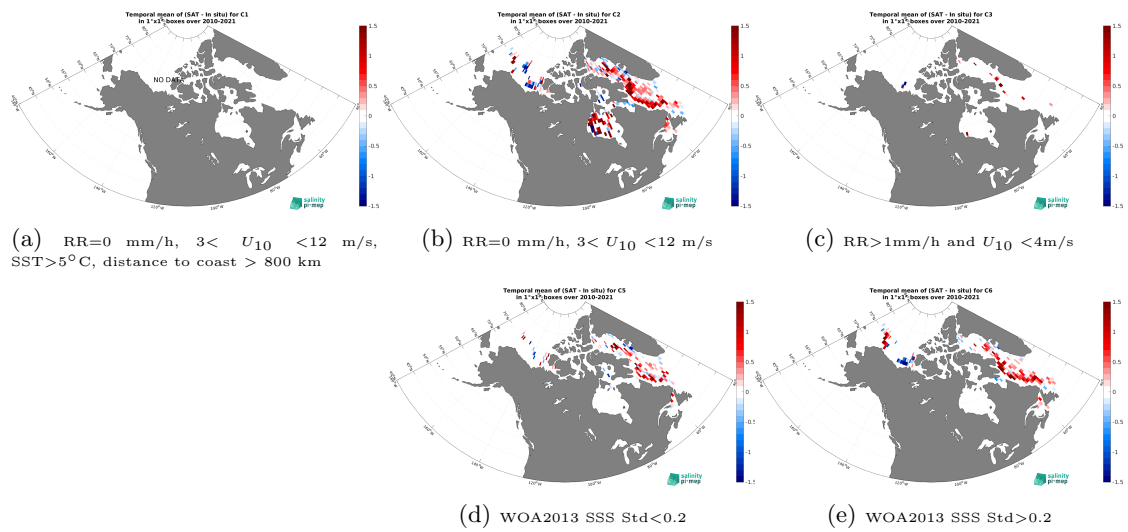
Figure 14: Temporal mean gridded over spatial boxes of size 1^\circ \times 1^\circ of \Delta SSS (CCI SSS L4 Merged-OI v5.5 - 7-day running (ESA) - TSG (Amundsen)) for 5 different subdatasets corresponding to: RR=0 mm/h, 3 < U_{10} < 12 m/s, SST > 5°C, distance to coast > 800 km (a), RR=0 mm/h, 3 < U_{10} < 12 m/s (b), RR > 1mm/h and U_{10} < 4 m/s (c), WOA2013 SSS Std < 0.2 (d), WOA2013 SSS Std > 0.2 (e).
