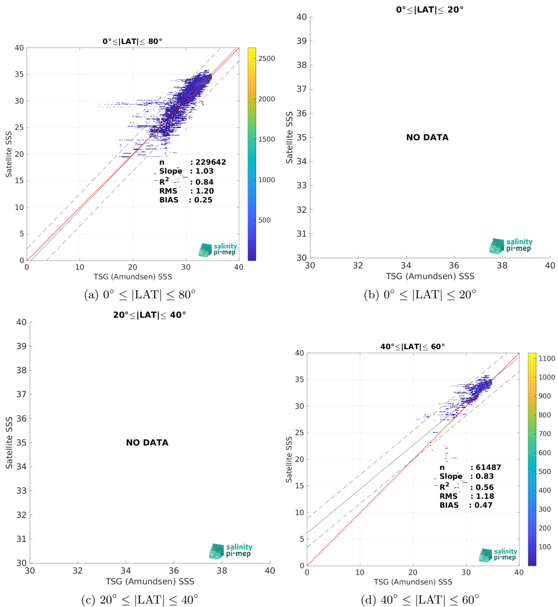
Figure 10: Contour maps of the concentration of CCI SSS L4 Merged-OI v5.5 - 7-day running (ESA) SSS (y-axis) versus TSG (Amundsen) SSS (x-axis) at match-up pairs for different latitude bands. For each plot, the red line shows x=y . The black thin and dashed lines indicate a linear fit through the data cloud and the \pm 95\% confidence levels, respectively. The number match-up pairs n , the slope and R^2 coefficient of the linear fit, the root mean square (RMS) and the mean bias between satellite and in situ data are indicated for each latitude band in each plot.
