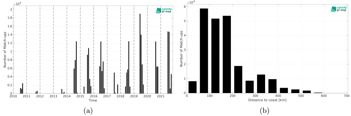
Figure 2: Number of match-ups between TSG (Amundsen) and CCI SSS L4 Merged-OI v5.5 - 7-day running (ESA) SSS as a function of time (a) and as function of the distance to coast (b) over the Global Ocean Pi-MEP region and for the full satellite product period.
