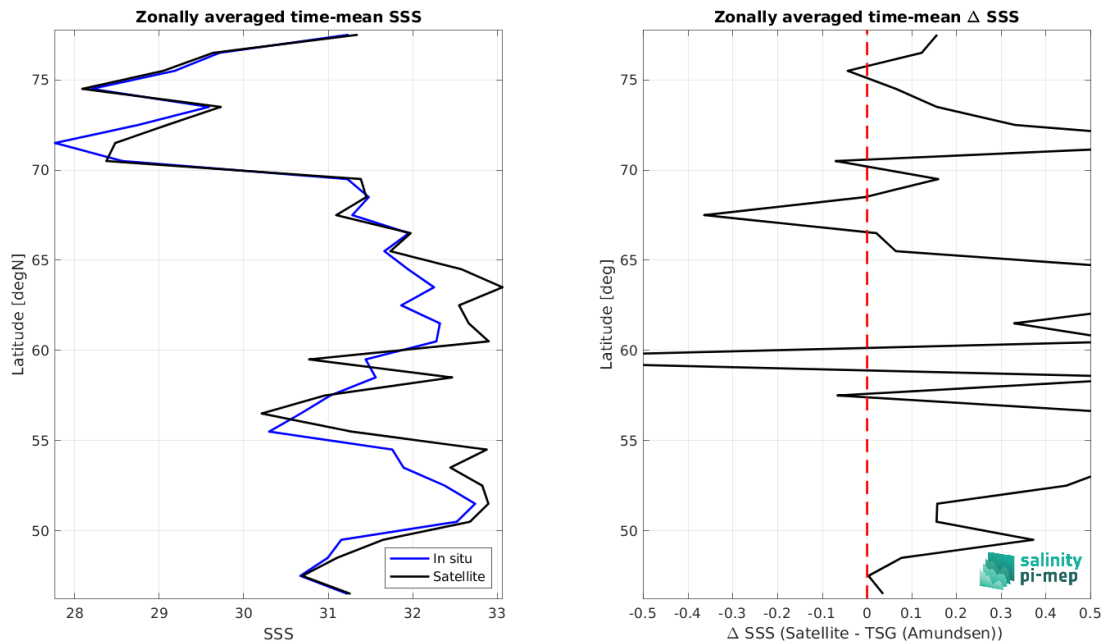
Figure 9: Left panel: Zonal mean SSS from CCI SSS L4 Merged-OI v5.5 - 7-day running (ESA) satellite product (black) and from TSG (Amundsen) (blue). Right panel: Zonal mean of \Delta SSS (Satellite - TSG (Amundsen)) for all the collected Pi-MEP match-up pairs estimated over the full satellite product period.
