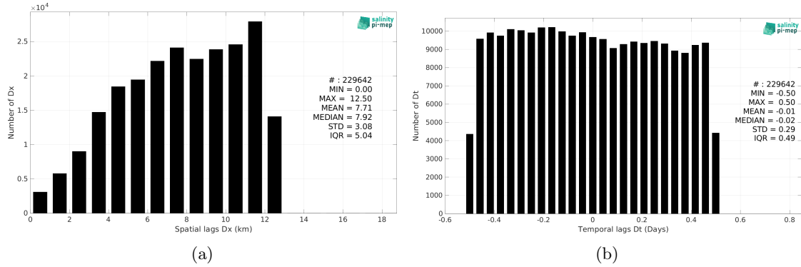
Figure 6: Histograms of the spatial (a) and temporal (b) lags between the location/time of the TSG (Amundsen) measurement and the date of the corresponding CCI SSS L4 Merged-OI v5.5 - 7-day running (ESA) SSS pixel.
