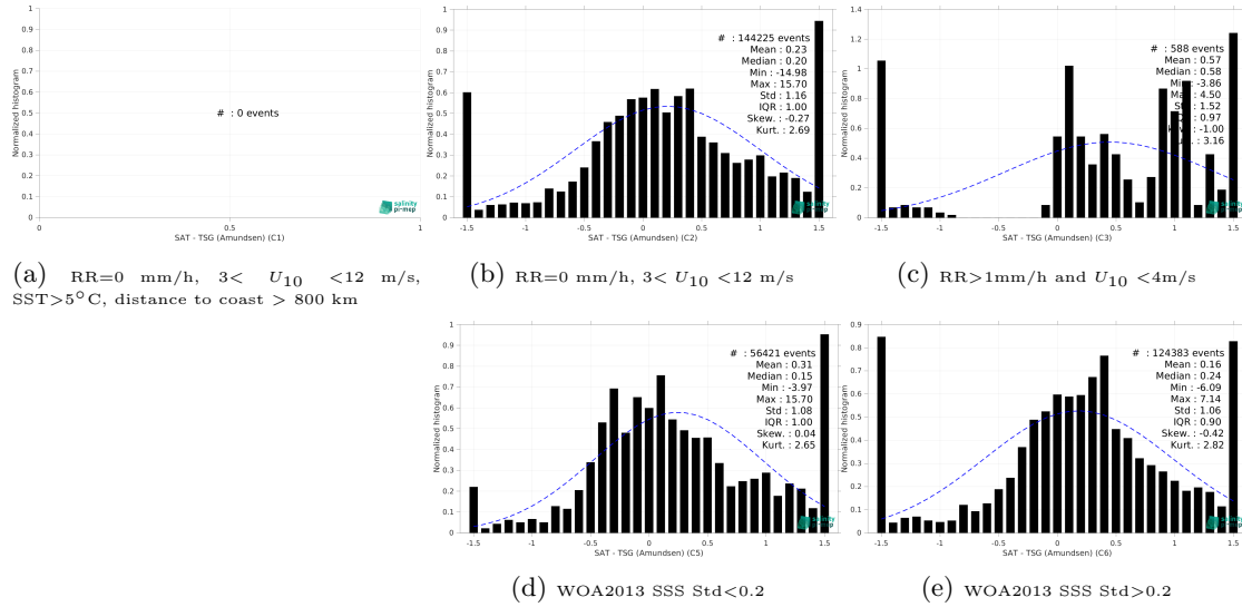
Figure 15: Normalized histogram of \Delta SSS (CCI SSS L4 Merged-OI v5.5 - 7-day running (ESA) - TSG (Amundsen)) for 5 different subdatasets corresponding to: RR=0 mm/h, 3 < U_{10} < 12 m/s, SST > 5°C, distance to coast > 800 km (a), RR=0 mm/h, 3 < U_{10} < 12 m/s (b), RR > 1mm/h and U_{10} < 4 m/s (c), WOA2013 SSS Std < 0.2 (d), WOA2013 SSS Std > 0.2 (e).
