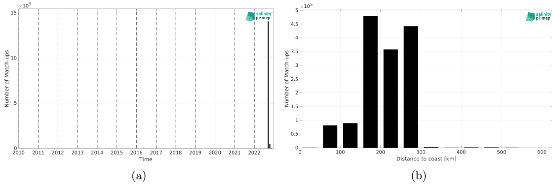
Figure 2: Number of match-ups between SASSIE and CCI SSS L4 Merged-OI v5.5 - 7-day running (ESA) SSS as a function of time (a) and as function of the distance to coast (b) over the Global Ocean Pi-MEP region and for the full satellite product period.
