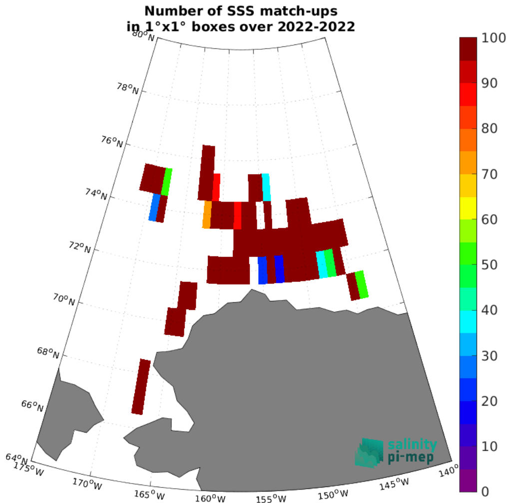
Figure 5: Number of SSS match-ups between SASSIE SSS and the CCI SSS L4 Merged-OI v5.5 - 7-day running (ESA) SSS product for the Global Ocean Pi-MEP region over 1^\circ \times 1^\circ boxes and for the full satellite product period.
