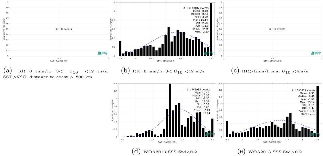
Figure 15: Normalized histogram of \Delta SSS (CCI SSS L4 Merged-OI v5.5 - 7-day running (ESA) - SASSIE) for 5 different subdatasets corresponding to: RR=0 mm/h, 3 < U_{10} < 12 m/s, SST > 5°C, distance to coast > 800 km (a), RR=0 mm/h, 3 < U_{10} < 12 m/s (b), RR > 1mm/h and U_{10} < 4 m/s (c), WOA2013 SSS Std < 0.2 (d), WOA2013 SSS Std > 0.2 (e).
