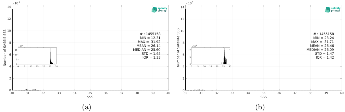
Figure 3: Histograms of SSS from SASSIE (a) and CCI SSS L4 Merged-OI v5.5 - 7-day running (ESA) (b) considering all match-up pairs per bins of 0.1 over the Global Ocean Pi-MEP region and for the full satellite product period.
