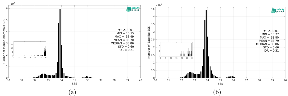
Figure 3: Histograms of SSS from Marine mammals (a) and CCI SSS L4 Merged-OI v5.5 - 7-day running (ESA) (b) considering all match-up pairs per bins of 0.1 over the Global Ocean Pi-MEP region and for the full satellite product period.
