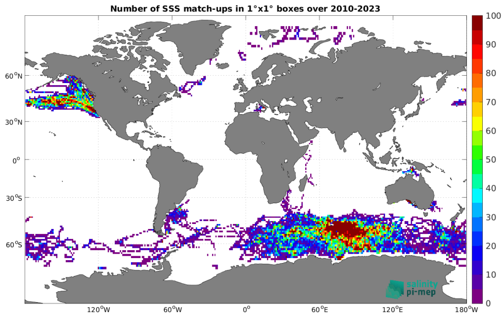
Figure 5: Number of SSS match-ups between Marine mammals SSS and the CCI SSS L4 Merged-OI v5.5 - 7-day running (ESA) SSS product for the Global Ocean Pi-MEP region over 1°x1° boxes and for the full satellite product period.
