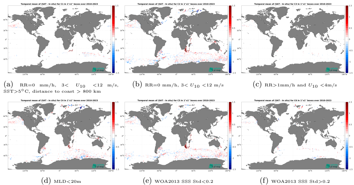
Figure 14: Temporal mean gridded over spatial boxes of size 1^\circ \times 1^\circ of \Delta SSS (CCI SSS L4 Merged-OI v5.5 - 7-day running (ESA) - Marine mammals) for 6 different subdatasets corresponding to:RR=0 mm/h, 3 < U_{10} < 12 m/s, SST >5^\circ C, distance to coast > 800 km (a), RR=0 mm/h, 3 < U_{10} < 12 m/s (b), RR >1 mm/h and U_{10} < 4 m/s (c),MLD <20 m (d),WOA2013 SSS Std <0.2 (e),WOA2013 SSS Std >0.2 (f).
