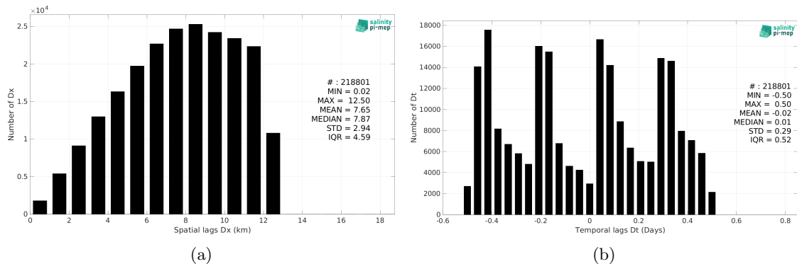
Figure 6: Histograms of the spatial (a) and temporal (b) lags between the location/time of the Marine mammals measurement and the date of the corresponding CCI SSS L4 Merged-OI v5.5 - 7-day running (ESA) SSS pixel.
