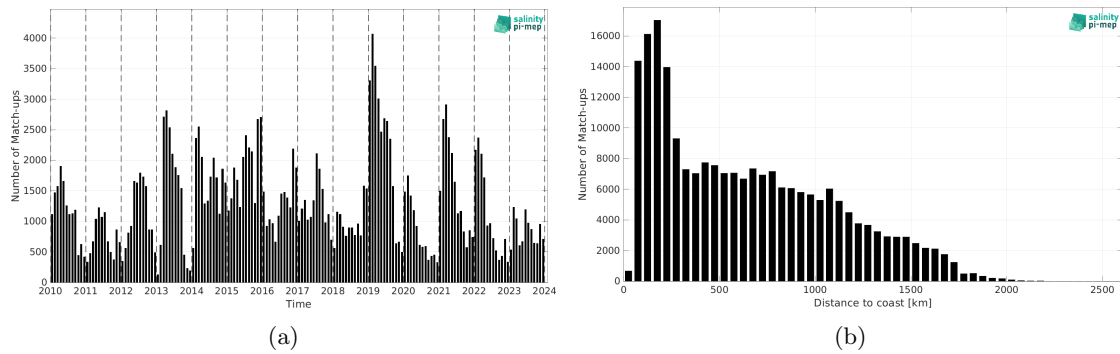
Figure 2: Number of match-ups between Marine mammals and CCI SSS L4 Merged-OI v5.5 - 7-day running (ESA) SSS as a function of time (a) and as function of the distance to coast (b) over the Global Ocean Pi-MEP region and for the full satellite product period.
