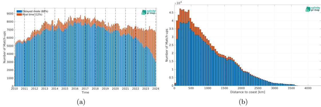
Figure 2: Number of match-ups between Argo and CCI SSS L4 Merged-OI v5.5 - 7-day running (ESA) SSS as a function of time (a) and as function of the distance to coast (b) over the Global Ocean Pi-MEP region and for the full satellite product period.
