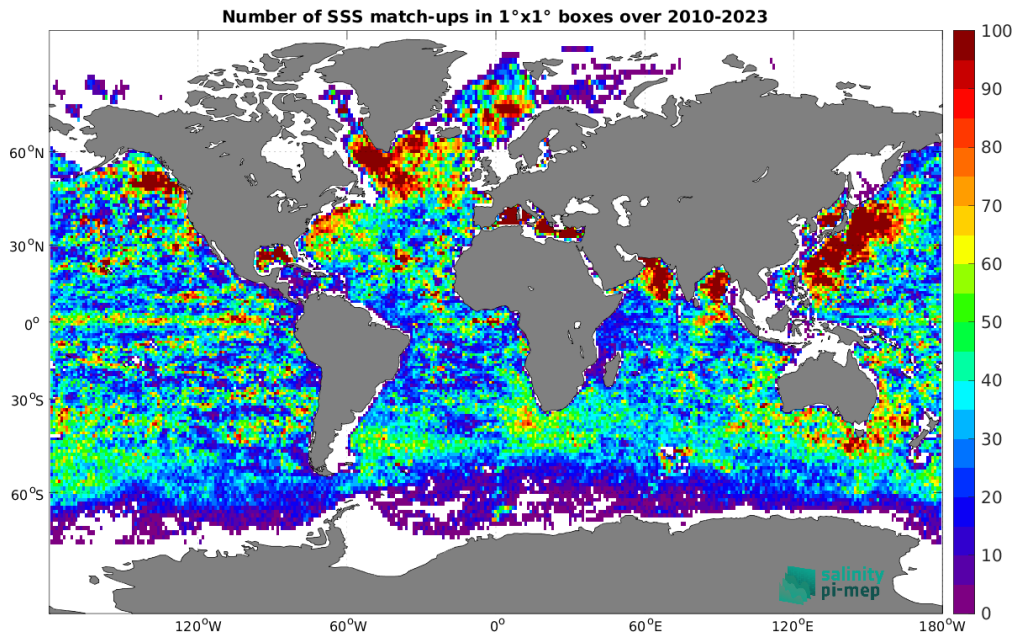
Figure 5: Number of SSS match-ups between Argo SSS and the CCI SSS L4 Merged-OI v5.5 - 7-day running (ESA) SSS product for the Global Ocean Pi-MEP region over 1^\circ \times 1^\circ boxes and for the full satellite product period.
