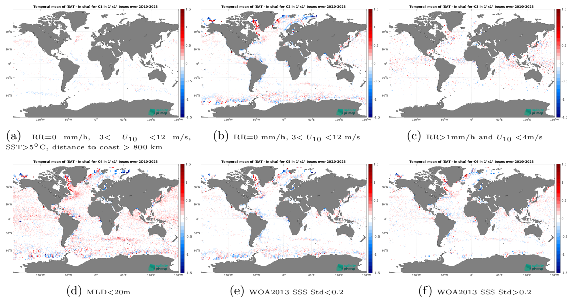
Figure 14: Temporal mean gridded over spatial boxes of size 1^\circ \times 1^\circ of \Delta SSS (CCI SSS L4 Merged-OI v5.5 - 7-day running (ESA) - Argo) for 6 different subdatasets corresponding to:RR=0 mm/h, 3 < U_{10} < 12 m/s, SST >5^\circ C, distance to coast > 800 km (a), RR=0 mm/h, 3 < U_{10} < 12 m/s (b), RR >1 mm/h and U_{10} < 4 m/s (c),MLD <20 m (d),WOA2013 SSS Std <0.2 (e),WOA2013 SSS Std >0.2 (f).
