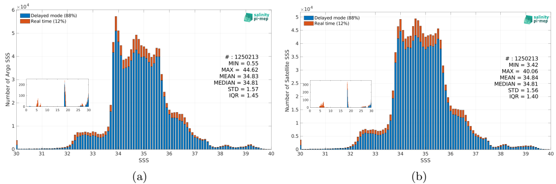
Figure 3: Histograms of SSS from Argo (a) and CCI SSS L4 Merged-OI v5.5 - 7-day running (ESA) (b) considering all match-up pairs per bins of 0.1 over the Global Ocean Pi-MEP region and for the full satellite product period.
