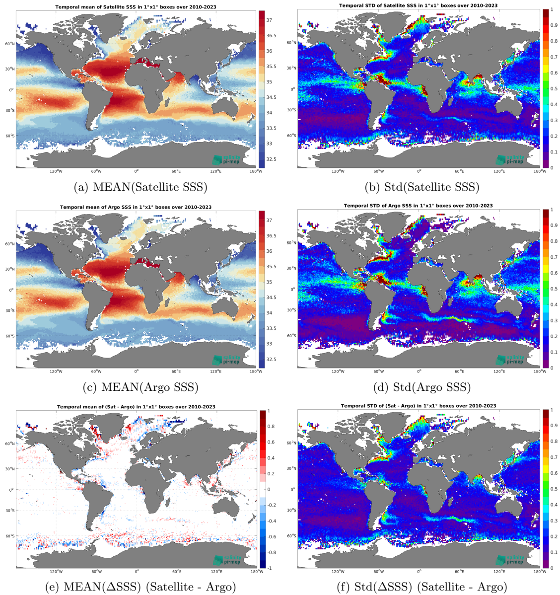
Figure 7: Temporal mean (left) and Std (right) of SSS from CCI SSS L4 Merged-OI v5.5 - 7-day running (ESA) (top), Argo (middle), and of \Delta SSS (Satellite - Argo). Only match-up pairs are used to generate these maps.
