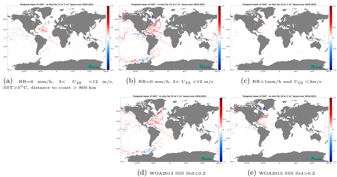
Figure 14: Temporal mean gridded over spatial boxes of size 1^\circ \times 1^\circ of \Delta\text{SSS} (CCI SSS L4 Merged-OI v5.5 - 30-day running (ESA) - TSG (SAMOS)) for 5 different subdatasets corresponding to:RR=0 mm/h, 3 < U_{10} < 12 m/s, SST > 5^\circ\text{C} , distance to coast > 800 km (a), RR=0 mm/h, 3 < U_{10} < 12 m/s (b), RR > 1 mm/h and U_{10} < 4 m/s (c), WOA2013 SSS Std < 0.2 (d), WOA2013 SSS Std > 0.2 (e).
