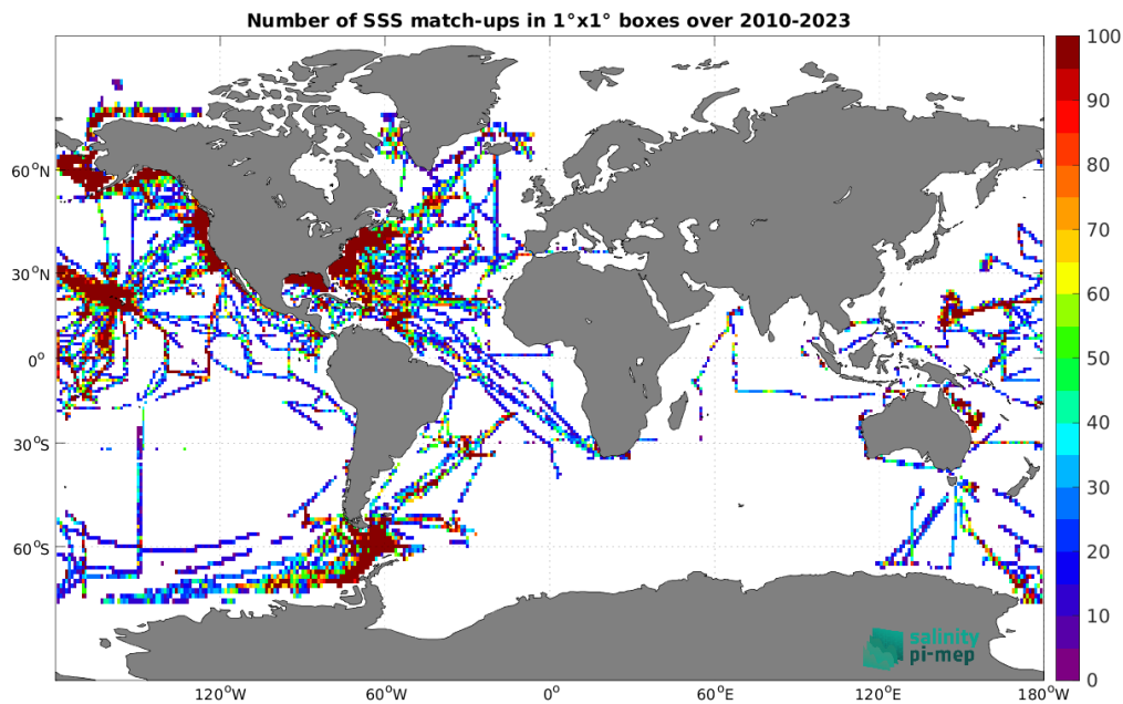
Figure 5: Number of SSS match-ups between TSG (SAMOS) SSS and the CCI SSS L4 Merged-OI v5.5 - 30-day running (ESA) SSS product for the Global Ocean Pi-MEP region over 1^\circ \times 1^\circ boxes and for the full satellite product period.
