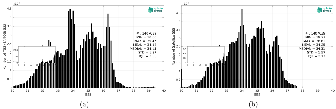
Figure 3: Histograms of SSS from TSG (SAMOS) (a) and CCI SSS L4 Merged-OI v5.5 - 30-day running (ESA) (b) considering all match-up pairs per bins of 0.1 over the Global Ocean Pi-MEP region and for the full satellite product period.
