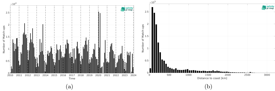
Figure 2: Number of match-ups between TSG (SAMOS) and CCI SSS L4 Merged-OI v5.5 - 30-day running (ESA) SSS as a function of time (a) and as function of the distance to coast (b) over the Global Ocean Pi-MEP region and for the full satellite product period.
