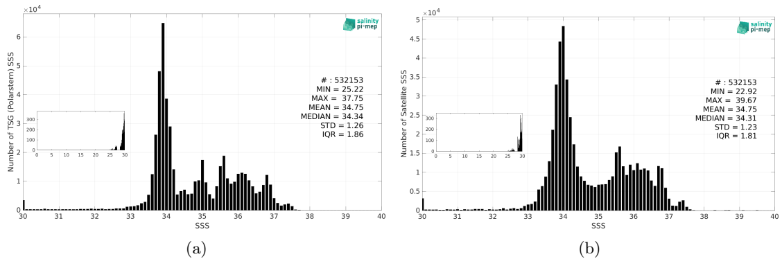
Figure 3: Histograms of SSS from TSG (Polarstern) (a) and CCI SSS L4 Merged-OI v5.5 - 30-day running (ESA) (b) considering all match-up pairs per bins of 0.1 over the Global Ocean Pi-MEP region and for the full satellite product period.
