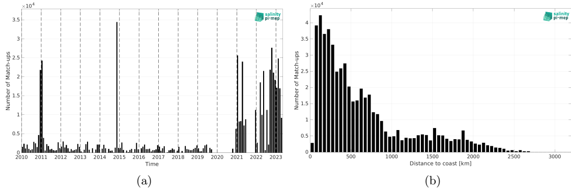
Figure 2: Number of match-ups between TSG (Polarstern) and CCI SSS L4 Merged-OI v5.5 - 30-day running (ESA) SSS as a function of time (a) and as function of the distance to coast (b) over the Global Ocean Pi-MEP region and for the full satellite product period.
