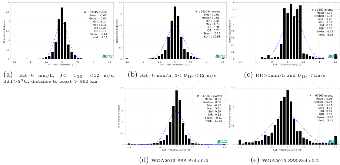
Figure 15: Normalized histogram of \Delta\text{SSS} (CCI SSS L4 Merged-OI v5.5 - 30-day running (ESA) - TSG (Polarstern)) for 5 different subdatasets corresponding to: RR=0 mm/h, 3 < U_{10} < 12 m/s, SST>5°C, distance to coast > 800 km (a), RR=0 mm/h, 3 < U_{10} < 12 m/s (b), RR>1mm/h and U_{10} < 4 m/s (c), WOA2013 SSS Std<0.2 (d), WOA2013 SSS Std>0.2 (e).
