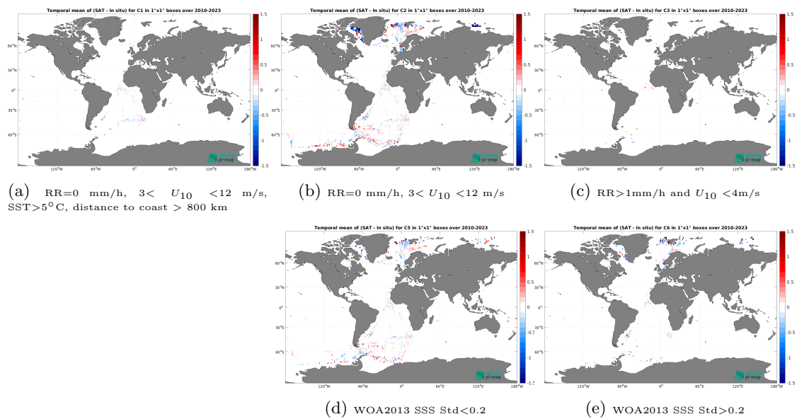
Figure 14: Temporal mean gridded over spatial boxes of size 1^\circ \times 1^\circ of \Delta SSS (CCI SSS L4 Merged-OI v5.5 - 30-day running (ESA) - TSG (Polarstern)) for 5 different subdatasets corresponding to: RR=0 mm/h, 3 < U_{10} < 12 m/s, SST > 5^\circ\text{C} , distance to coast > 800 km (a), RR=0 mm/h, 3 < U_{10} < 12 m/s (b), RR > 1\text{mm/h} and U_{10} < 4\text{m/s} (c), WOA2013 SSS Std < 0.2 (d), WOA2013 SSS Std > 0.2 (e).
