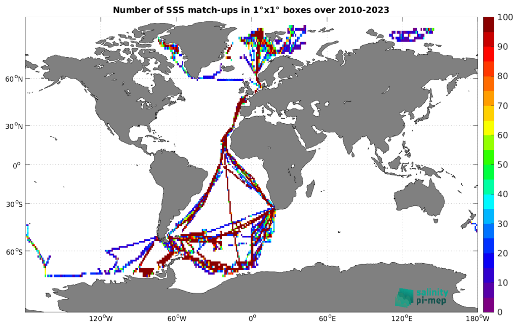
Figure 5: Number of SSS match-ups between TSG (Polarstern) SSS and the CCI SSS L4 Merged-OI v5.5 - 30-day running (ESA) SSS product for the Global Ocean Pi-MEP region over 1^\circ \times 1^\circ boxes and for the full satellite product period.
