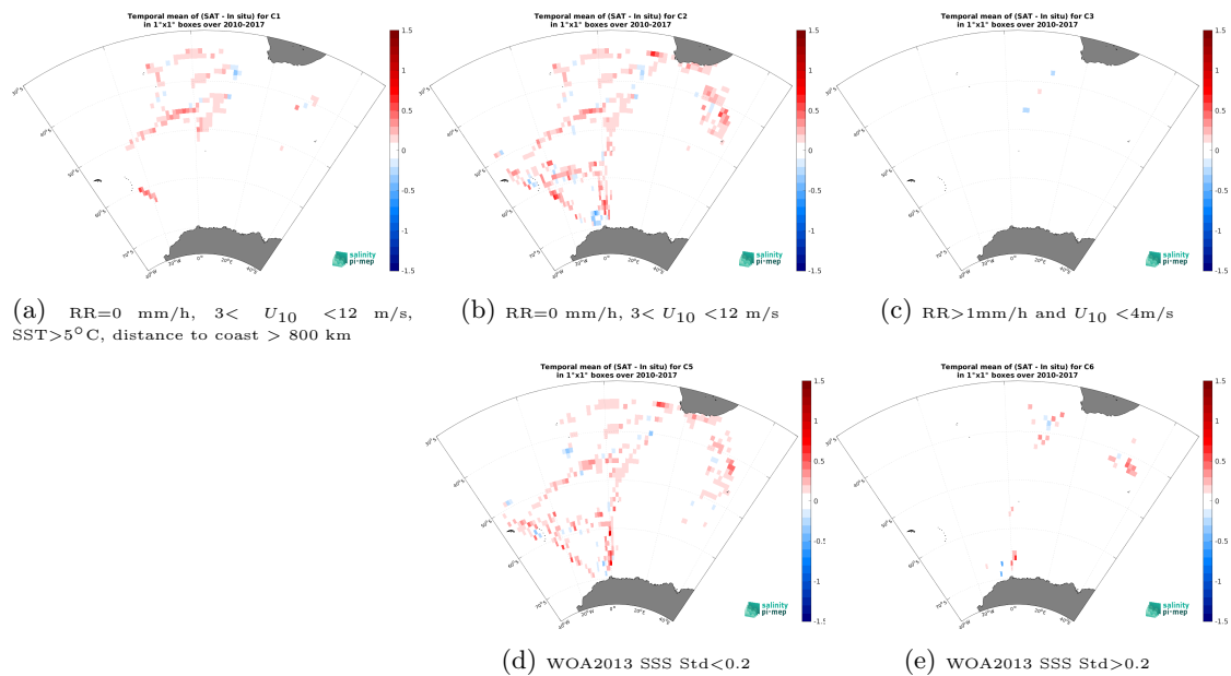
Figure 14: Temporal mean gridded over spatial boxes of size 1^\circ \times 1^\circ of \Delta\text{SSS} (CCI SSS L4 Merged-OI v5.5 - 30-day running (ESA) - TSG (NCEI-0170743)) for 5 different subdatasets corresponding to:RR=0 mm/h, 3 < U_{10} < 12 m/s, SST >5^\circ\text{C} , distance to coast > 800 km (a), RR=0 mm/h, 3 < U_{10} < 12 m/s (b), RR >1 mm/h and U_{10} < 4 m/s (c), WOA2013 SSS Std <0.2 (d), WOA2013 SSS Std >0.2 (e).
