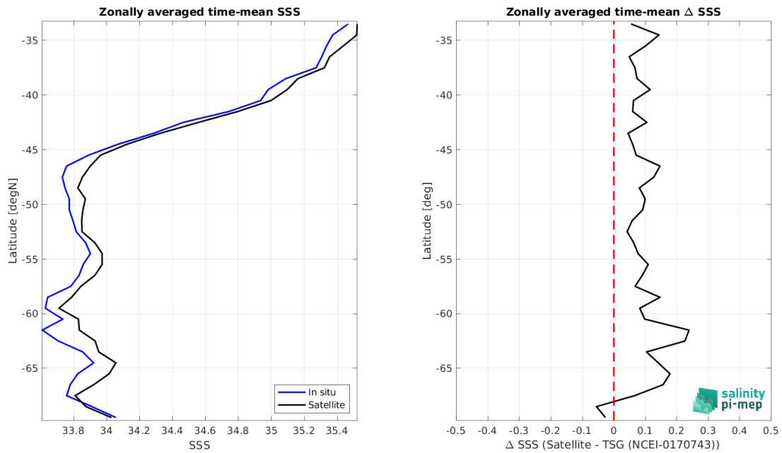
Figure 9: Left panel: Zonal mean SSS from CCI SSS L4 Merged-OI v5.5 - 30-day running (ESA) satellite product (black) and from TSG (NCEI-0170743) (blue). Right panel: Zonal mean of \Delta SSS (Satellite - TSG (NCEI-0170743)) for all the collected Pi-MEP match-up pairs estimated over the full satellite product period.
