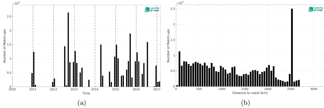
Figure 2: Number of match-ups between TSG (NCEI-0170743) and CCI SSS L4 Merged-OI v5.5 - 30-day running (ESA) SSS as a function of time (a) and as function of the distance to coast (b) over the Global Ocean Pi-MEP region and for the full satellite product period.
