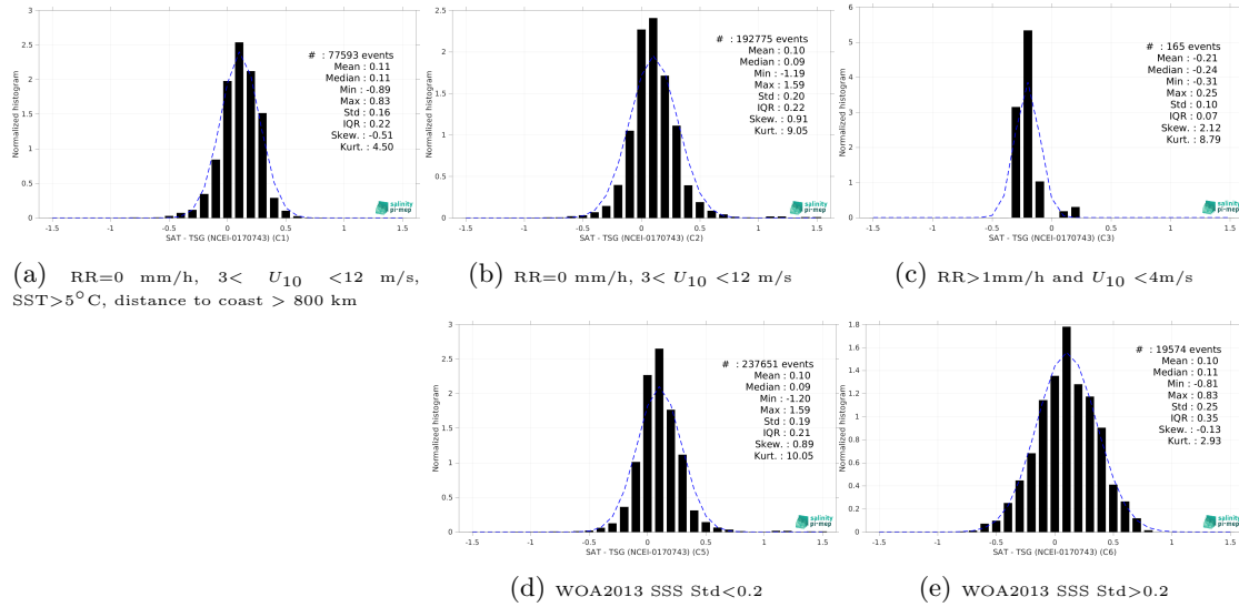
Figure 15: Normalized histogram of \Delta\text{SSS} (CCI SSS L4 Merged-OI v5.5 - 30-day running (ESA) - TSG (NCEI-0170743)) for 5 different subdatasets corresponding to: RR=0 mm/h, 3 < U_{10} < 12 m/s, SST>5°C, distance to coast > 800 km (a), RR=0 mm/h, 3 < U_{10} < 12 m/s (b), RR>1mm/h and U_{10} < 4 m/s (c), WOA2013 SSS Std<0.2 (d), WOA2013 SSS Std>0.2 (e).
