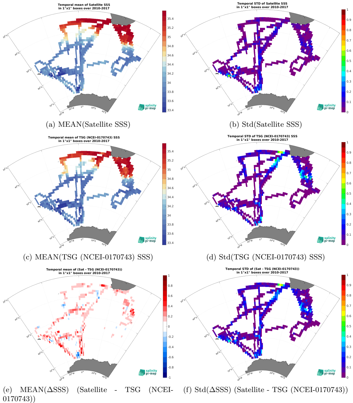
Figure 7: Temporal mean (left) and Std (right) of SSS from CCI SSS L4 Merged-OI v5.5 - 30-day running (ESA) (top), TSG (NCEI-0170743) (middle), and of \Delta SSS (Satellite - TSG (NCEI-0170743)). Only match-up pairs are used to generate these maps.
