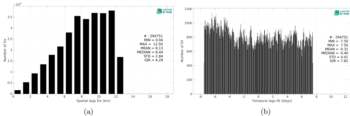
Figure 6: Histograms of the spatial (a) and temporal (b) lags between the location/time of the TSG (NCEI-0170743) measurement and the date of the corresponding CCI SSS L4 Merged-OI v5.5 - 30-day running (ESA) SSS pixel.
