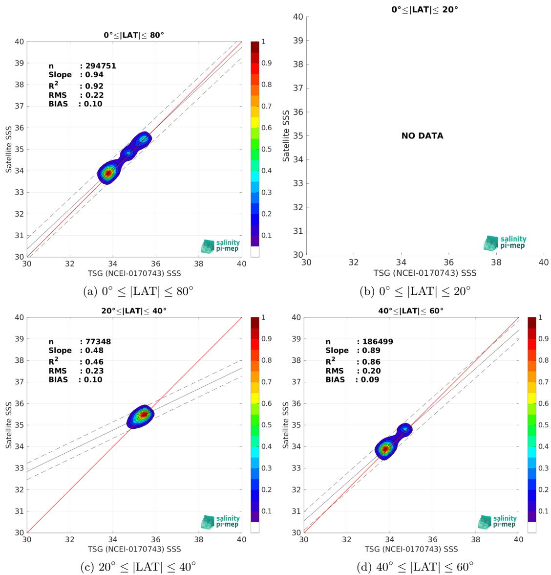
Figure 10: Contour maps of the concentration of CCI SSS L4 Merged-OI v5.5 - 30-day running (ESA) SSS (y-axis) versus TSG (NCEI-0170743) SSS (x-axis) at match-up pairs for different latitude bands. For each plot, the red line shows x=y . The black thin and dashed lines indicate a linear fit through the data cloud and the \pm 95\% confidence levels, respectively. The number match-up pairs n , the slope and R^2 coefficient of the linear fit, the root mean square (RMS) and the mean bias between satellite and in situ data are indicated for each latitude band in each plots.
