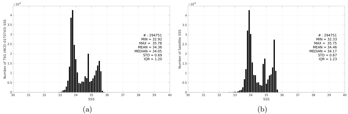
Figure 3: Histograms of SSS from TSG (NCEI-0170743) (a) and CCI SSS L4 Merged-OI v5.5 - 30-day running (ESA) (b) considering all match-up pairs per bins of 0.1 over the Global Ocean Pi-MEP region and for the full satellite product period.
