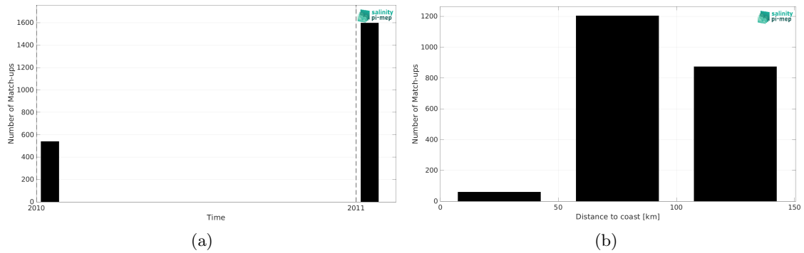
Figure 2: Number of match-ups between TSG (LEGOS-Surv-Adel) and CCI SSS L4 Merged-OI v5.5 - 30-day running (ESA) SSS as a function of time (a) and as function of the distance to coast (b) over the Global Ocean Pi-MEP region and for the full satellite product period.
