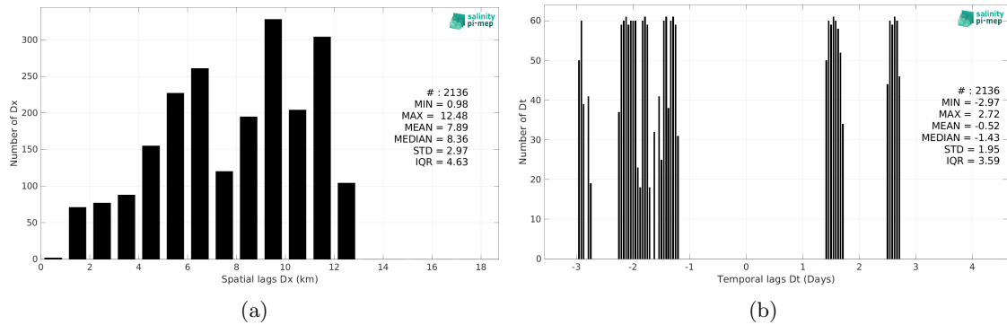
Figure 6: Histograms of the spatial (a) and temporal (b) lags between the location/time of the TSG (LEGOS-Surv-Adel) measurement and the date of the corresponding CCI SSS L4 Merged-OI v5.5 - 30-day running (ESA) SSS pixel.
