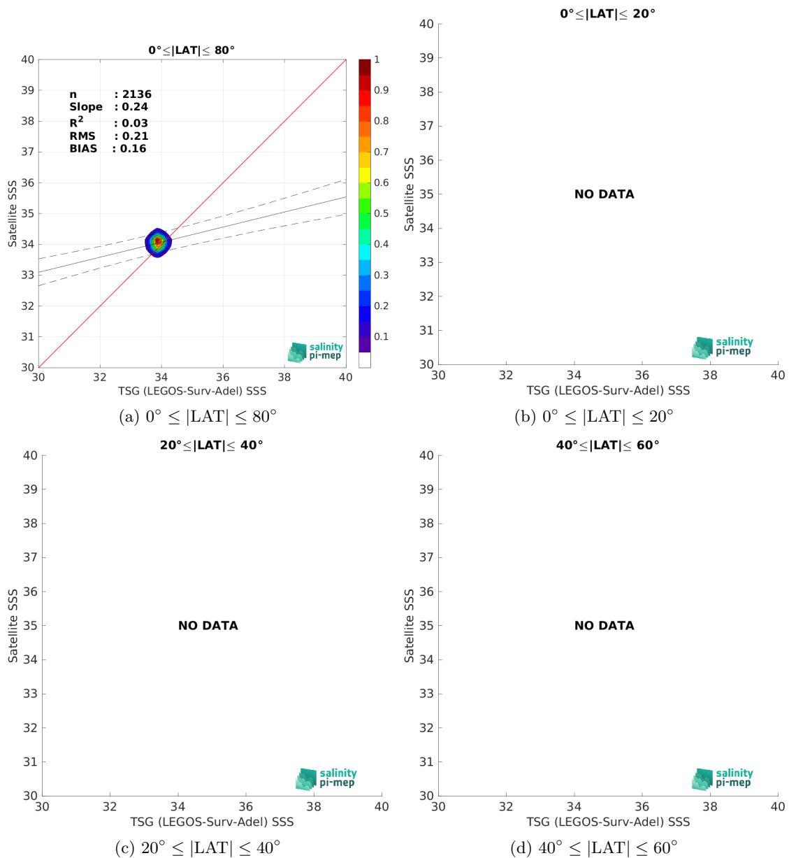
Figure 10: Contour maps of the concentration of CCI SSS L4 Merged-OI v5.5 - 30-day running (ESA) SSS (y-axis) versus TSG (LEGOS-Surv-Adel) SSS (x-axis) at match-up pairs for different latitude bands. For each plot, the red line shows x=y . The black thin and dashed lines indicate a linear fit through the data cloud and the \pm 95\% confidence levels, respectively. The number match-up pairs n , the slope and R^2 coefficient of the linear fit, the root mean square (RMS) and the mean bias between satellite and in situ data are indicated for each latitude band in each plots.
