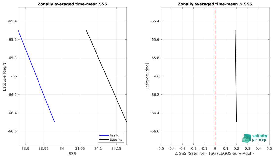
Figure 9: Left panel: Zonal mean SSS from CCI SSS L4 Merged-OI v5.5 - 30-day running (ESA) satellite product (black) and from TSG (LEGOS-Surv-Adel) (blue). Right panel: Zonal mean of \Delta SSS (Satellite - TSG (LEGOS-Surv-Adel)) for all the collected Pi-MEP match-up pairs estimated over the full satellite product period.
