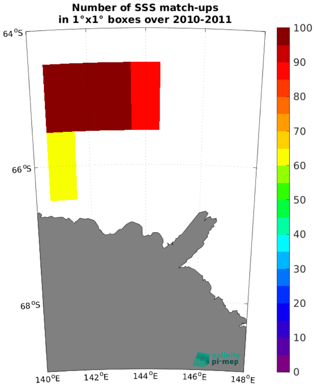
Figure 5: Number of SSS match-ups between TSG (LEGOS-Surv-Adel) SSS and the CCI SSS L4 Merged-OI v5.5 - 30-day running (ESA) SSS product for the Global Ocean Pi-MEP region over 1^\circ \times 1^\circ boxes and for the full satellite product period.
