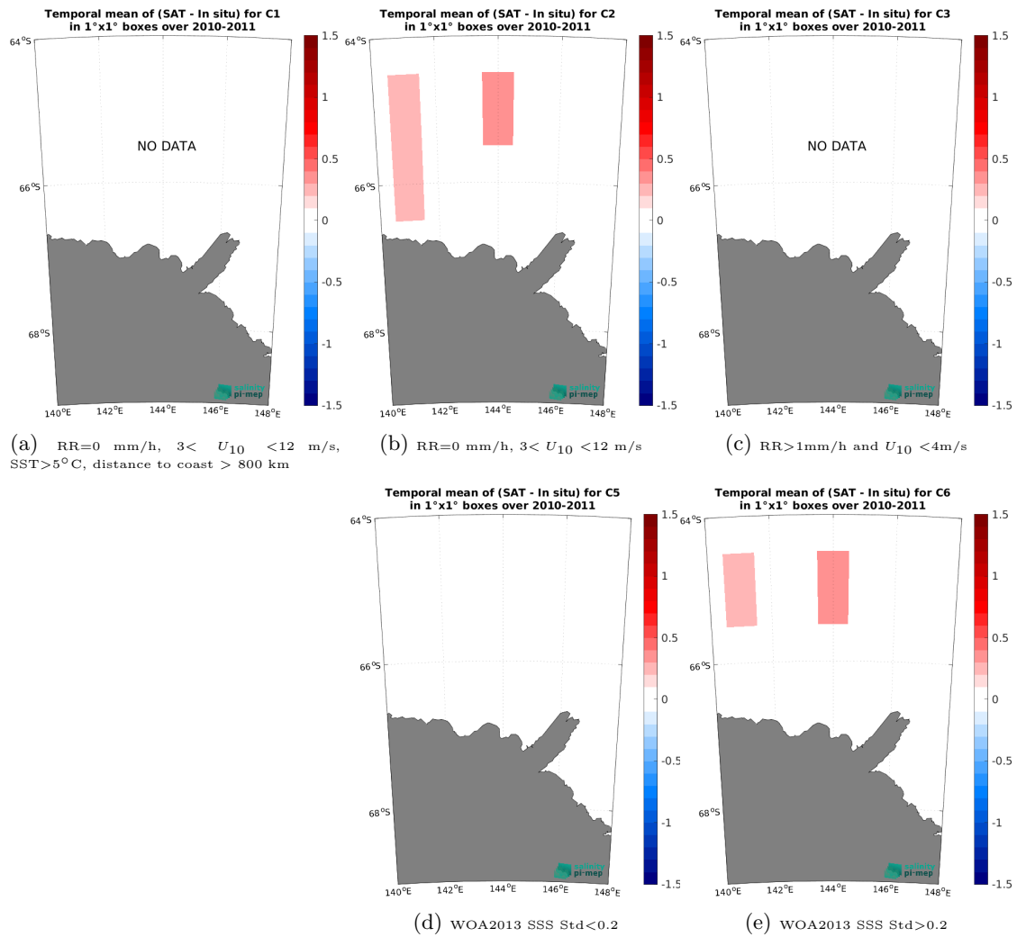
Figure 14: Temporal mean gridded over spatial boxes of size 1^\circ \times 1^\circ of \Delta SSS (CCI SSS L4 Merged-OI v5.5 - 30-day running (ESA) - TSG (LEGOS-Surv-Adel)) for 5 different subdatasets corresponding to: RR=0 mm/h, 3 < U_{10} < 12 m/s, SST>5°C, distance to coast > 800 km (a), RR=0 mm/h, 3 < U_{10} < 12 m/s (b), RR>1mm/h and U_{10} < 4 m/s (c), WOA2013 SSS Std<0.2 (d), WOA2013 SSS Std>0.2 (e).
