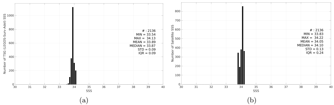
Figure 3: Histograms of SSS from TSG (LEGOS-Surv-Adel) (a) and CCI SSS L4 Merged-OI v5.5 - 30-day running (ESA) (b) considering all match-up pairs per bins of 0.1 over the Global Ocean Pi-MEP region and for the full satellite product period.
