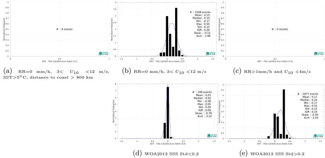
Figure 15: Normalized histogram of \Delta SSS (CCI SSS L4 Merged-OI v5.5 - 30-day running (ESA) - TSG (LEGOS-Surv-Adel)) for 5 different subdatasets corresponding to: RR=0 mm/h, 3 < U_{10} < 12 m/s, SST > 5°C, distance to coast > 800 km (a), RR=0 mm/h, 3 < U_{10} < 12 m/s (b), RR > 1mm/h and U_{10} < 4 m/s (c), WOA2013 SSS Std < 0.2 (d), WOA2013 SSS Std > 0.2 (e).
