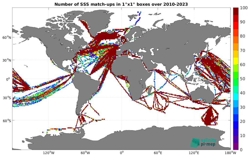
Figure 5: Number of SSS match-ups between TSG (LEGOS-DM) SSS and the CCI SSS L4 Merged-OI v5.5 - 30-day running (ESA) SSS product for the Global Ocean Pi-MEP region over 1^\circ \times 1^\circ boxes and for the full satellite product period.
