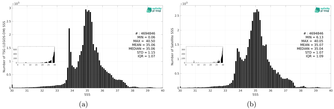
Figure 3: Histograms of SSS from TSG (LEGOS-DM) (a) and CCI SSS L4 Merged-OI v5.5 - 30-day running (ESA) (b) considering all match-up pairs per bins of 0.1 over the Global Ocean Pi-MEP region and for the full satellite product period.
