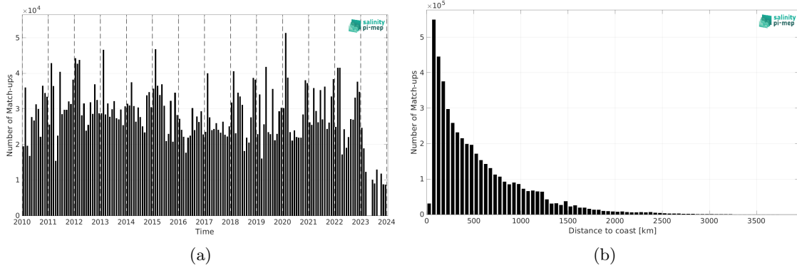
Figure 2: Number of match-ups between TSG (LEGOS-DM) and CCI SSS L4 Merged-OI v5.5 - 30-day running (ESA) SSS as a function of time (a) and as function of the distance to coast (b) over the Global Ocean Pi-MEP region and for the full satellite product period.
